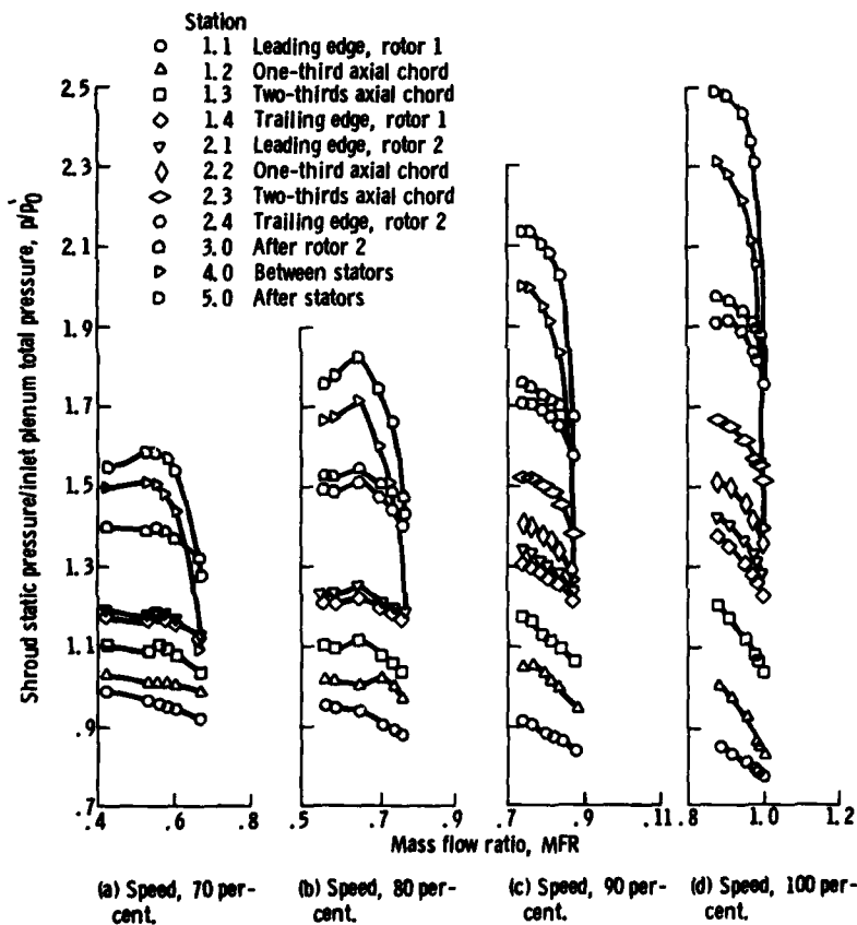
Figure 12. - Shroud static pressure ratio at various stations for medium clearance stage test.
