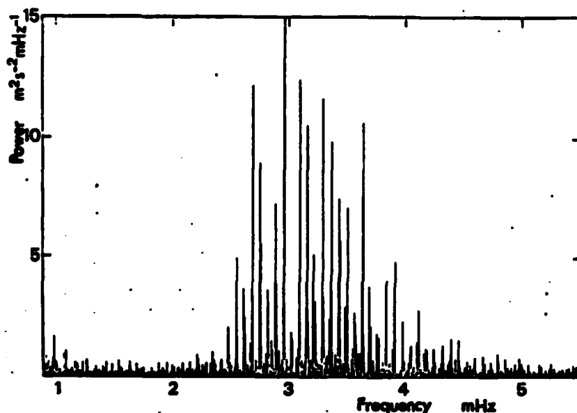
Figure 4. Power spectrum of the South Pole data. The sample analysed has a duration of about 6 days. The frequency resolution is 1.97 micro-Hz. (From Grec et al, 1982).
