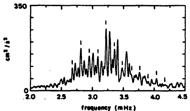
Figure 9. Average of 15 spectra from observations with an average duration of 9.6 hours. The vertical lines are the l=3 frequencies from Grec et al, 1982. (From Scherrer et al, 1982).
