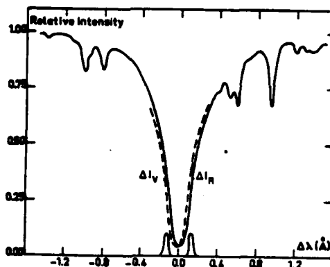
Figure 3. Principle of the resonant scattering devices. (From Grec et al, 1976).
