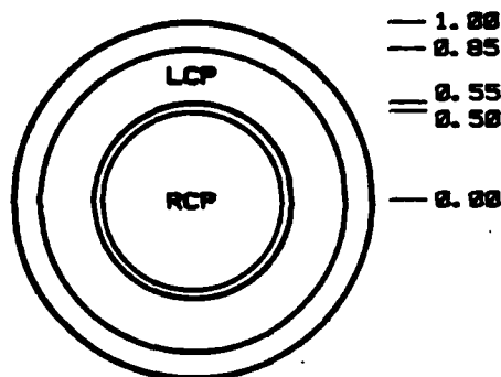
Figure 8. Polarizer configuration for Stanford modified magnetograph spectrometer.
