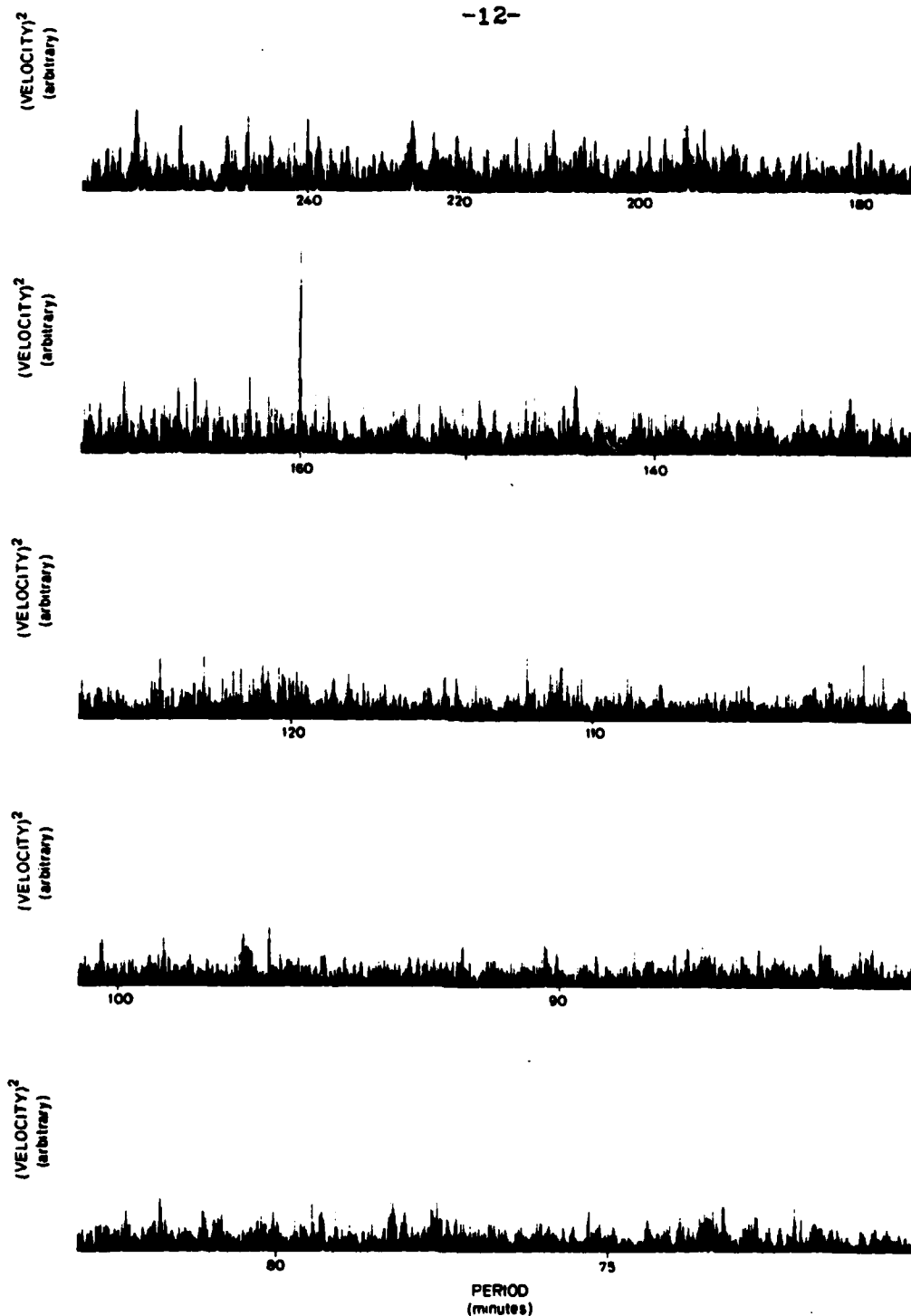
Figure 13. Combined Stanford and Crimean power spectrum. The spectrum includes periods from 1.2 hours to 4.6 hours, computed in steps of 2 nano-Hz. The peak near 160 minutes is seen to be unique in this range. (From Scherrer et al, 1982).
