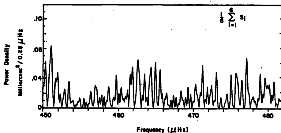
Figure 12. A portion of the power spectrum from the Santa Catalina Laboratory for Experimental Astrophysics. (SCLERA). (From Bos and Hill, 1982).
