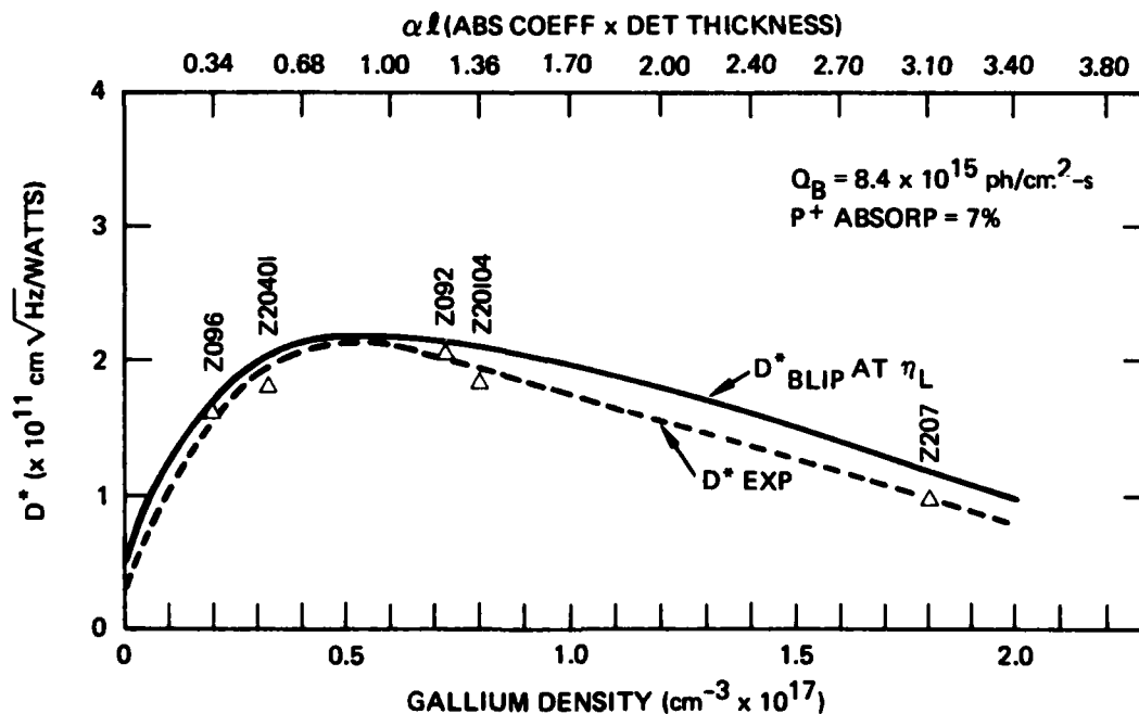
b. THEORETICAL AND EXPERIMENTAL D^* vs N_{\text{Ga}}
