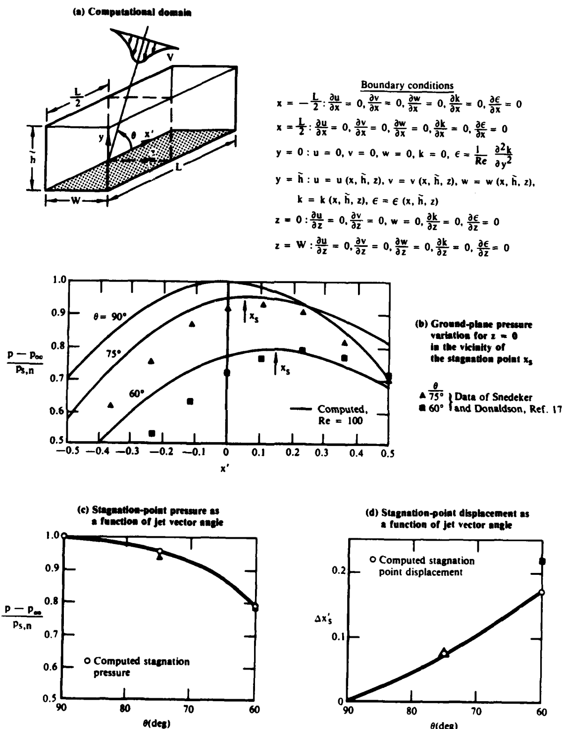
Figure 8. Flow properties for an isolated jet with inclined impingement.
