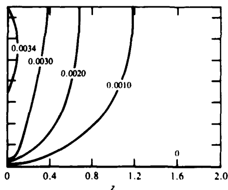
(f) Eddy viscosity for x = 0
