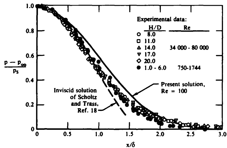
(b) Ground-plane pressure variation for z = 0
