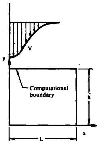
(a) Flow geometry
