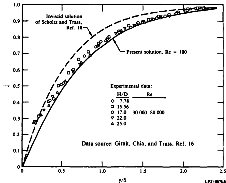
Figure 7. Flow properties for an isolated jet with normal impingement.
