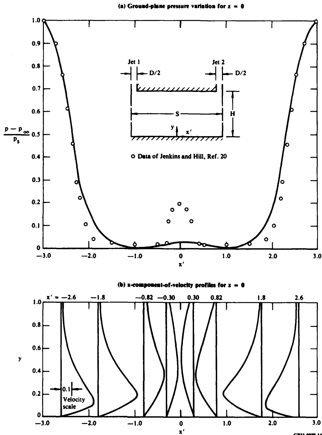
Figure 12. Flow properties for equal-strength jets with normal impingement ( S/D = 6 , H/D = 3 , Re = 200 ).
