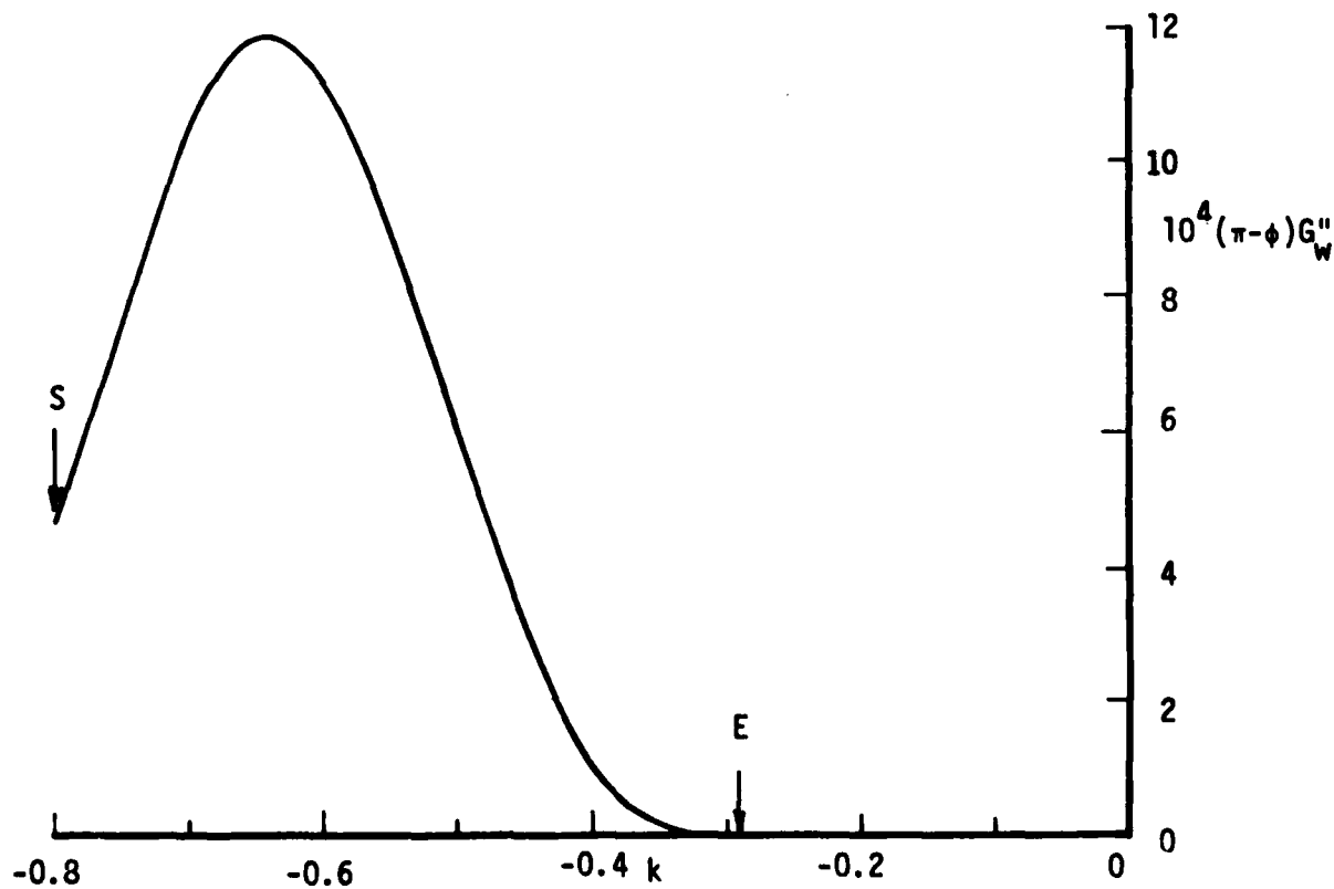
Fig. 2b. The values of 10^4 (\pi - \phi) G''_W as \phi \rightarrow \pi in the \phi -wise integration. S denotes the onset of separation of the crossflow for \phi < \pi and E denotes k = k^\dagger , where the similarity solution comes to an end.
