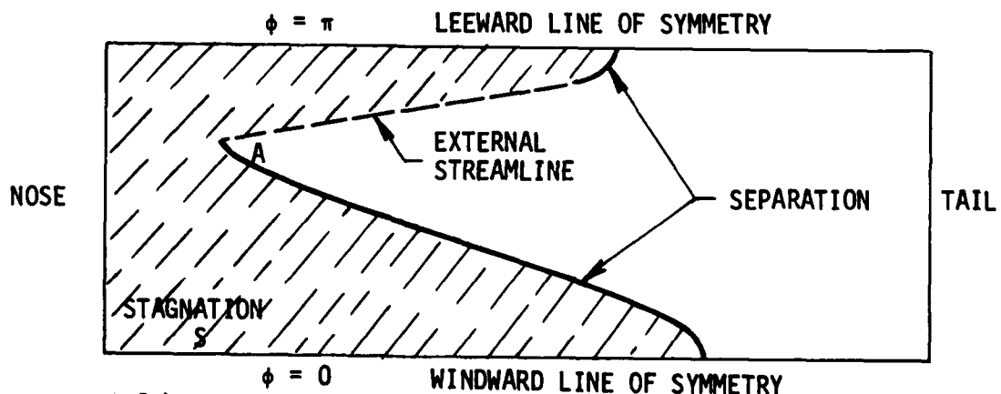
Fig. 1. The solution can be computed over the hatched part of the body starting from the forward stagnation point. Notice that the nose and tails are single points but in polar coordinates they must be replaced by lines ( 0 \leq \phi \leq \pi ).
