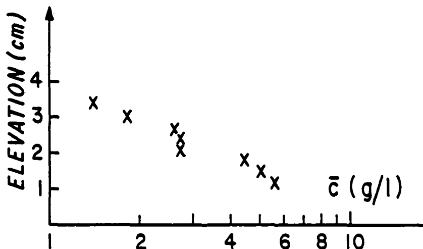
Figure 2.7: Time averaged suspended sediment concentrations \bar{C} from Nakato et. al. (1977), measured over natural ripples in an oscillating water tunnel. T = 1.8s , \alpha = .075m , d = .14mm .
