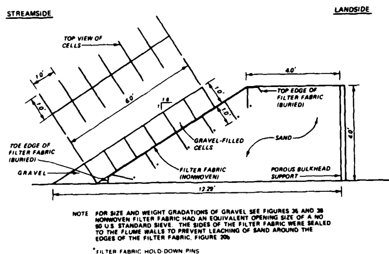
Figure 39. Plan 8C, sand streambank with gravel-filled cells and nonwoven filter fabric protection
