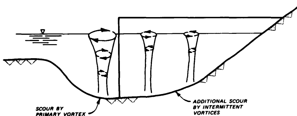
Figure 2. Scour hole profile along spur dike
