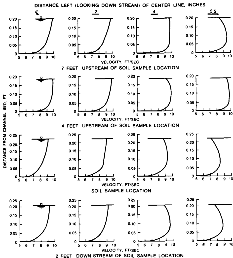
Figure C42. Calibration curves of velocity profiles at various locations and distances from the center line for zero bed slope, headgate opening of 3 in., and half headtank of water
