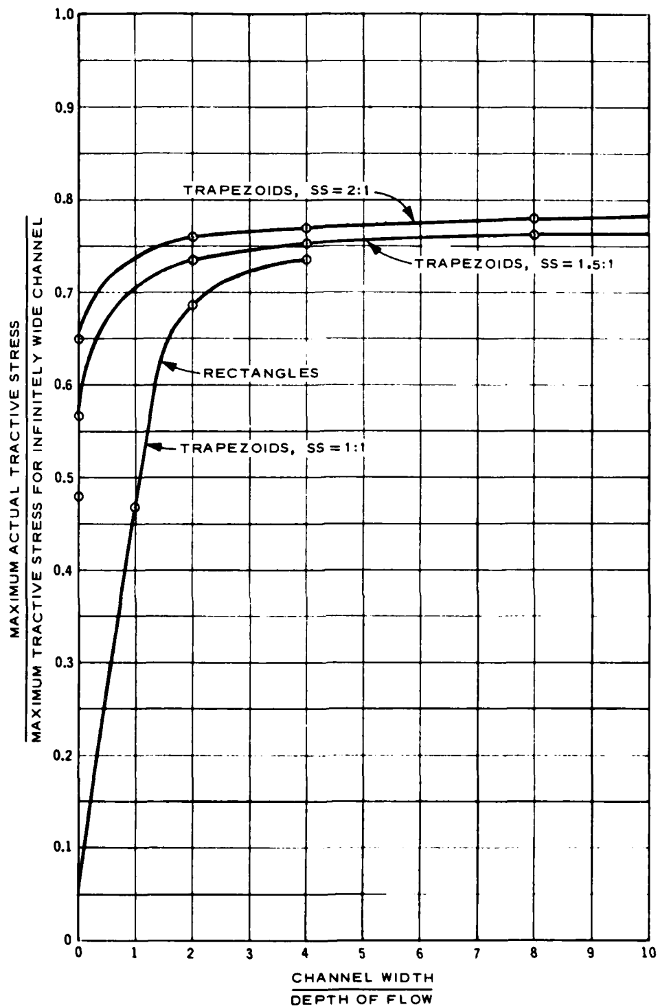
Figure C24. Ratio of actual maximum tractive shear stress on side of channel of finite width to maximum tractive shear stress on bed of infinitely wide channel (from Lane 1952)
