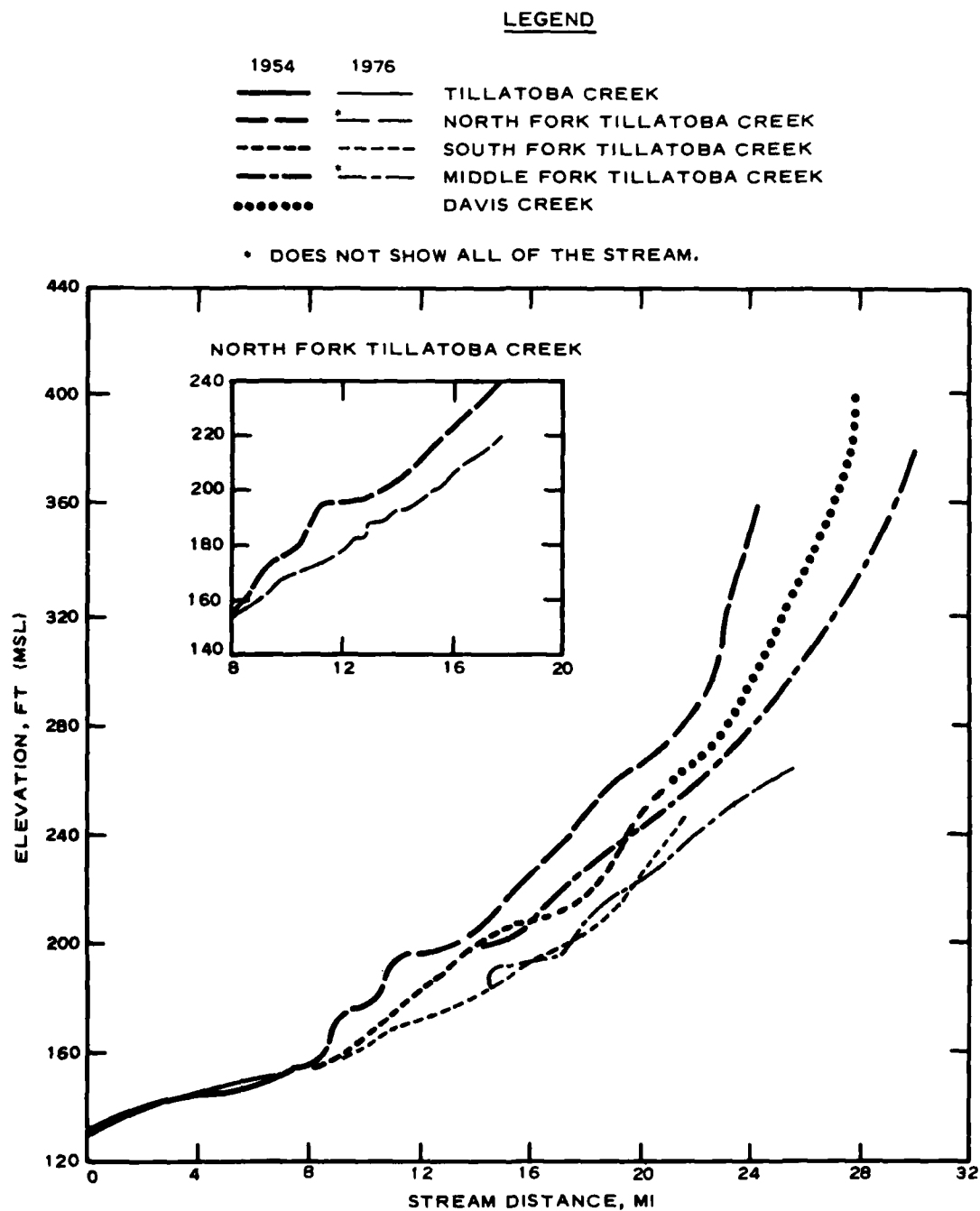
Figure C6. Changes in longitudinal profiles of Tillatoba Creek and principal tributaries (from Whitten and Patrick 1981)
