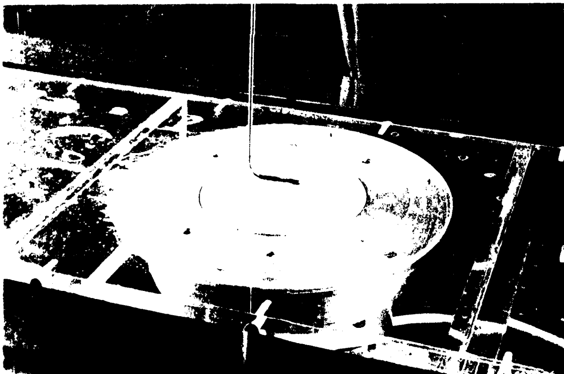
Figure C33. Soil sample mounted flush with bottom of flume and Pitot tube
