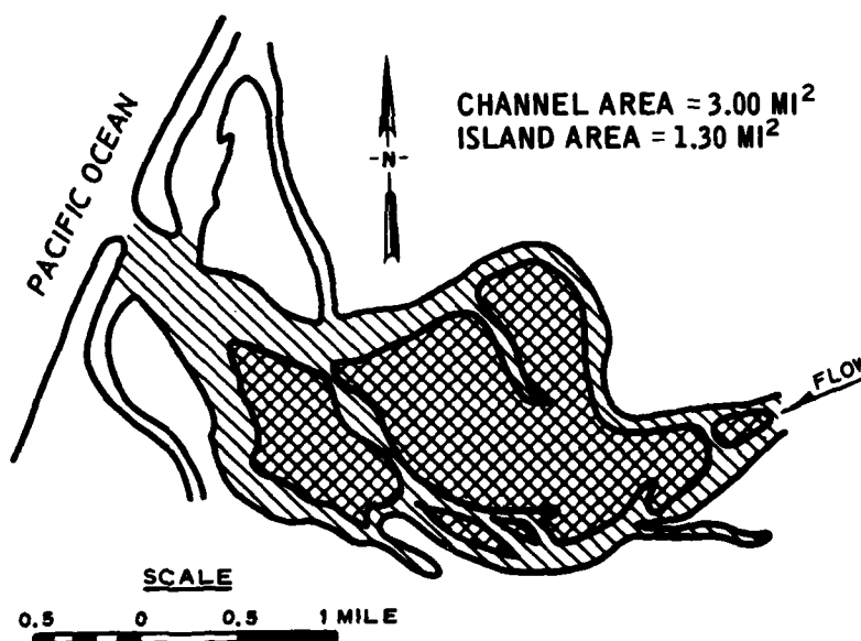
Figure C4. Changes in channel configuration in the Eel River Delta (from Smith and Patrick 1979)
