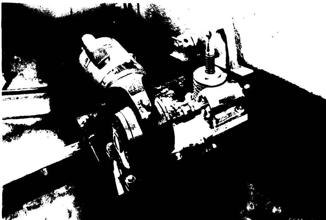
Figure C31. Electrically operated synchronized jack screws to tilt the flume
