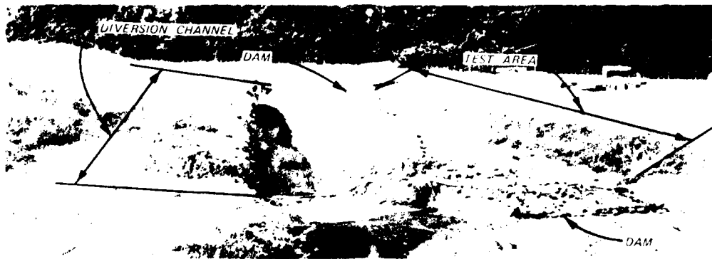
Photo C4. Diversion canal
