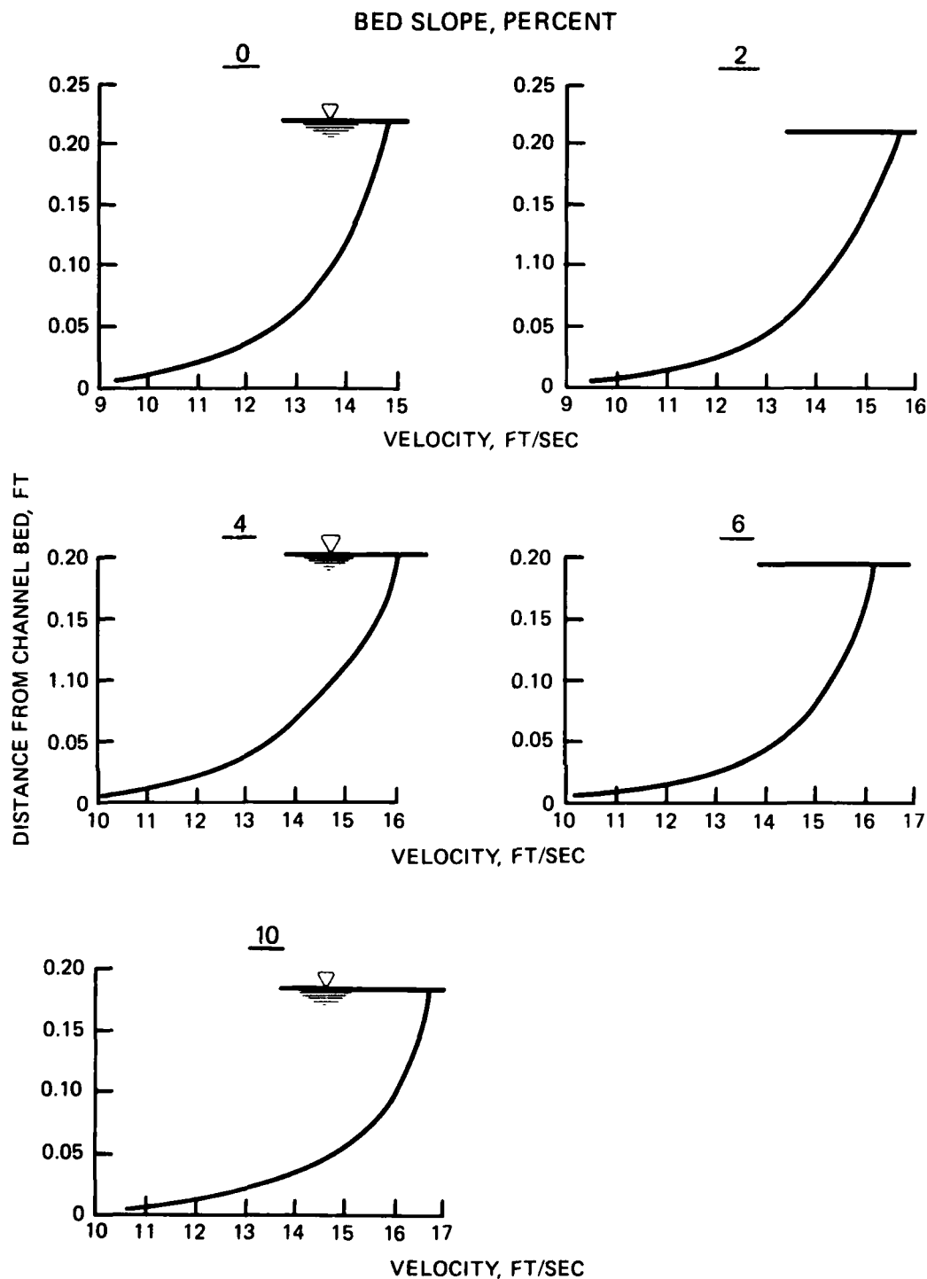
Figure C41. Calibration curves of velocity profiles at location of soil sample on center line for headgate opening of 3 in. and full headtank plus 12 in. of water in standpipe
