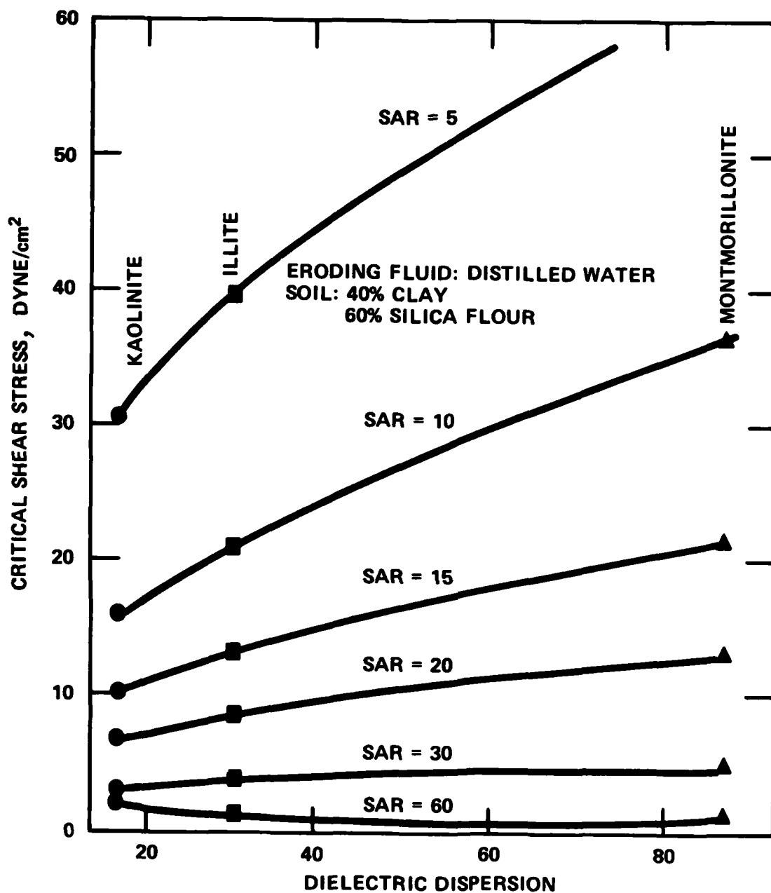
Figure C51. Relationship between critical tractive shear stress, sodium adsorption ratio, and dielectric dispersion for saturated remolded soil with distilled water as eroding fluid and soil pore fluid concentration of 125 milliequivalents/liter (from Alizadeh 1974 and Heinzen 1976)
