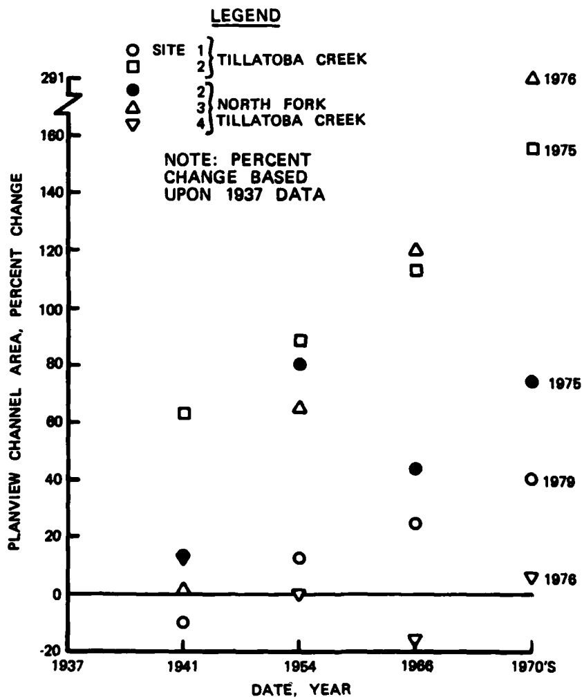
Figure C8. Changes in channel area and length of Tillatoba Creek and North Fork (from Whitten and Patrick 1981)
