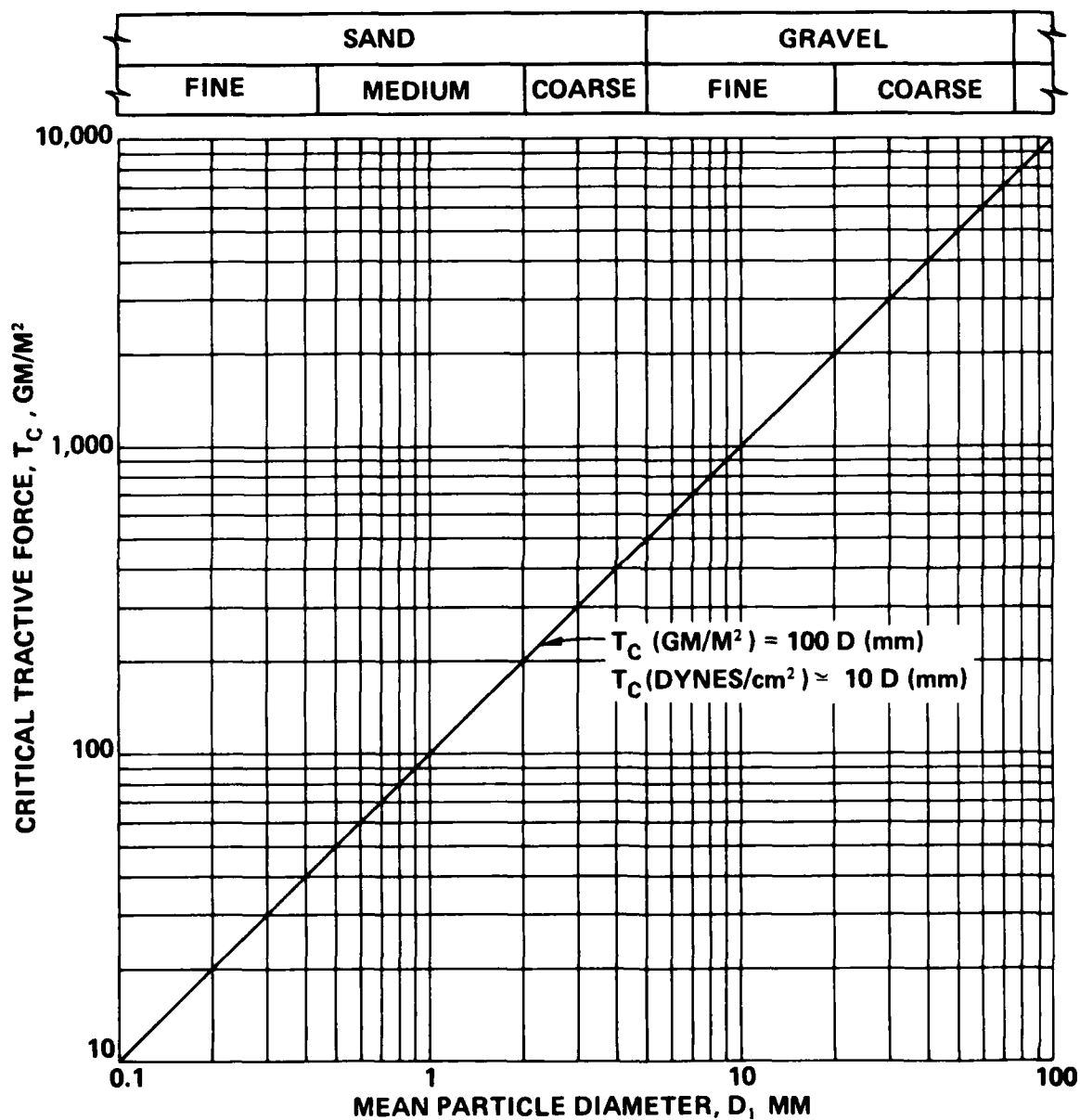
Figure C44. Relationship between critical tractive shear stress and mean particle diameter for sand and gravel (from Lane 1952)
