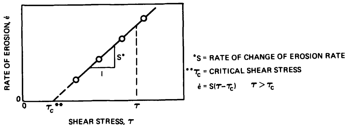
Figure C43. Definition of critical tractive shear stress, rate of change of erosion rate, and rate of erosion
