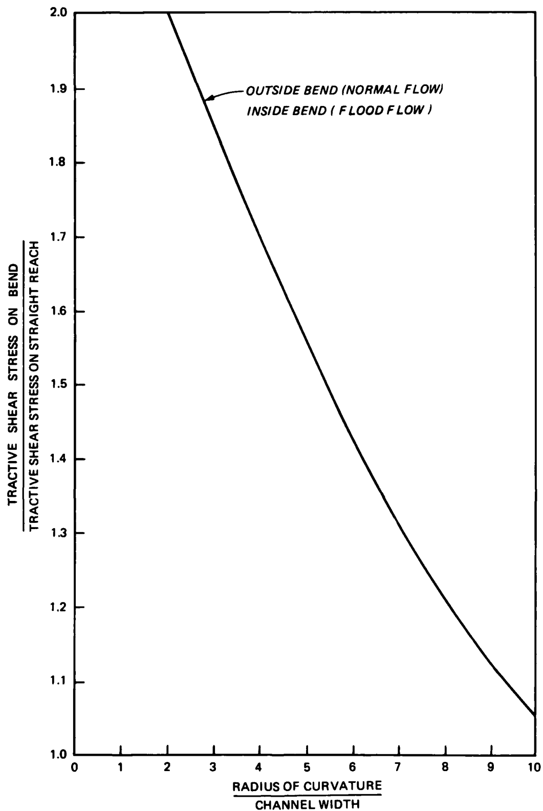
Figure C26. Ratio of tractive shear stress on bend to tractive shear stress on straight reach (from Soil Conservation Service 1977)
