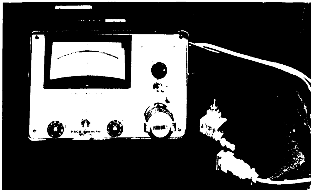
Figure C37. Variable reluctance differential pressure transducer and indicator used in calibrating the flume
