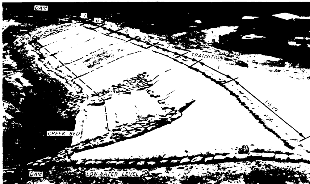
Photo C5. View (looking downstream) of test materials installed prior to removal of dams at each end of test area
