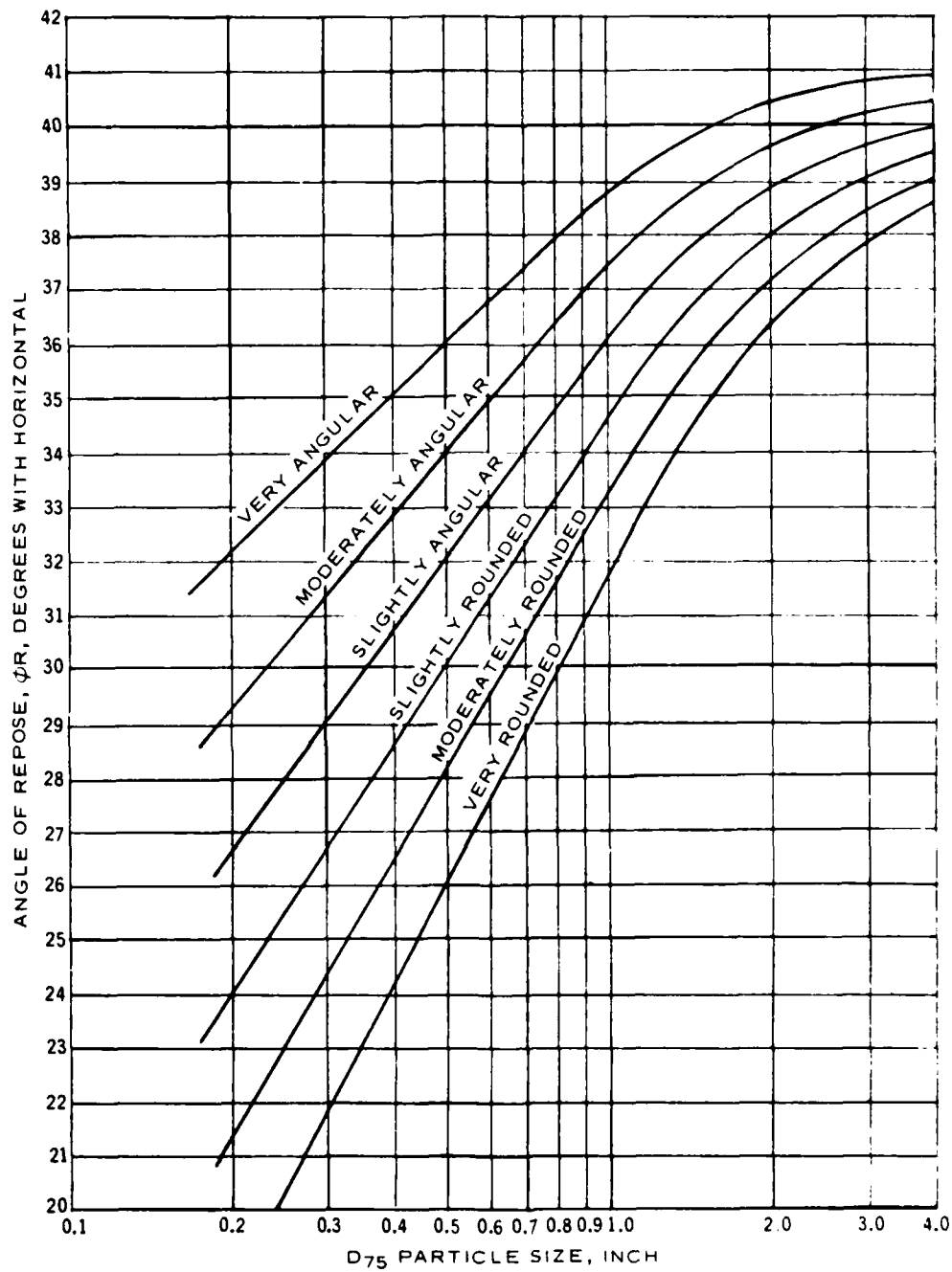
Figure C45. Relationship between angle of repose and D_{75} particle size for cohesionless soil (from Lane 1952)
