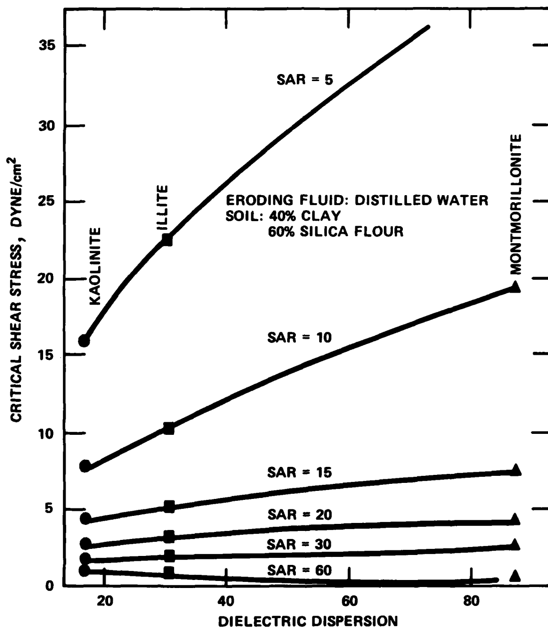
Figure C50. Relationship between critical tractive shear stress, sodium adsorption ratio, and dielectric dispersion for saturated remolded soil with distilled water as eroding fluid and soil pore fluid concentration of 50 milliequivalents/liter (from Alizadeh 1974 and Heinzen 1976)
