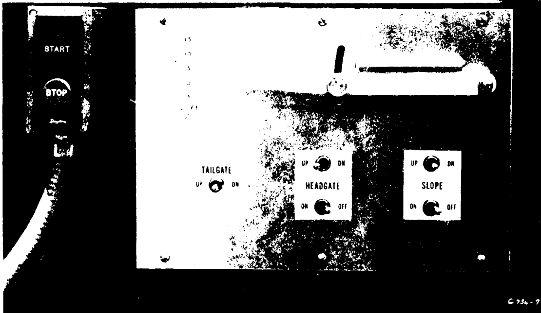
Figure C32. Control box for headgate, tailgate, and slope
