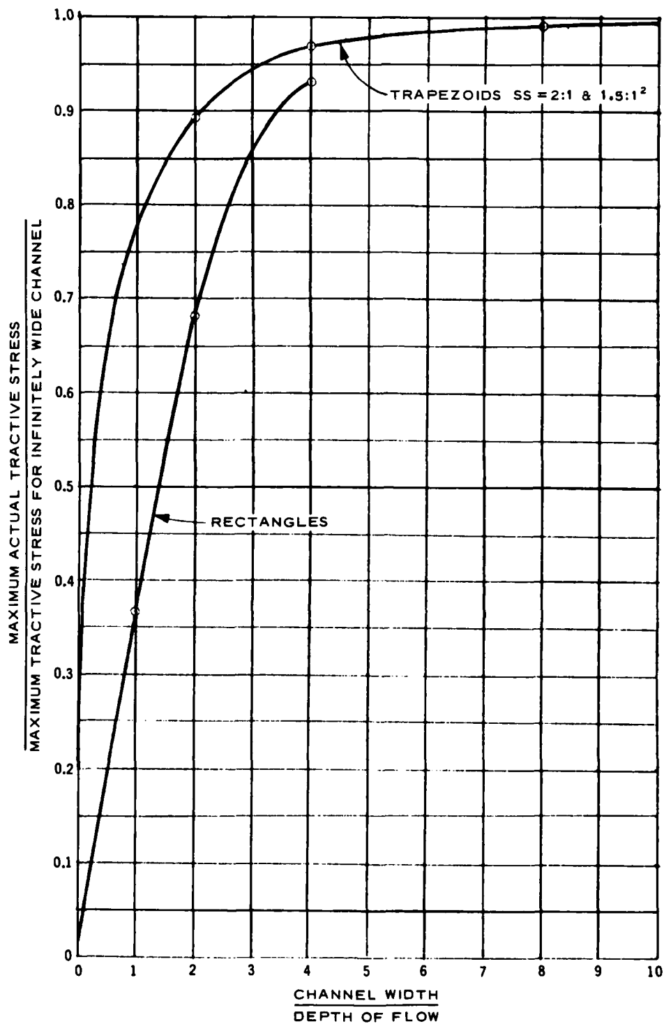
Figure C23. Ratio of actual maximum tractive shear stress on bed of channel of finite width to maximum tractive shear stress on bed of infinitely wide channel (from Lane 1952)
