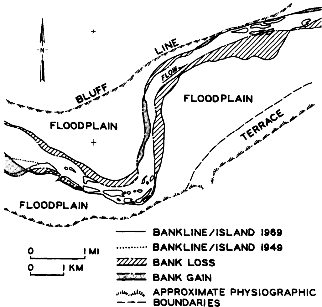
Figure C10. Changes in bankline occurring between 1949 and 1969 for a reach of the Missouri River below Garrison Dam (from Patrick 1977)
