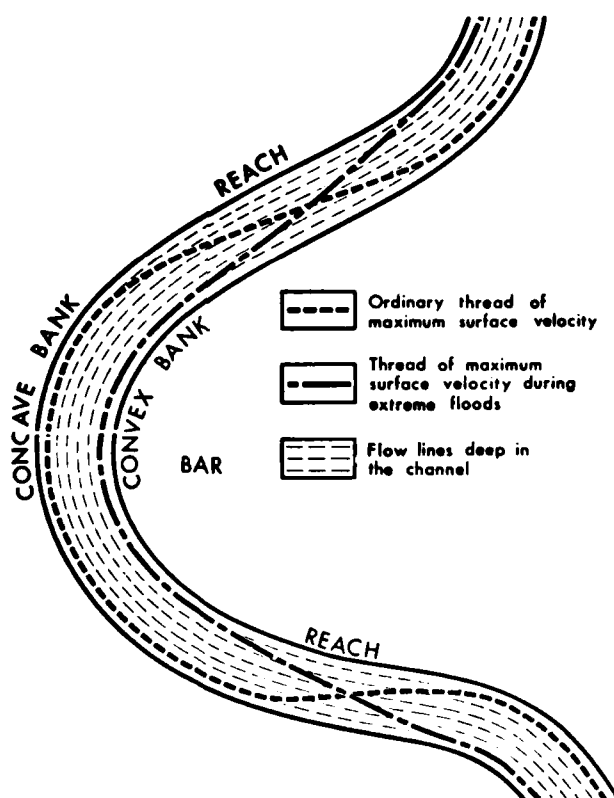
Figure C25. Velocity in a river bend during normal and flood flows (from Russell 1979)
