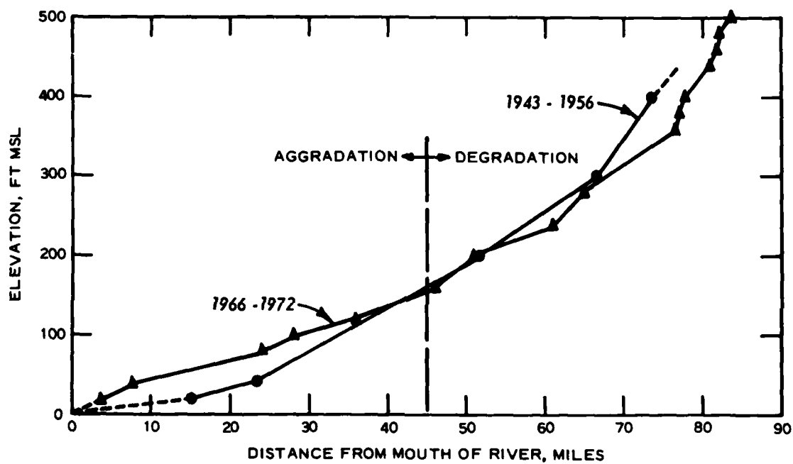
Figure C3. Changes in longitudinal profiles of the Eel River (from Smith and Patrick 1979)
