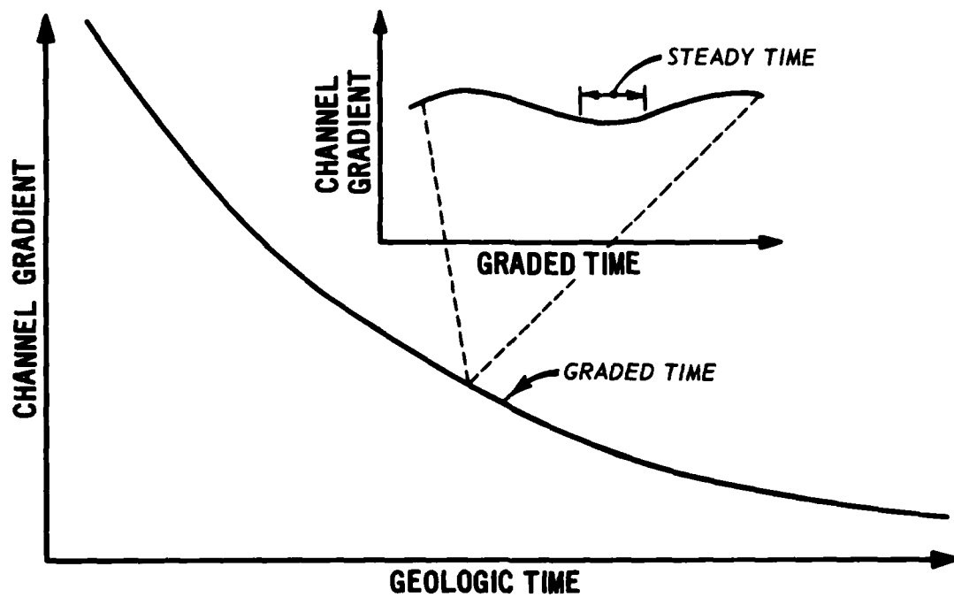
Figure C1. The influence of time on channel morphology (after Schumm 1971)
