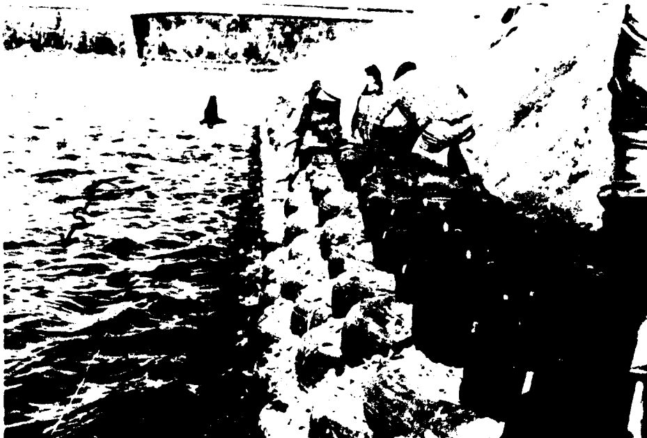
PHOTO 6 INSTALLING TIRE BULKHEAD OCTOBER 1980
