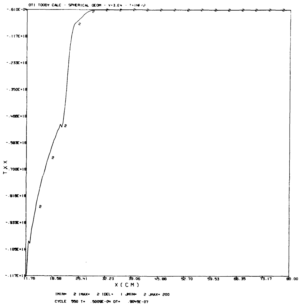
Figure 4. Stress Versus Distance at 50 Microseconds for Spherical Geometry, V=300 m/s.
