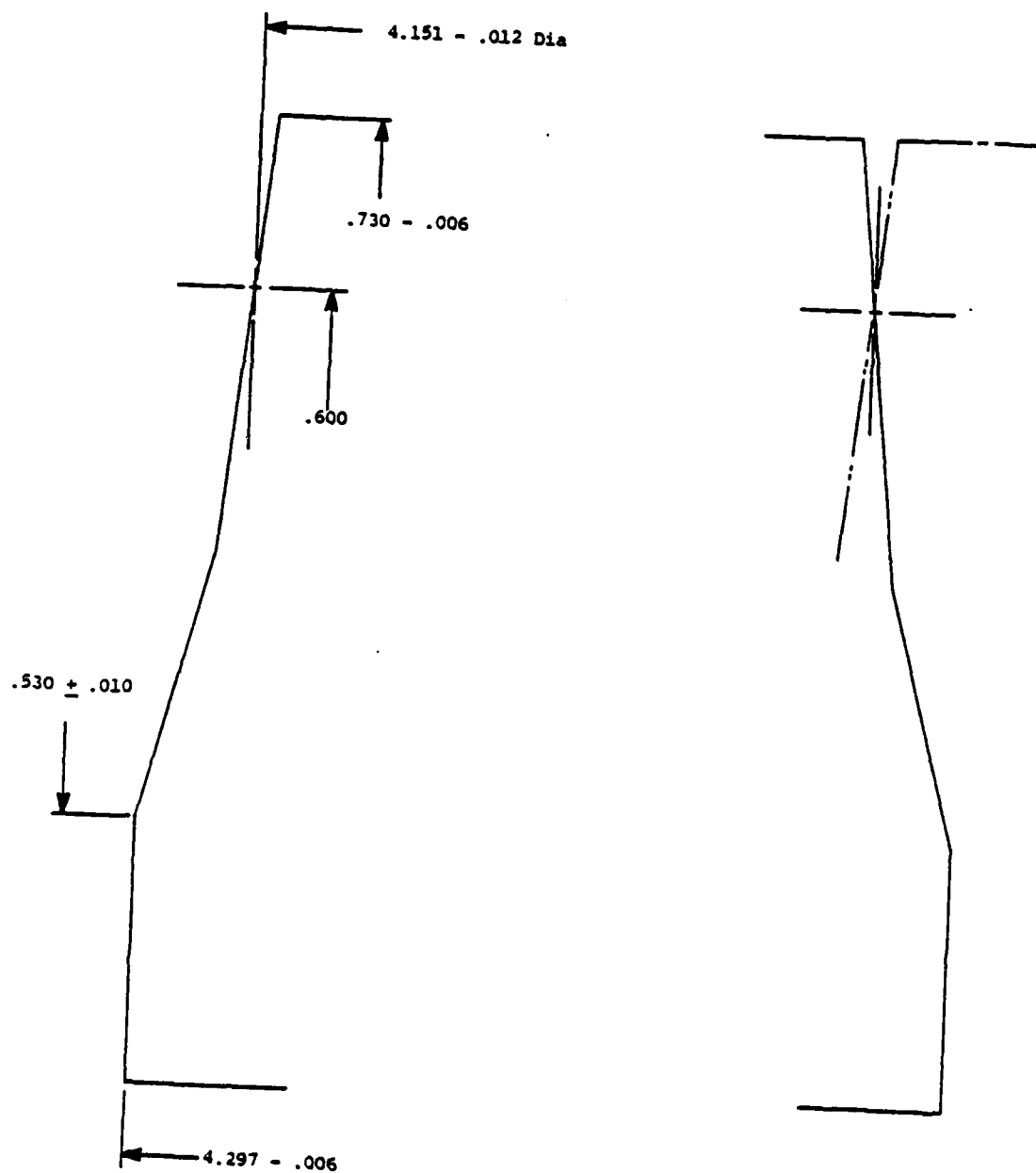
Figure 6. Optical Comparator Inspection Transparency
