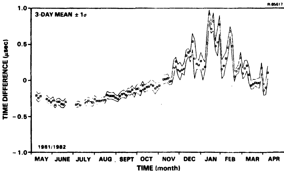
Figure 4.1-1 TDY Time Series at London Fixed-Site Monitor
