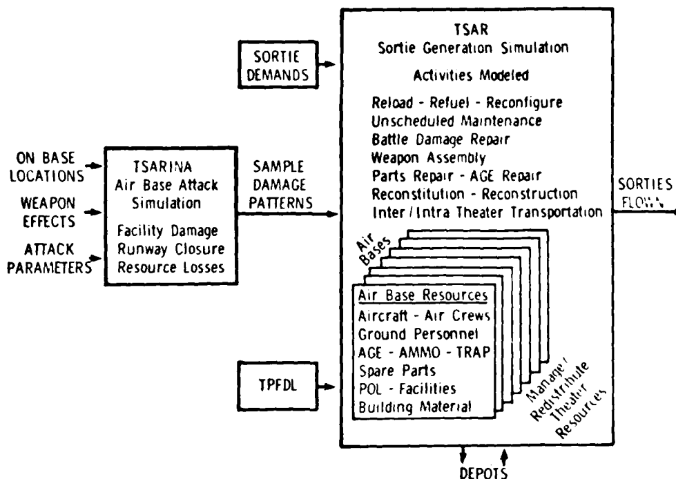
Fig. 2--TSAR-TSARINA -- For Analyzing Sortie Improvement Initiatives
