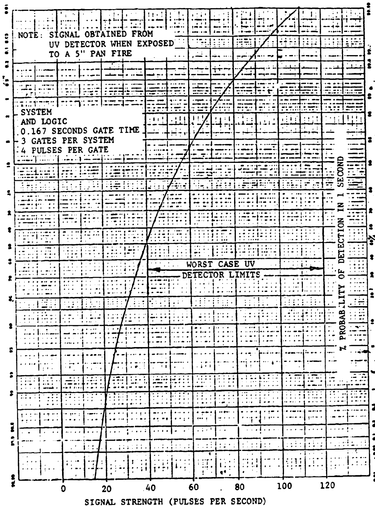
FIGURE 2-1 SIGNAL STRENGTH
