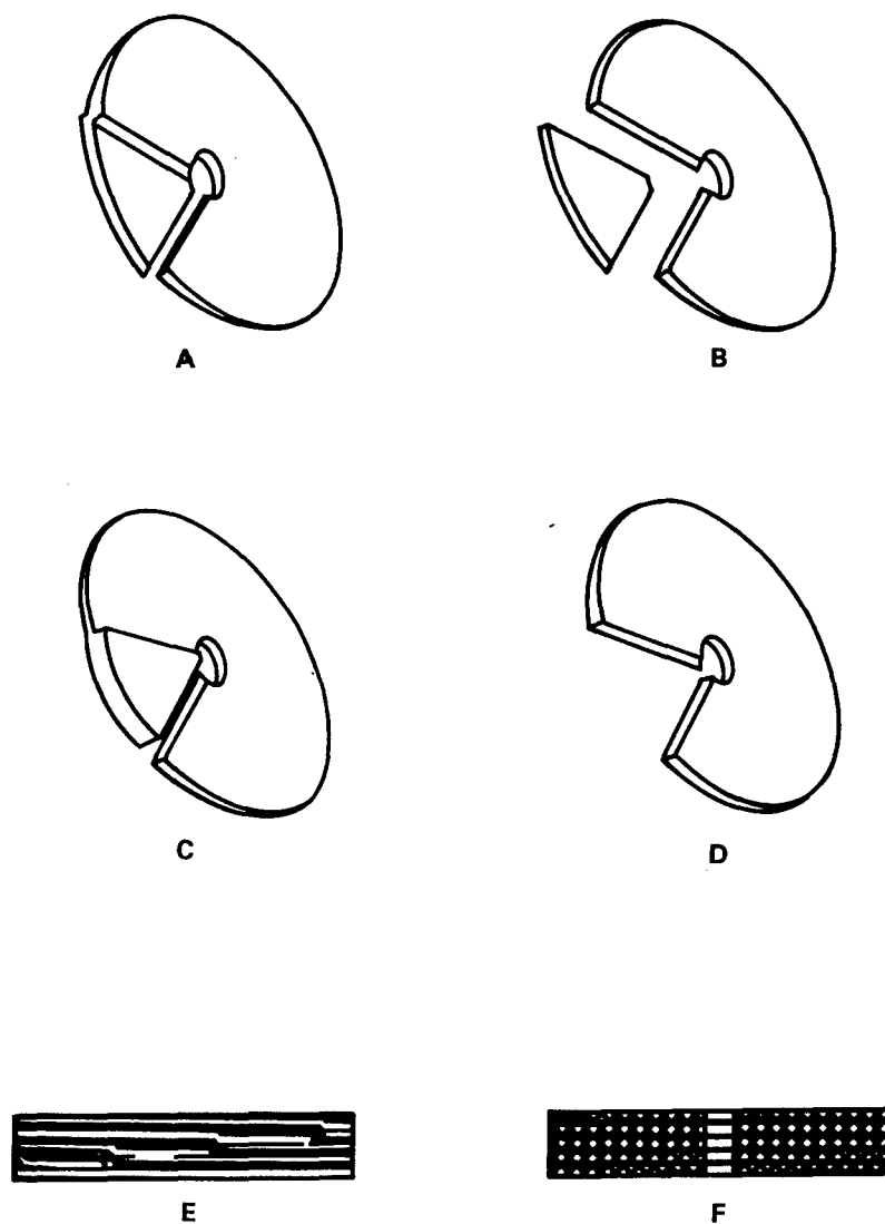
FIGURE 8 SCHEMATIC DIAGRAM DEPICTING COMPONENTS FOR A BITTER-TYPE, DISK INDUCTOR
