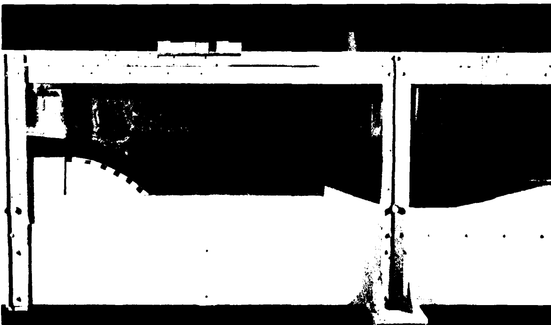
Photo 11. 1:29-scale section model of low-stage structure with type 4 design crest; discharge 3,100 cfs, tailwater el 228.0
