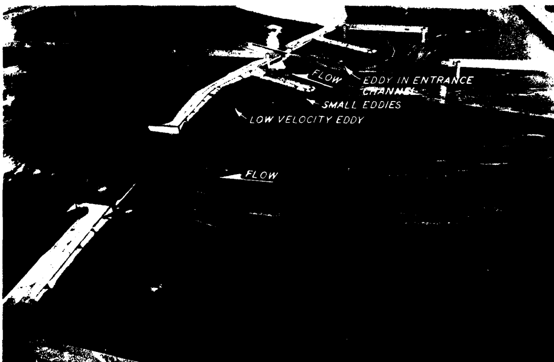
Photo 1. Flow conditions with the original design; discharge 14,800 cfs, tailwater el 234.3. Confetti accents surface flow patterns; exposure time 15 sec prototype
