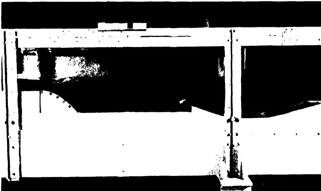
Photo 10. 1:29-scale section model of low-stage structure with type 3 design crest; discharge 3,100 cfs, tailwater el 228.0
