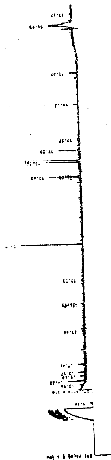
Figure E-5. Gas chromatogram of component(s) extracted from Core 13, position 1 on day 131.
