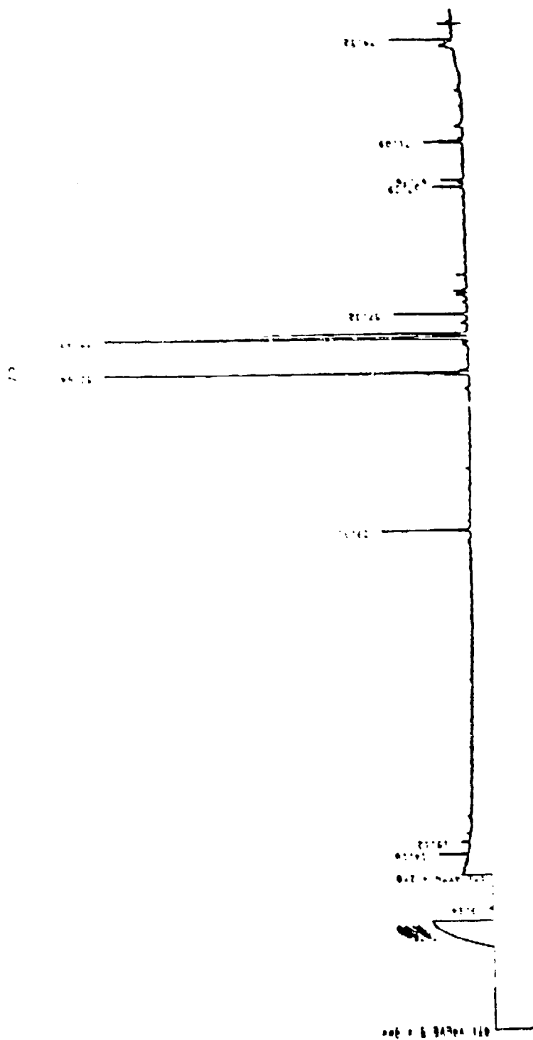
Figure D-4. Gas chromatogram of component(s) extracted from Core 12, position 1 on day 89.
