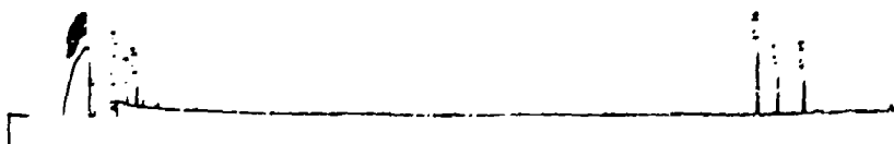
Figure B-4. Gas chromatogram of pentane extracts from biodegradation of model JP-5, B 2 -16.25 \mu L-standard, day 7, 10, 18, 24.
