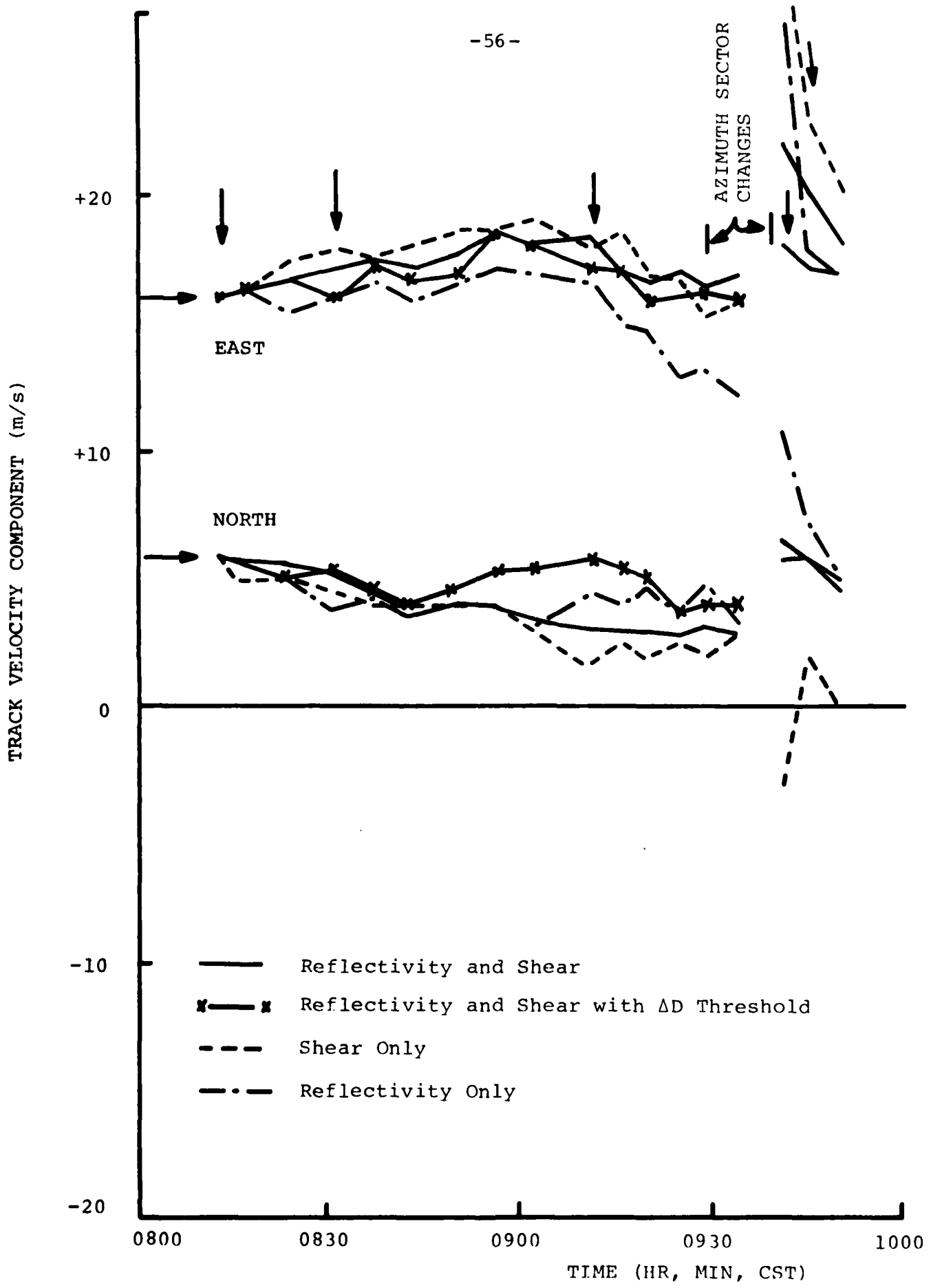
FIGURE 14. Average tracking velocities for the separate tracking runs.
