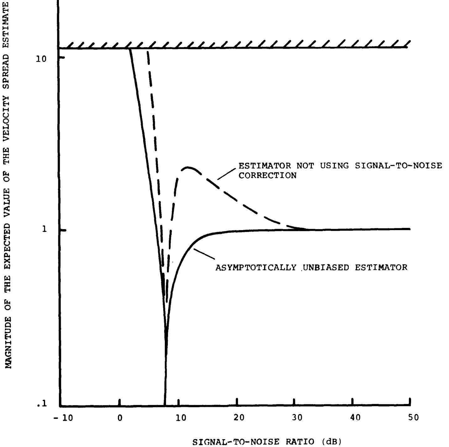
FIGURE 3. Doppler spread (spectrum width) estimation bias.
