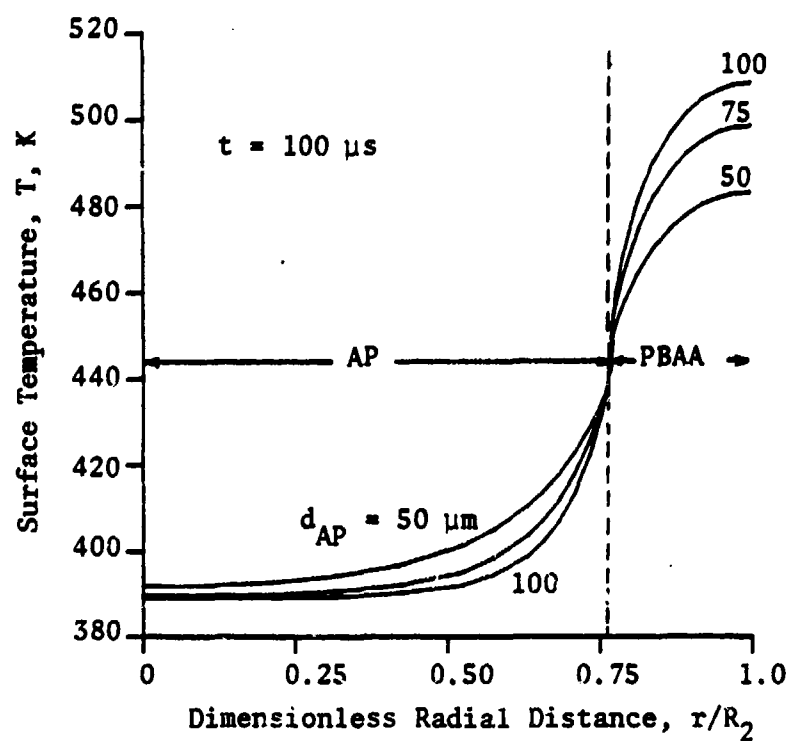
Fig. 13 Effect of AP Particle Size on Radial Variation of Surface Temperature (Average dP/dt = 120 GPa/s)
