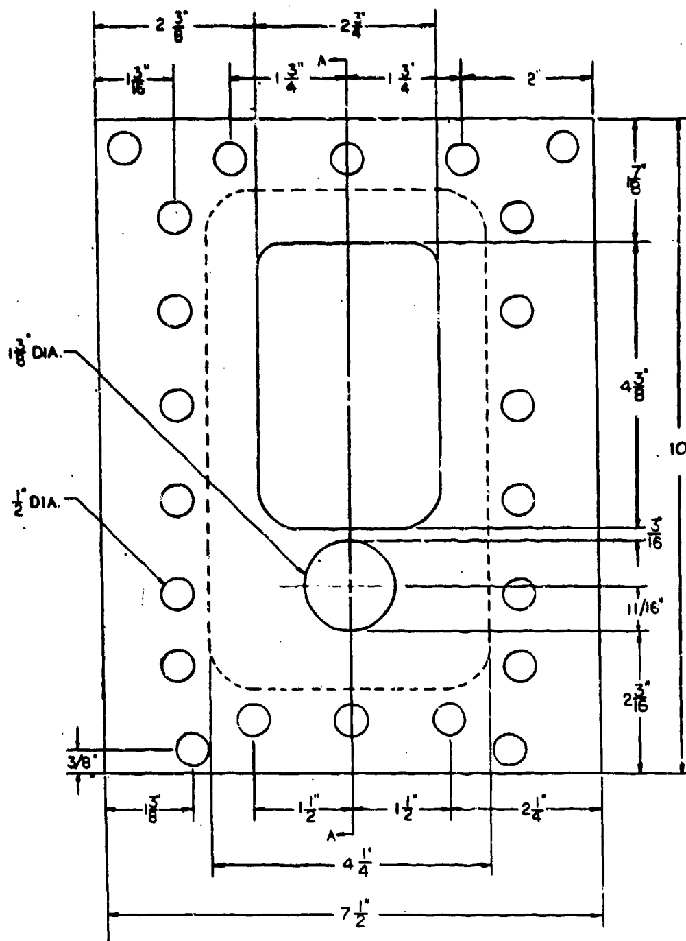
Fig. 25 Front View of the Window Retainer Plate
