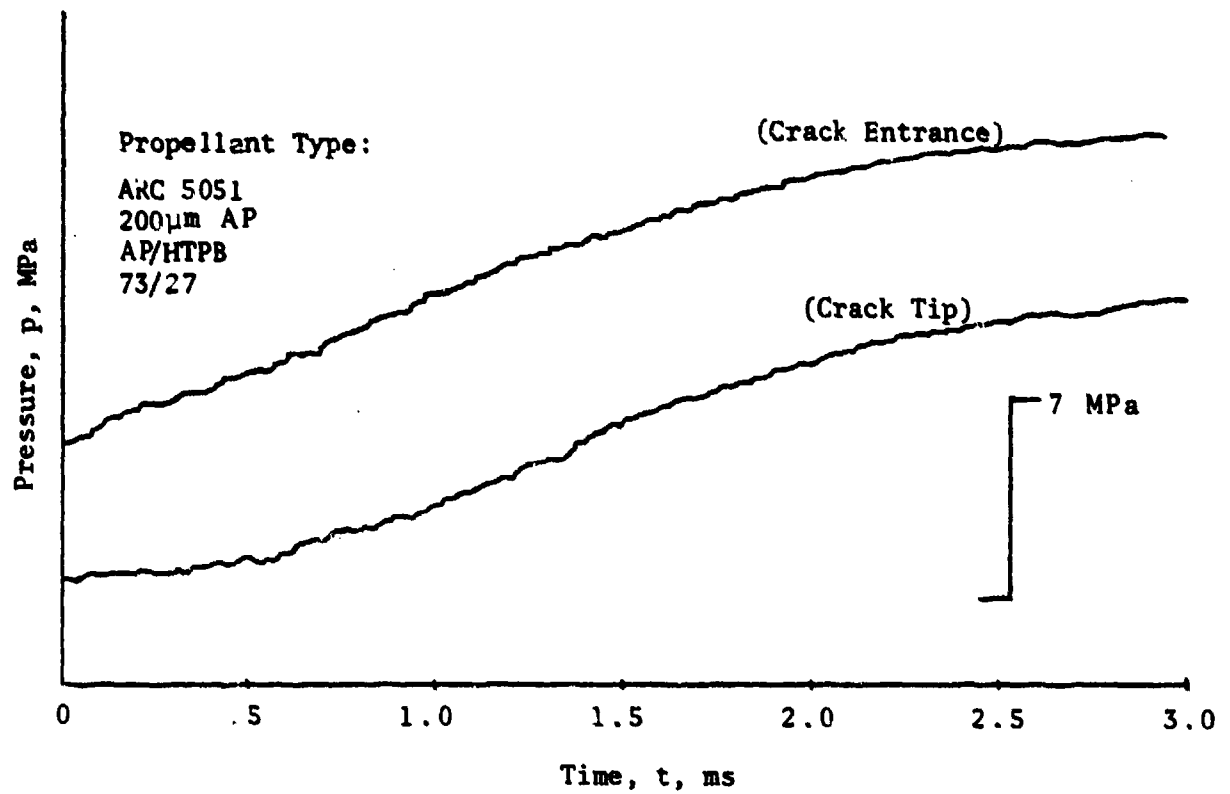
FIG. 19 PRESSURE-TIME TRACE FOR CRACK PROPAGATION TEST (TEST No. DNCPI-7; dp/dt = 4 \times 10^5 MPa/s DURING MEASURED CRACK PROPAGATION)
