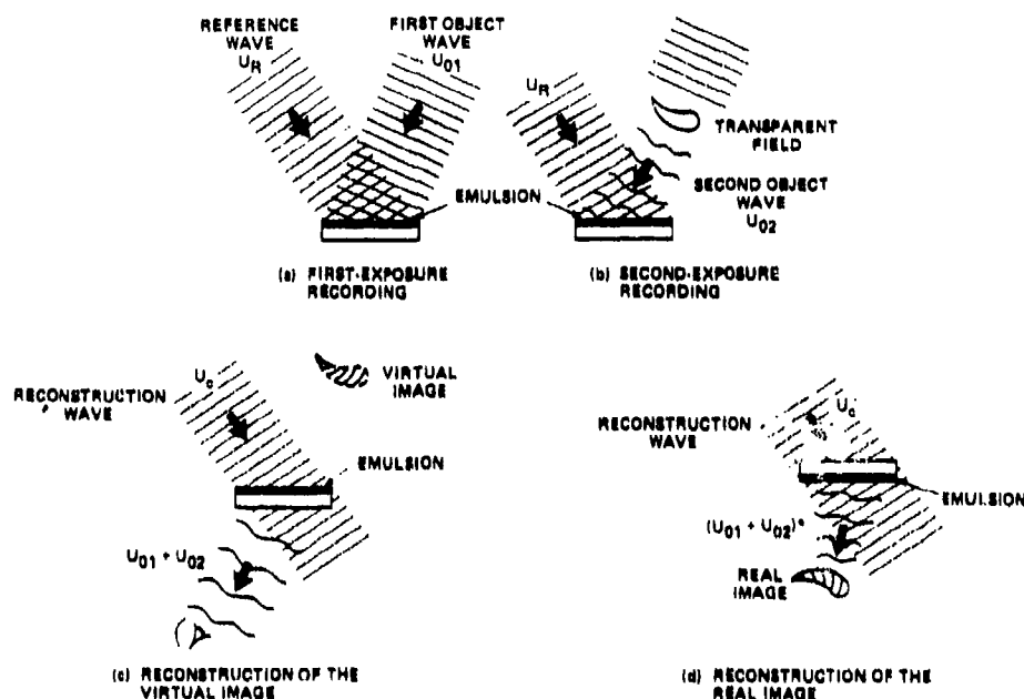
Figure 4. Double-exposure holographic interferometry.
