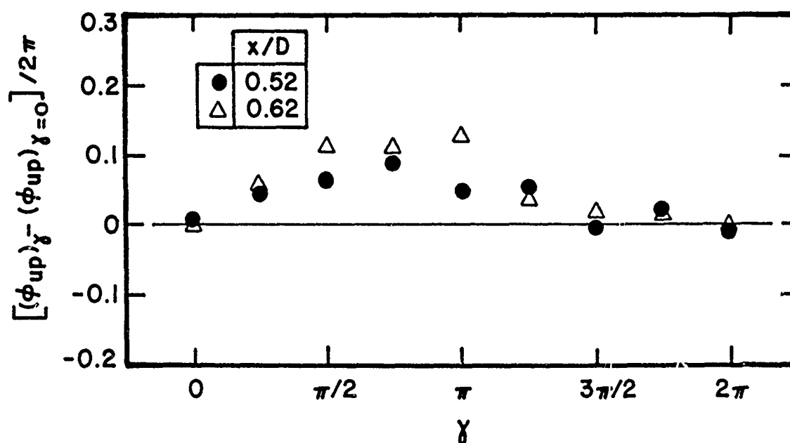
Figure 122. Azimuthal Variation of Phase Difference Between Velocity and Near-Field Pressure for Initial Axisymmetric Mode at Re = 52,000 for Case 1L
