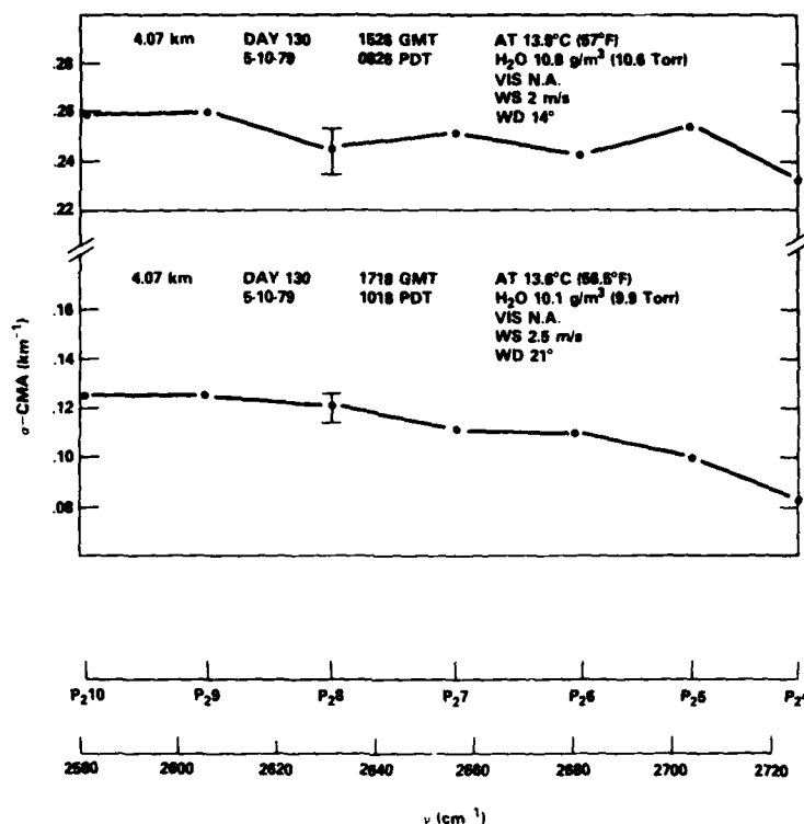
Fig. 10 — Measured extinction coefficients minus calculated molecular absorption coefficients vs wavenumber for NRL measurements at SNI of several DF laser lines
