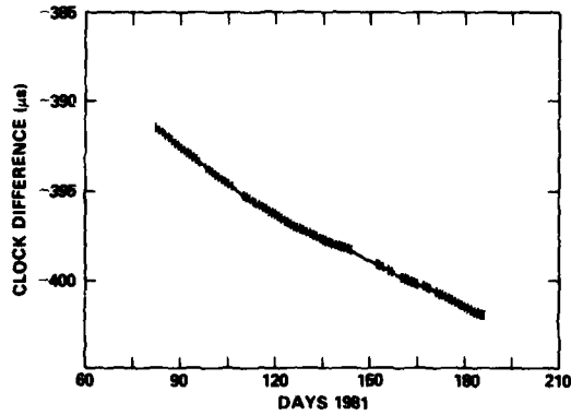
Fig. 5 - 100 days of clock differences between NAVSTAR-6 (SV9) and the GPS Vandenberg Monitor Site (VMS)
