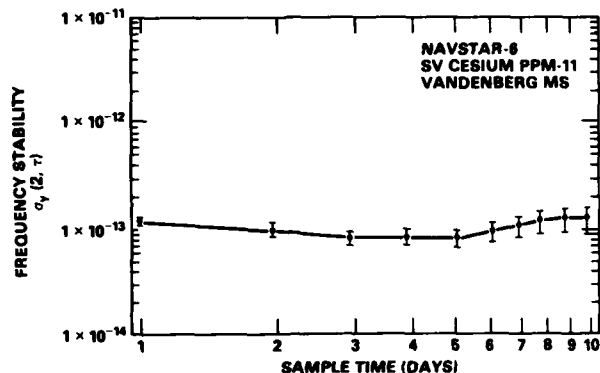
Fig. 9 — NAVSTAR-6 Cesium Clock (PPM-11) on-orbit clock/ephemeris frequency stability for 1- to 10-day sample times
