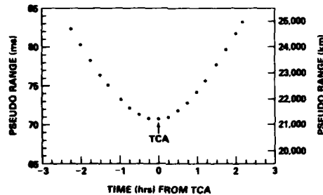
Fig. 2 — Typical NAVSTAR pseudo-range signature, plotted every 15 min
