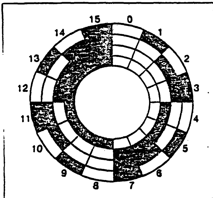
An absolute shaft encoder utilizing a binary code.
