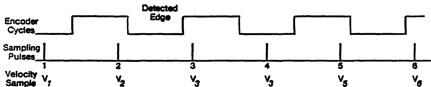
CONSTANT VELOCITY OF ROTATION
