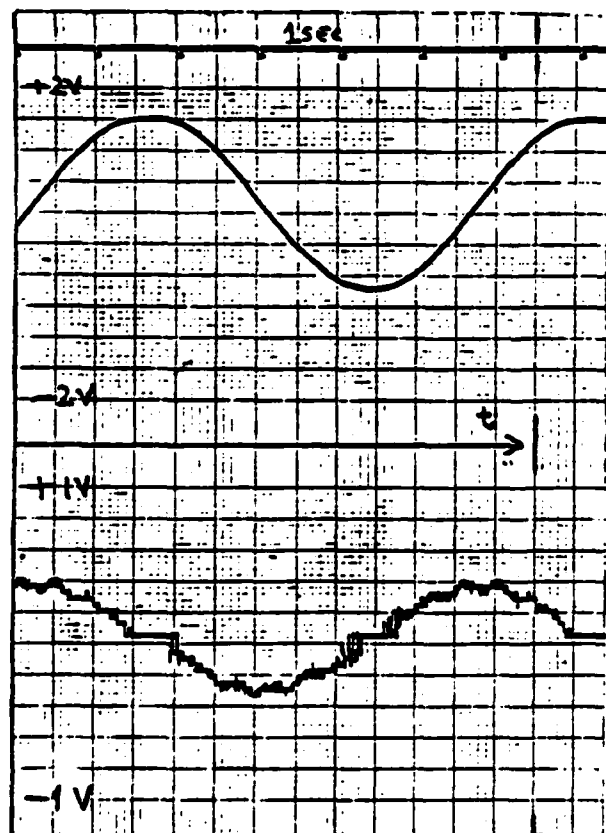
FIG.8. SINUSOIDAL VARIATION IN POSITION AND VELOCITY. (JOINT-6)
