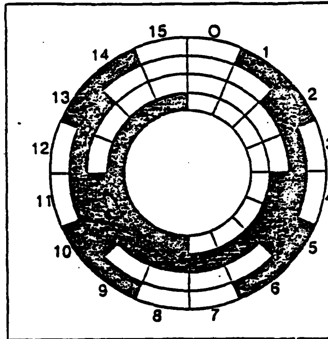
An absolute shaft encoder utilizing a grey code.
