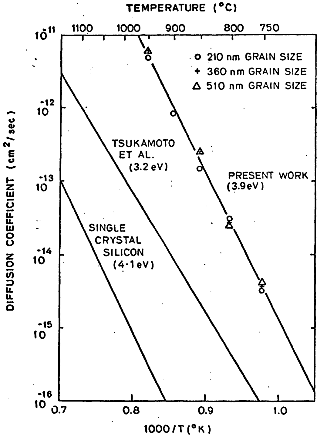
Fig. 15.2: The diffusion coefficient of arsenic in the polysilicon grain boundaries as a function of temperature. Also shown are the data of Tsukamoto et al. [15.16] as well as the diffusivity of arsenic at low concentrations in single-crystal silicon [15.6].
