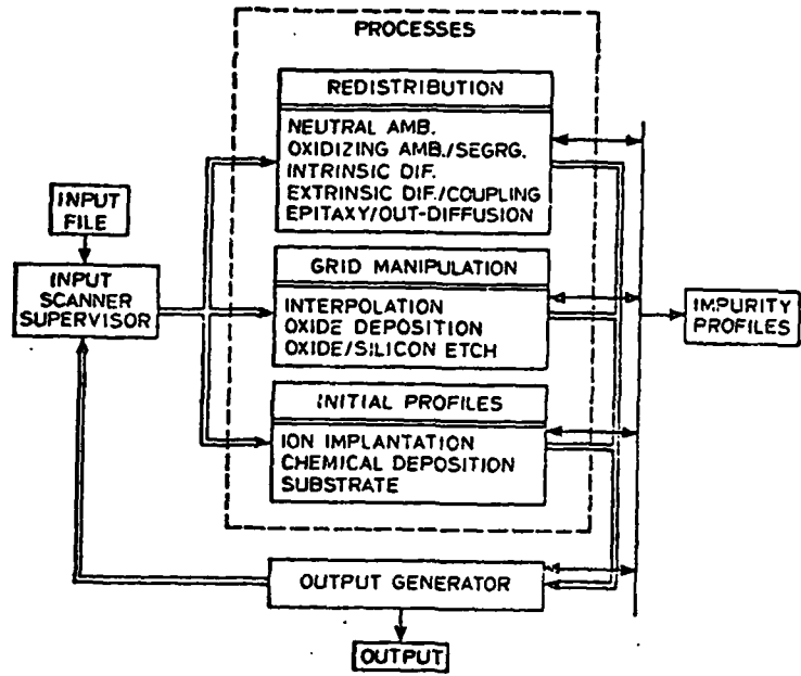
Fig. 1.1: Basic structure of SUPREM Process Modeling Program.
