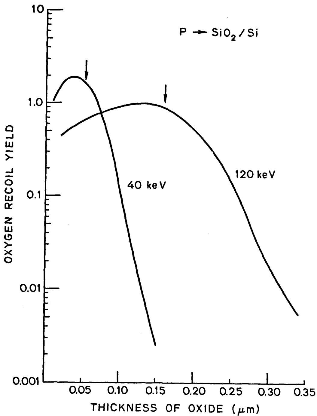
Fig. 12.3: Oxygen recoil yield as a function of oxide thickness for implantations of phosphorus into SiO 2 on silicon. Arrows indicate the projected range R_p for each energy.
