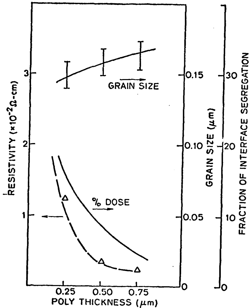
Fig. 1.30: Resistivity, grain size and fraction of dopant segregated at grain boundaries as functions of poly thickness for phosphorus doped films annealed at 950°C for three hours.
