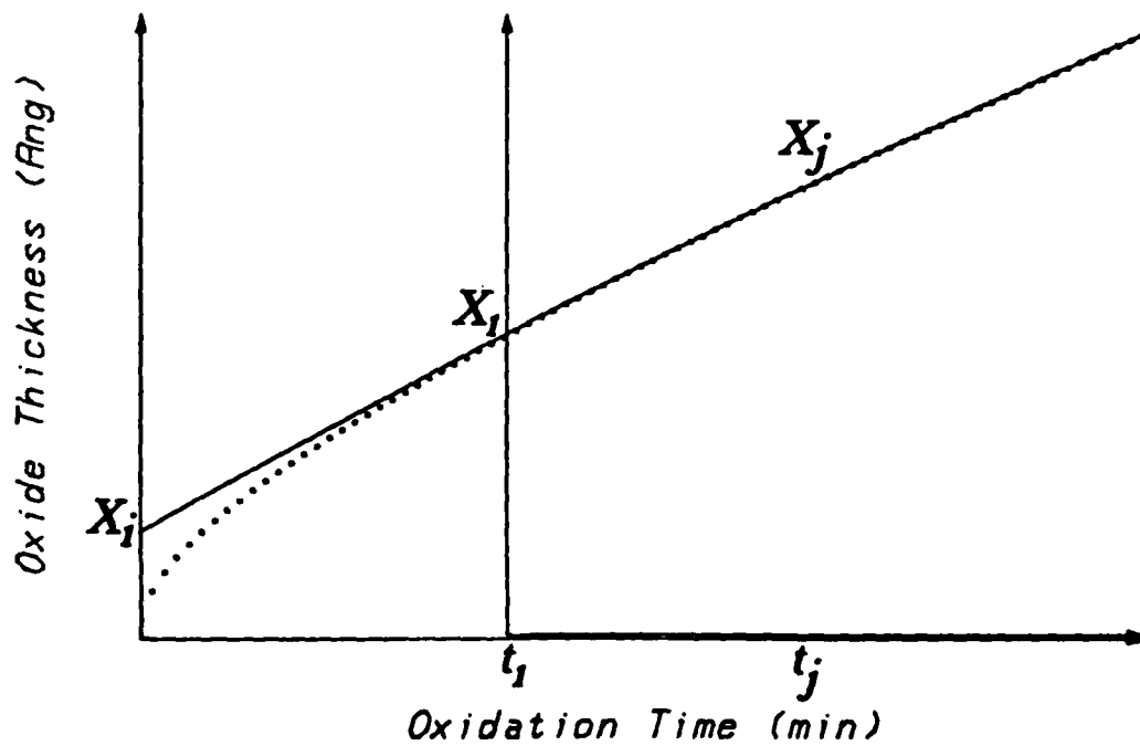
Fig. 5.3: Linear and parabolic rate constants extraction by shifting the time axis to t_1 and fitting the data beyond X_i .
