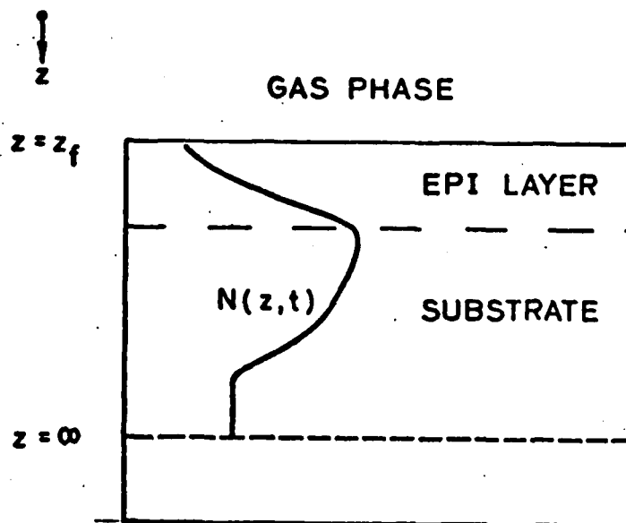
Fig.1.22: Schematic cross-section of a silicon wafer for the purpose of solving Fick's Second Law.
