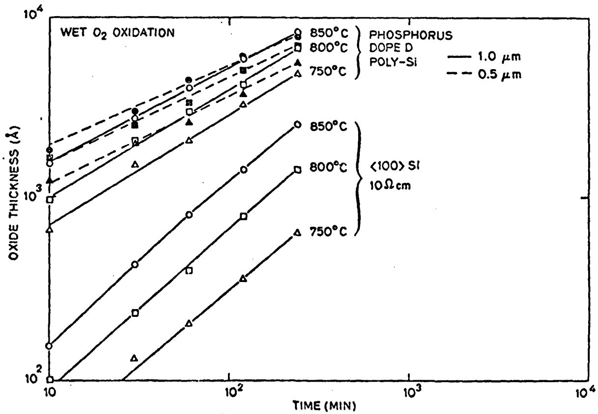
Fig. 1.27: Oxide thickness vs. oxidation time for steam ( \text{O}_2 bubbled through 95^\circ\text{C} \text{H}_2\text{O} ) oxidation of phosphorus doped polysilicon films and lightly doped \langle 100 \rangle silicon.
