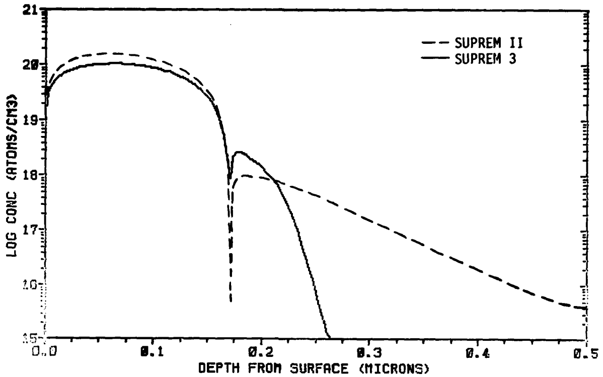
Fig. 1.17: SUPREM II and SUPREM III outputs for the bipolar example of Fig. 1.16.
