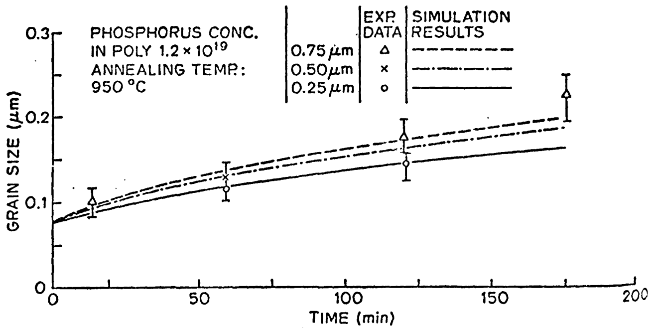
Fig. 1.26: Change in average grain-size as a function of annealing time at 950^\circ\text{C} for three different thicknesses of poly.
