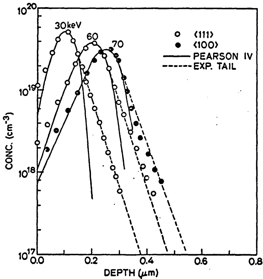
Fig.1.12: Boron as-implanted profiles in (111) and (100) silicon in a random direction. Pearson IV and modified Pearson IV distributions were used. Dose is 10^{13}/\text{cm}^2 .
