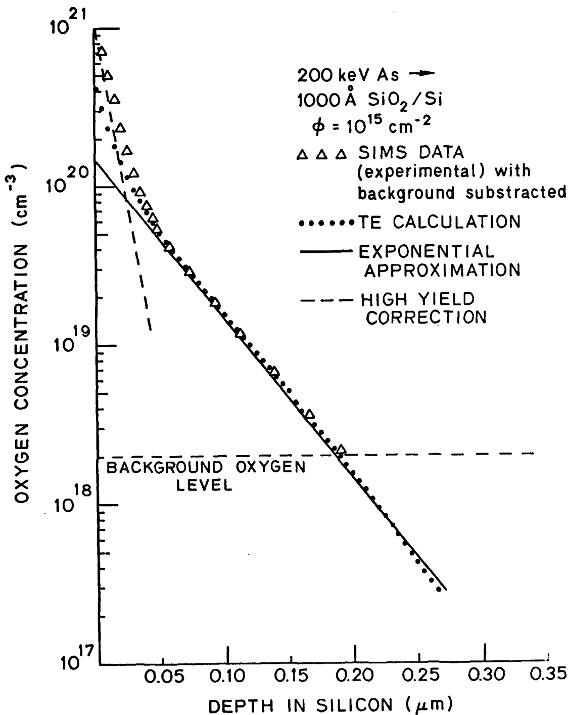
Fig. 12.1: Comparison of a TE calculation with experimental results from Magee et. al. [12.12] for the oxygen recoil distribution resulting from implantation of 200 keV As into 1000 Å \text{SiO}_2 on Si to a dose of 10^{15} \text{ cm}^{-2} . Also shown is the analytic (exponential) approximation (solid line) and the high yield correction (dashed line).
