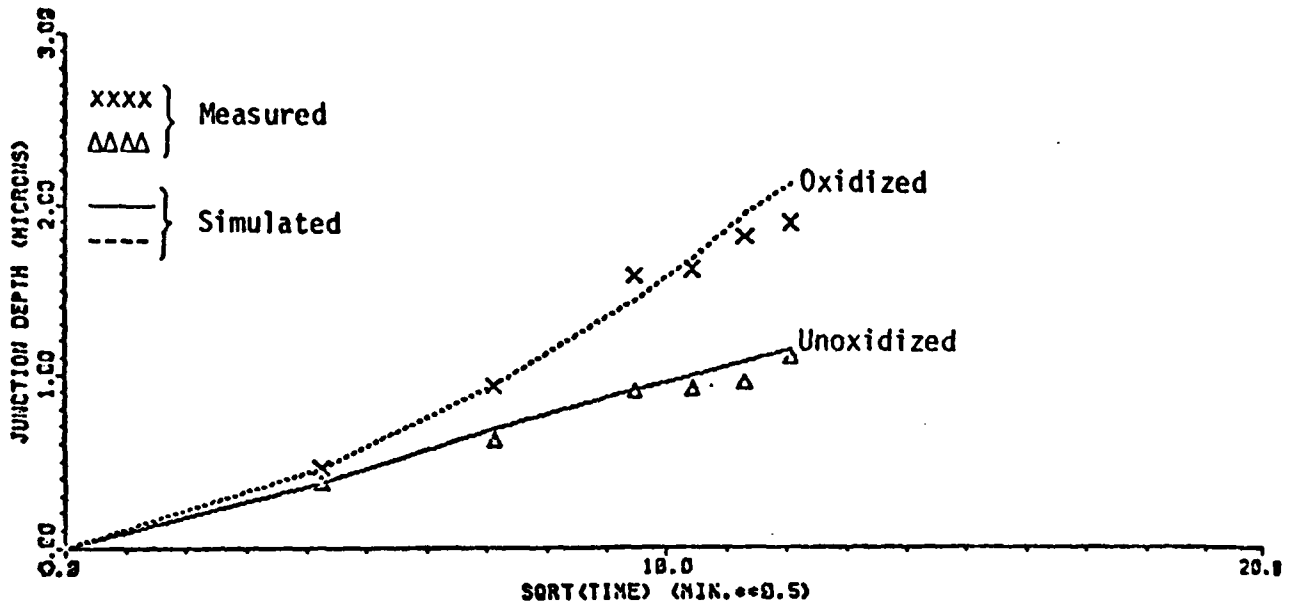
Fig. 1.33: Comparison of Theory (SUPREM) and experiment for junction depth vs. \sqrt{t} for a 3100 Å doped poly layer in oxidized and unoxidized regions (T = 1000°C).
