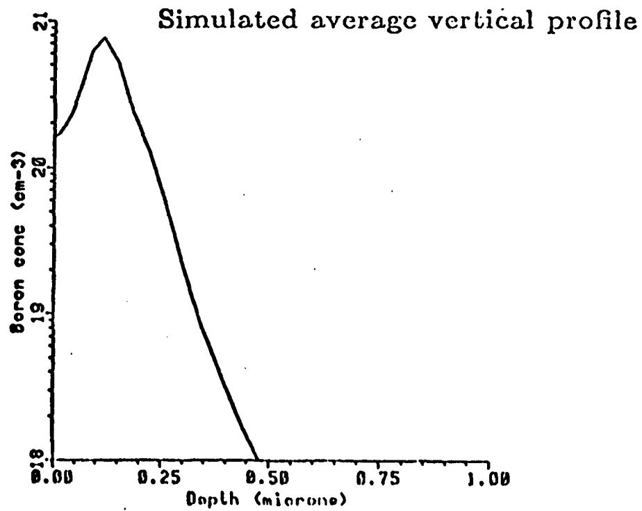
(b) Vertical profile of average boron concentration versus depth through the polysilicon layer.
