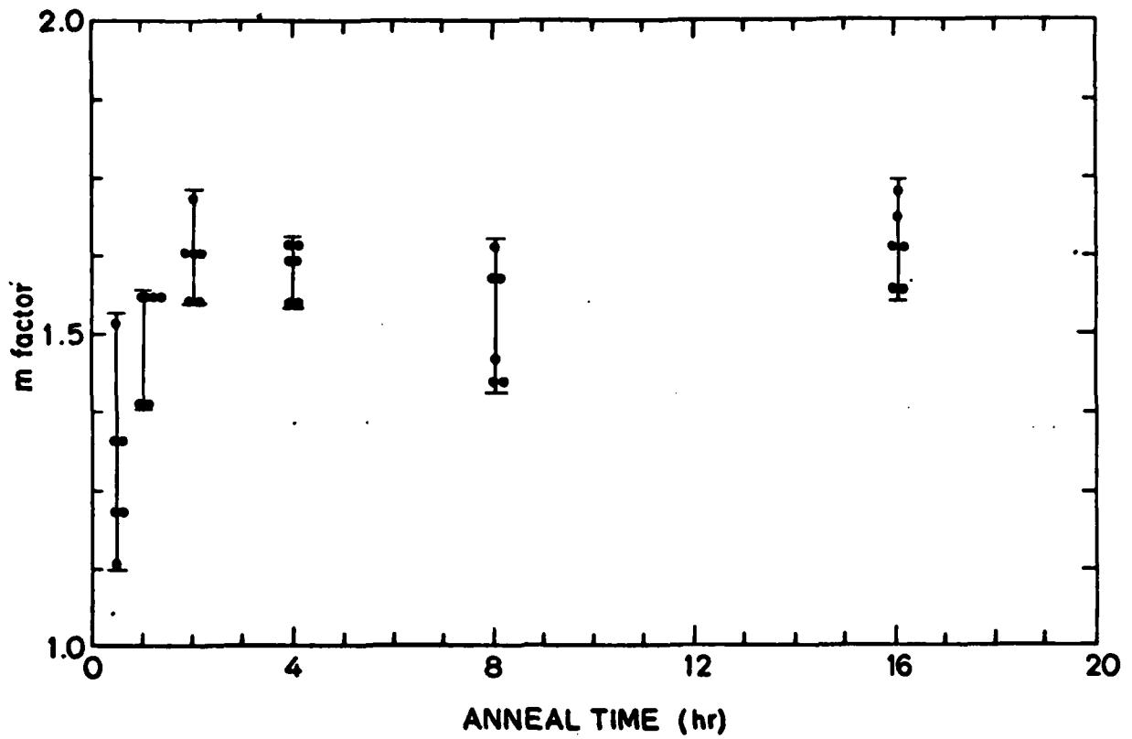
Fig. 13.7: Low current I_b slopes (m) of devices after successive gettering anneals at 850°C.
