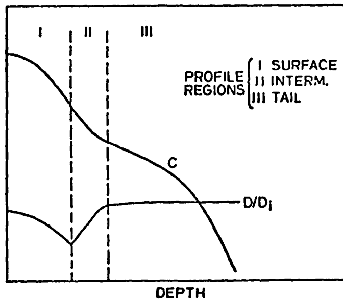
Fig.1.18: A typical phosphorus doping profile with a demarcation of the three regions considered by the Fair and Tsai model. Also shown in the local diffusivity profile derived by the model.
