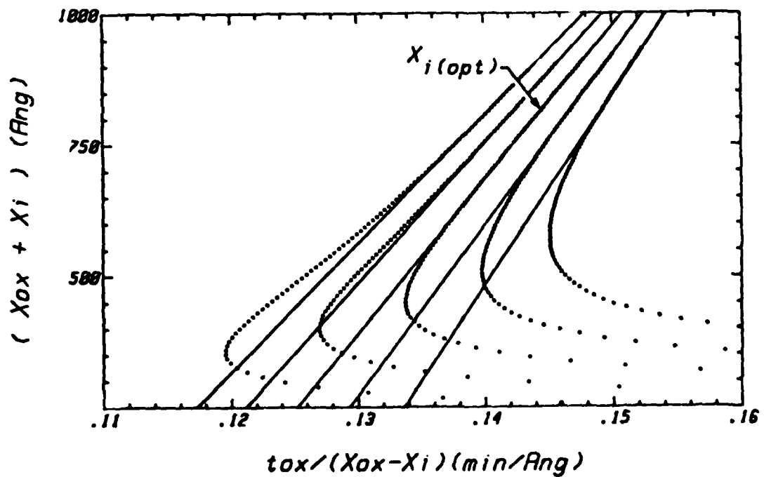
Fig. 5.6: Effect of X_i on extracted rate constants. The plots shown are for X_i = 100, 110, 120, 130 and 140 A.
