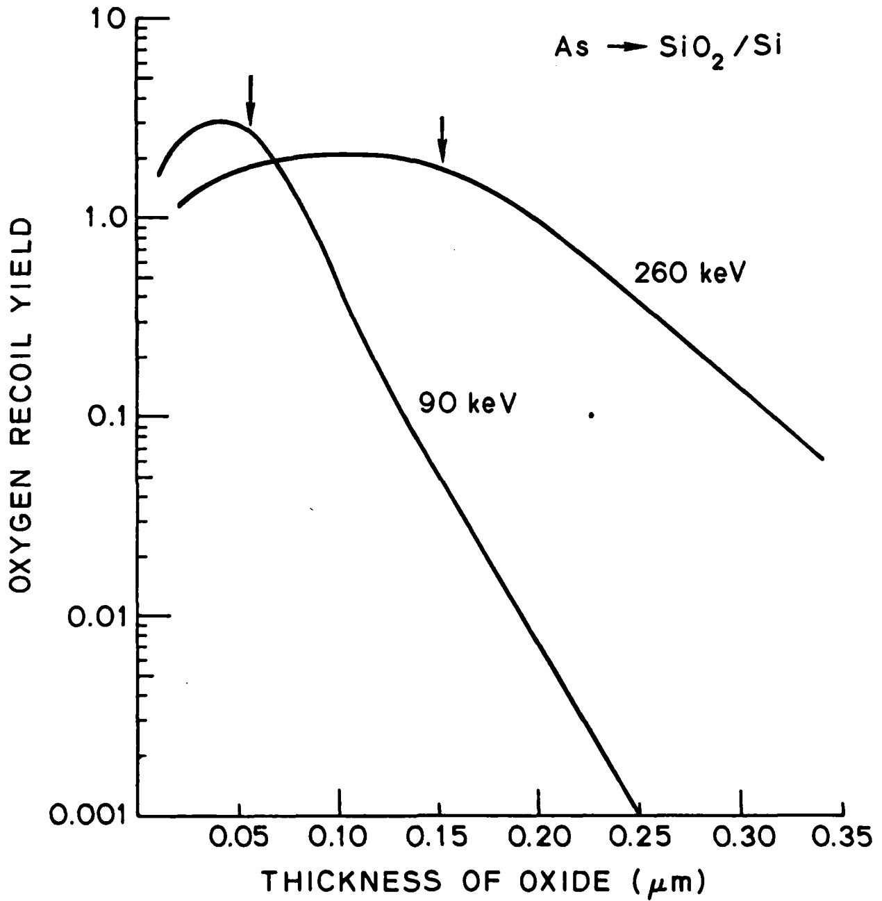
Fig. 12.4: Oxygen recoil yield as a function of oxide thickness for implantations of arsenic into SiO 2 on silicon. Arrows indicate the projected range R_p for each energy.
