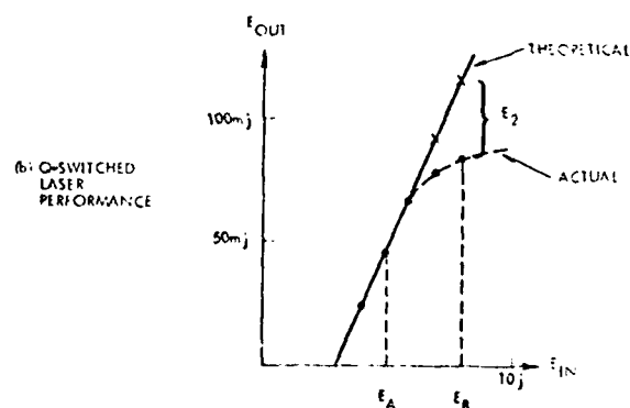
Fig. 1. Conventional Q-switched laser and its performance. The cavity is 46 cm long, and employs a 6.4 mm \times 76 mm airtron Nd:YAG rod.
