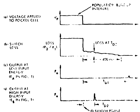
Fig. 2. Basic waveforms. The output pulse width is 20 nsec at E_{in} = E_B .
