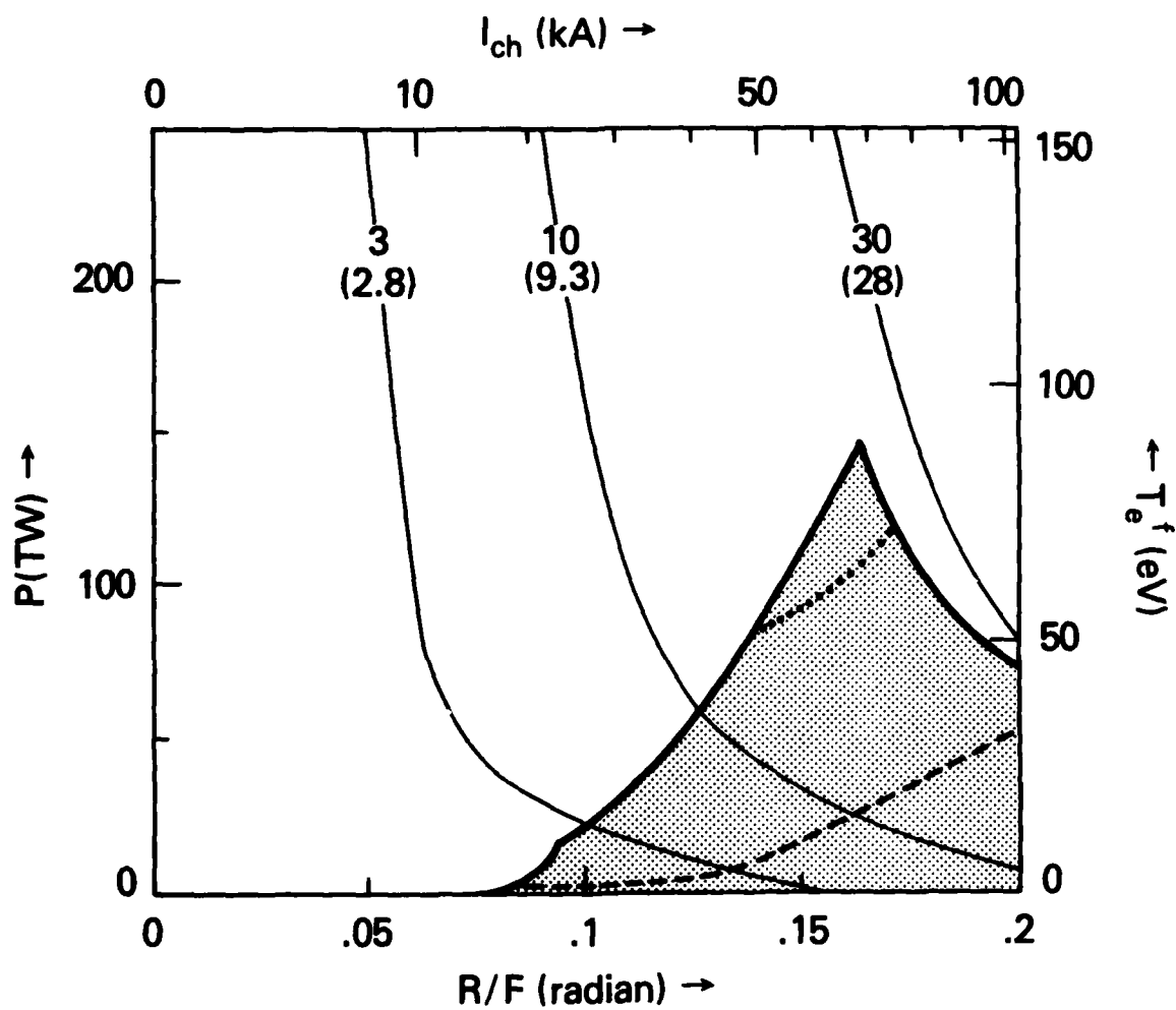
Figure 13 - Operational transport window for a H^{+1} beam with x = 2 , r_b = 1.5 cm, E_0 = 4 MeV and \tau_b = 1 \times 10^{-8} s.
