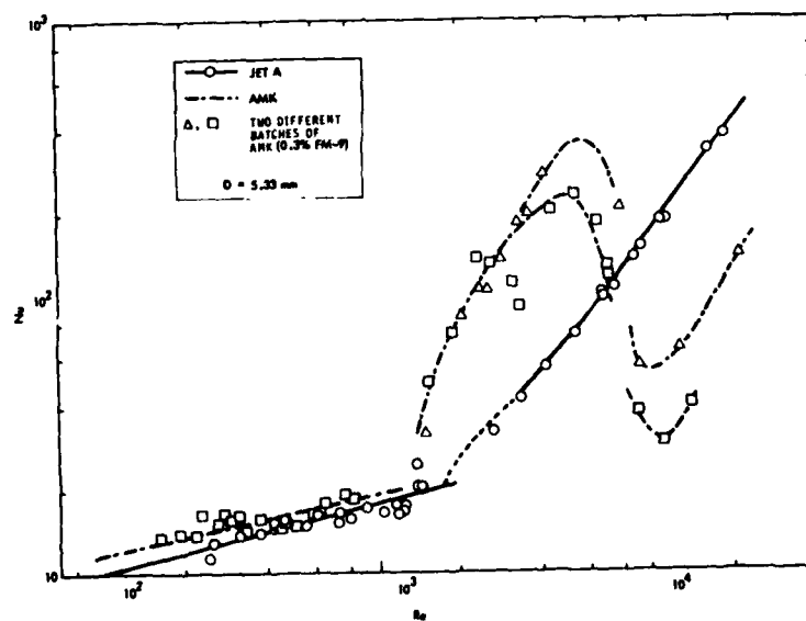
FIGURE 17. HEAT TRANSFER OF JET A AND 0.3% M-9 AMK; Re = Re_b , D = 5.33 \text{ MM}
