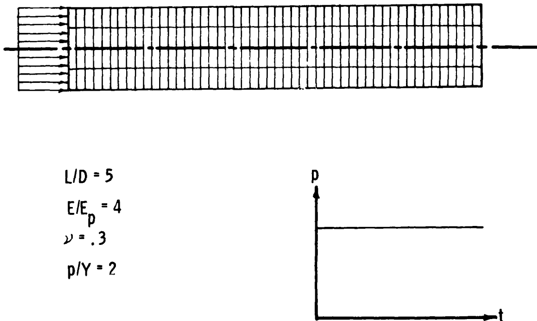
FIGURE 7. Elastic-Plastic Rod Subjected to Step Pressure at One End.
