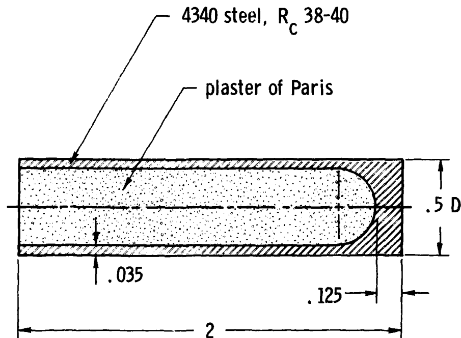
FIGURE 11. Cross-Sectional View of Projectile Used for Oblique Firings.
