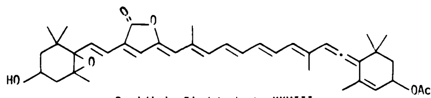
Peridinin 5'-dehydrate XXVIII
