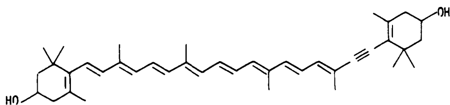
Diatoxanthin XXIII
