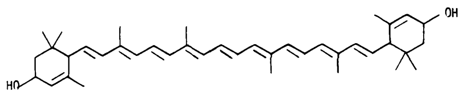
Tunaxanthin XXI
