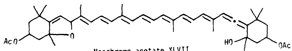
Neochrome acetate XLVII
