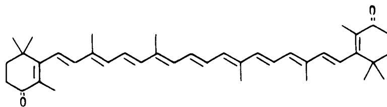
Canthaxanthin XXV
