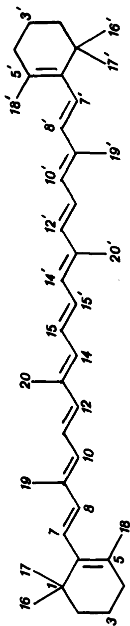
\beta -Carotene (II)
