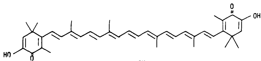
Astacene IX
