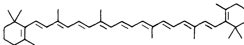
̢-carotene I
