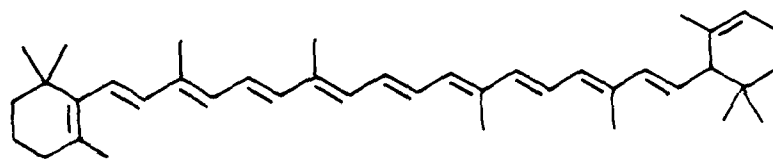
\alpha -carotene XLVI
