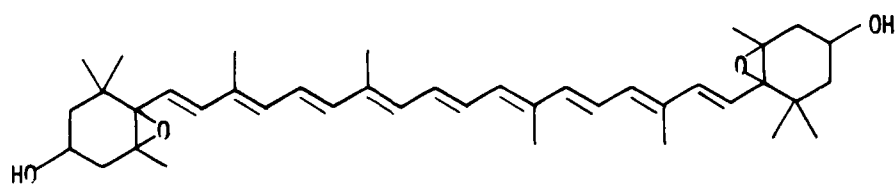
Violaxanthin XXII
