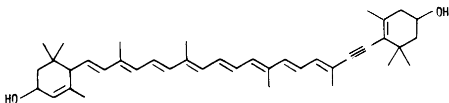
Monadoxanthin XXIV
