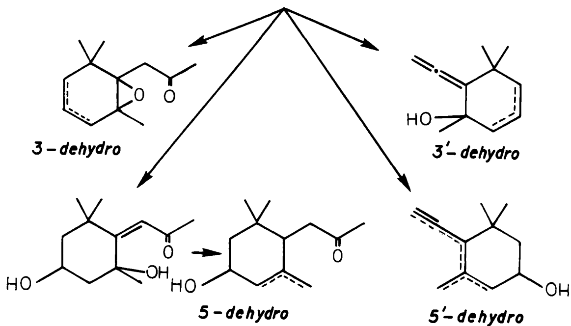
FUCOXANTHINOL
