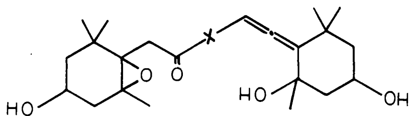
FUCOXANTHINOL
