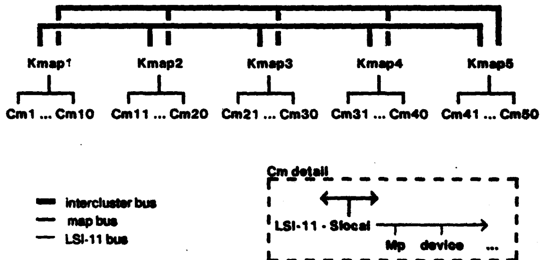
Figure 7.1. Cm* Architecture
