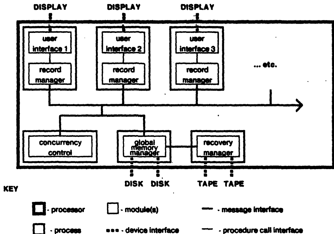
Figure 2.3. Centralized System
