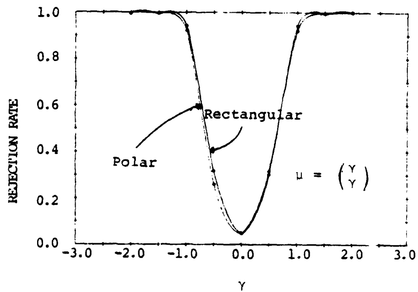
FIGURE 3: POWER CURVES FOR SHIFTS IN MEAN
