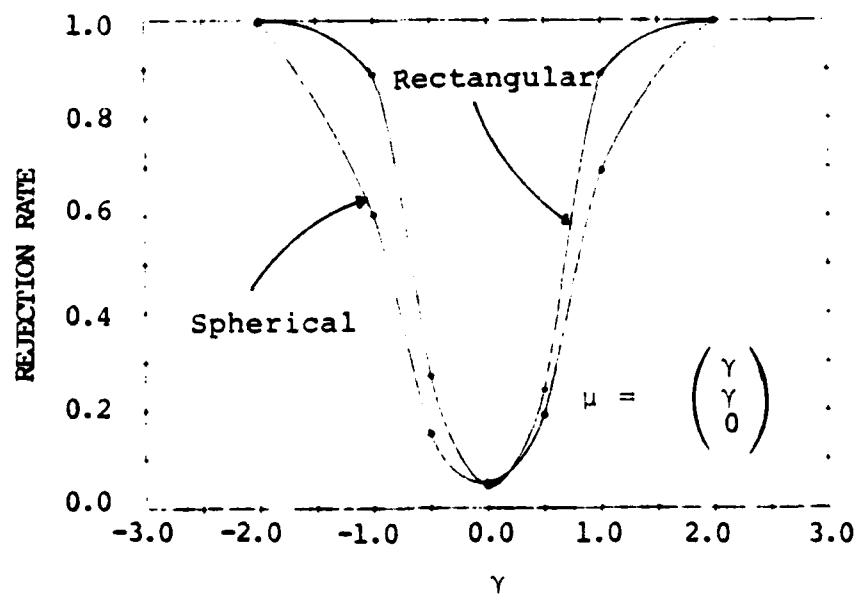
FIGURE 4: POWER CURVES FOR SHIFTS IN MEAN
