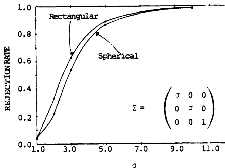
FIGURE 6: POWER CURVES FOR SHIFTS IN VARIANCE
