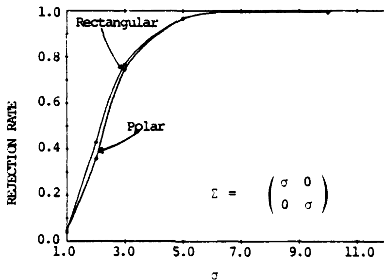
FIGURE 5: POWER CURVES FOR SHIFTS IN VARIANCE
