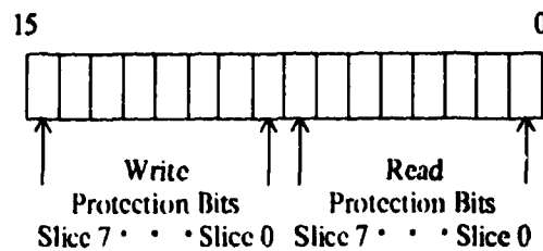
Figure 14: Slice Protection Register
