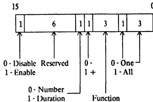
Figure 16: Monitor Control Register Format
