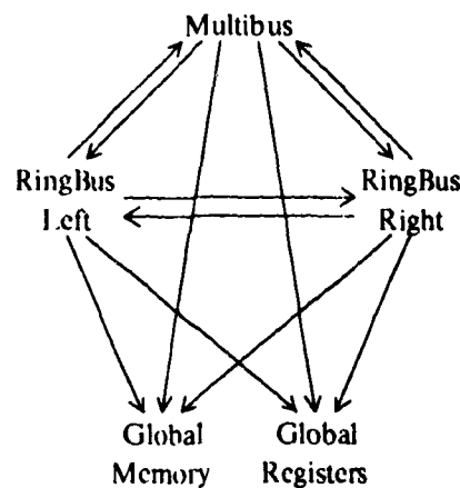
Figure 18: Possible Access Paths in the RIB
