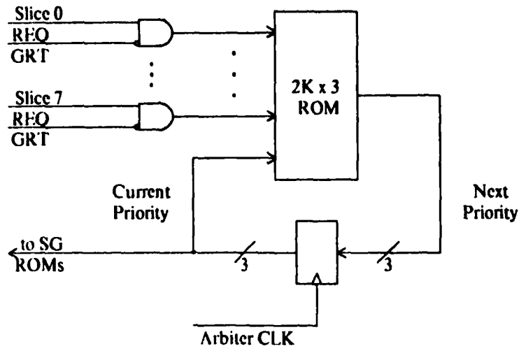
Figure 27: Concert Arbiter Priority Implementation
