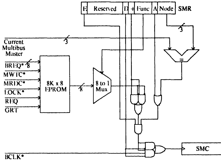
Figure 17: Hardware Monitor Support
