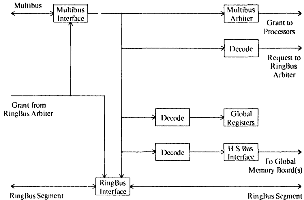
Figure 10: RingBus Interface Board
