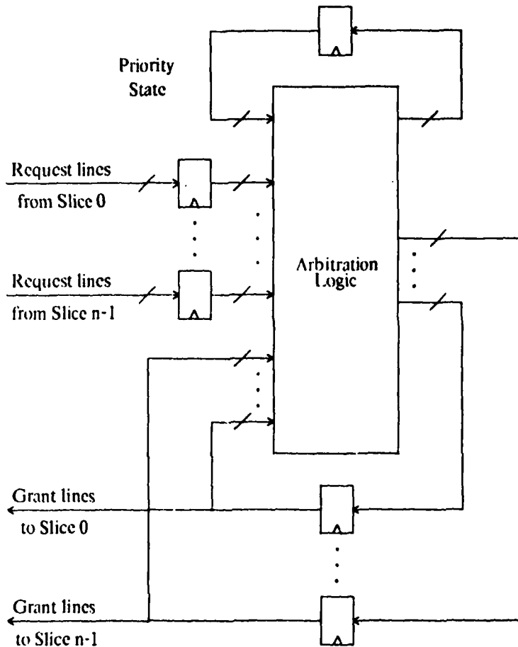
Figure 6: Model of Arbiter with Priority
