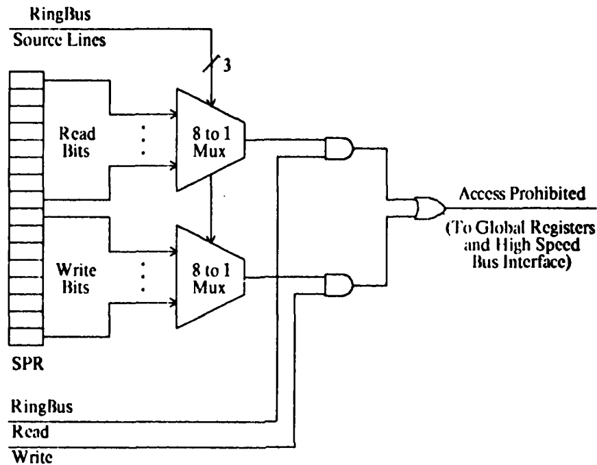
Figure 15: Hardware Protection Support
