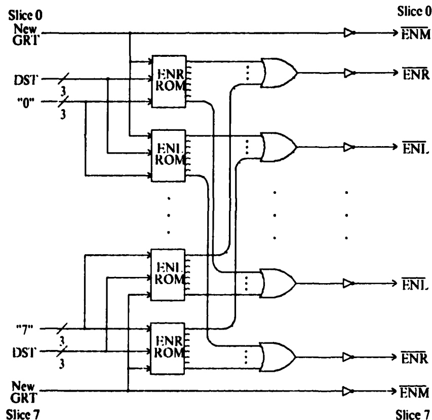
Figure 25: Arbiter Enable Signal Generation
