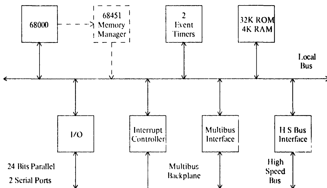
Figure 8: Concert Node — DBC68K Board
