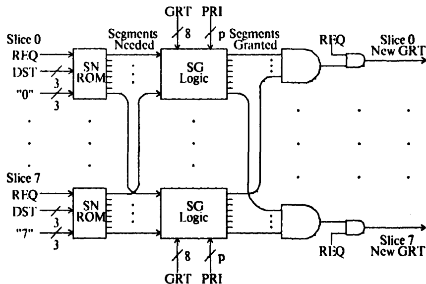
Figure 24: Criss-Cross Arbiter Implementation
