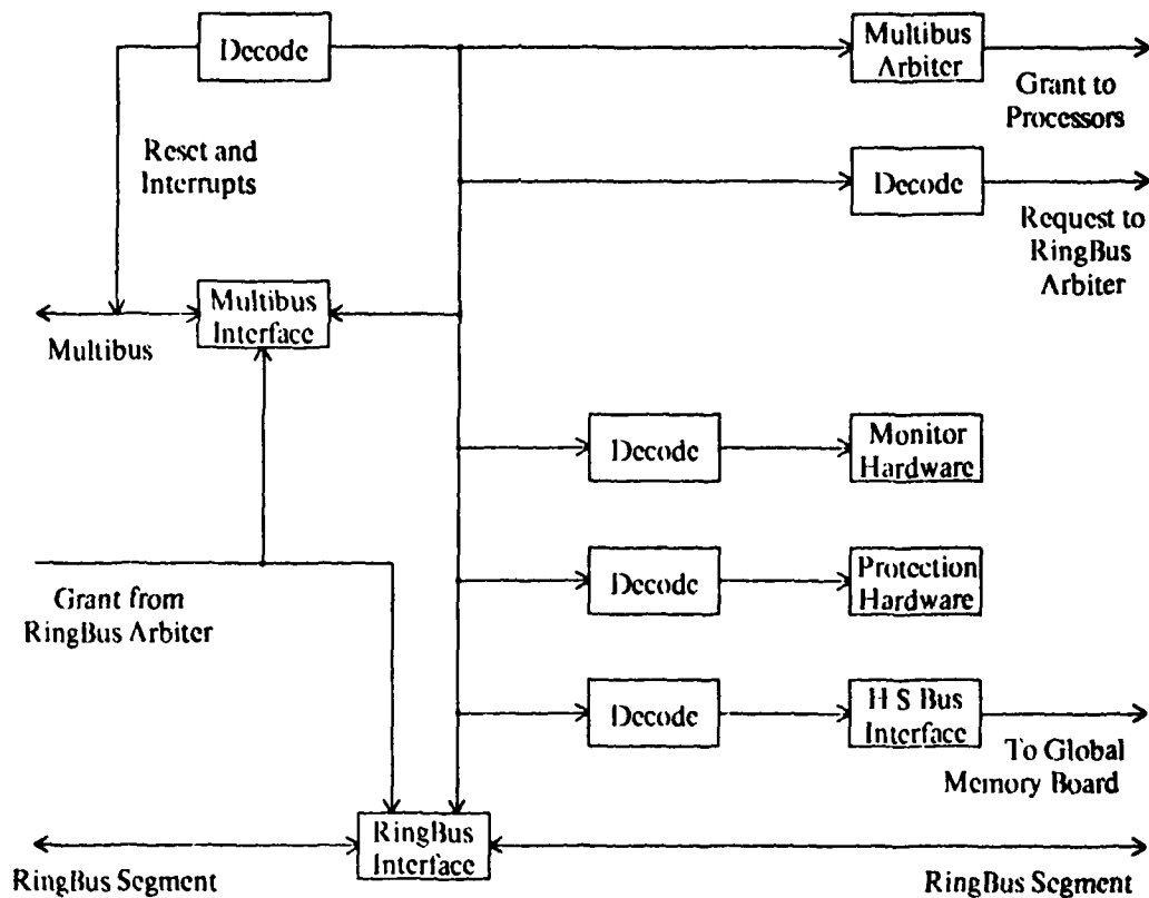
Figure 13: RingBus Interface Board Block Diagram
