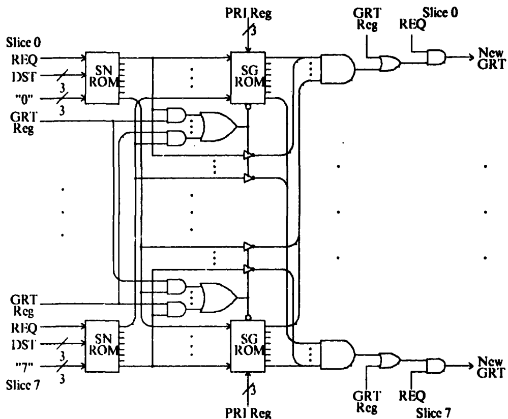
Figure 26: Concert Arbiter Design Scheme
