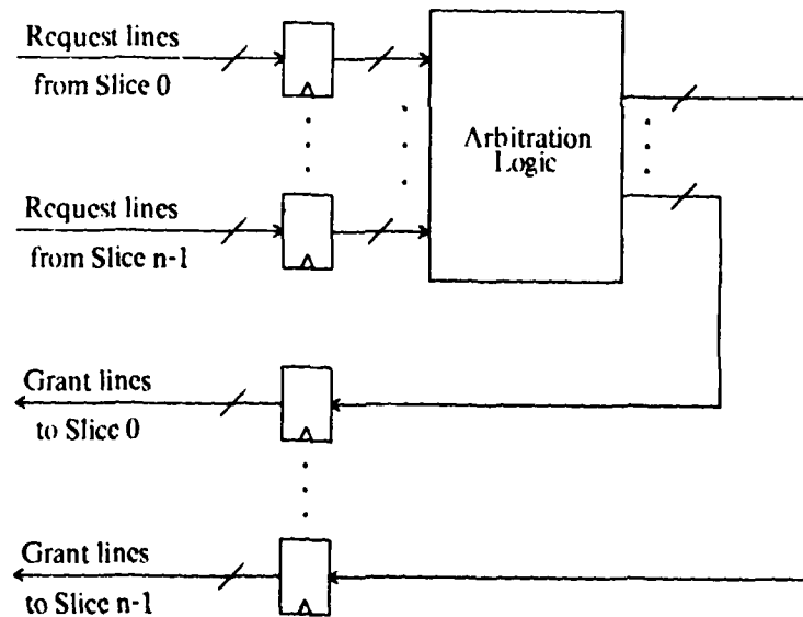
Figure 4: Combinational Model of the Arbiter
