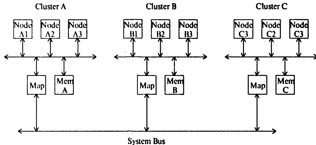
Figure 1: Hierarchical Bus Architecture
