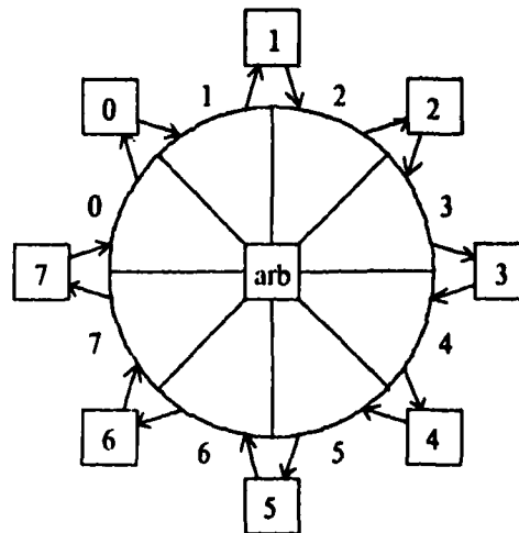
Figure 22: Concert Ring with Slice and Segment Numbers
