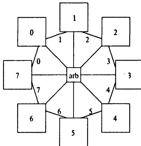
Figure 3: Ring with Slice and Segment Numbers
