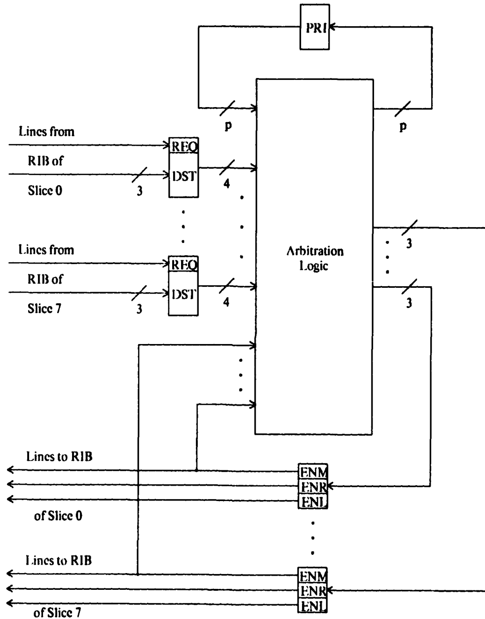
Figure 21: Top-Level View of the Concert Arbiter
