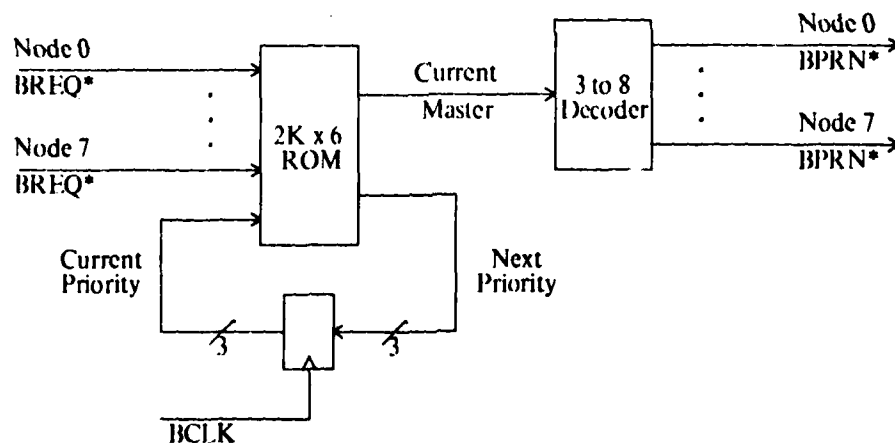
Figure 20: Multibus Parallel Arbitration Scheme
