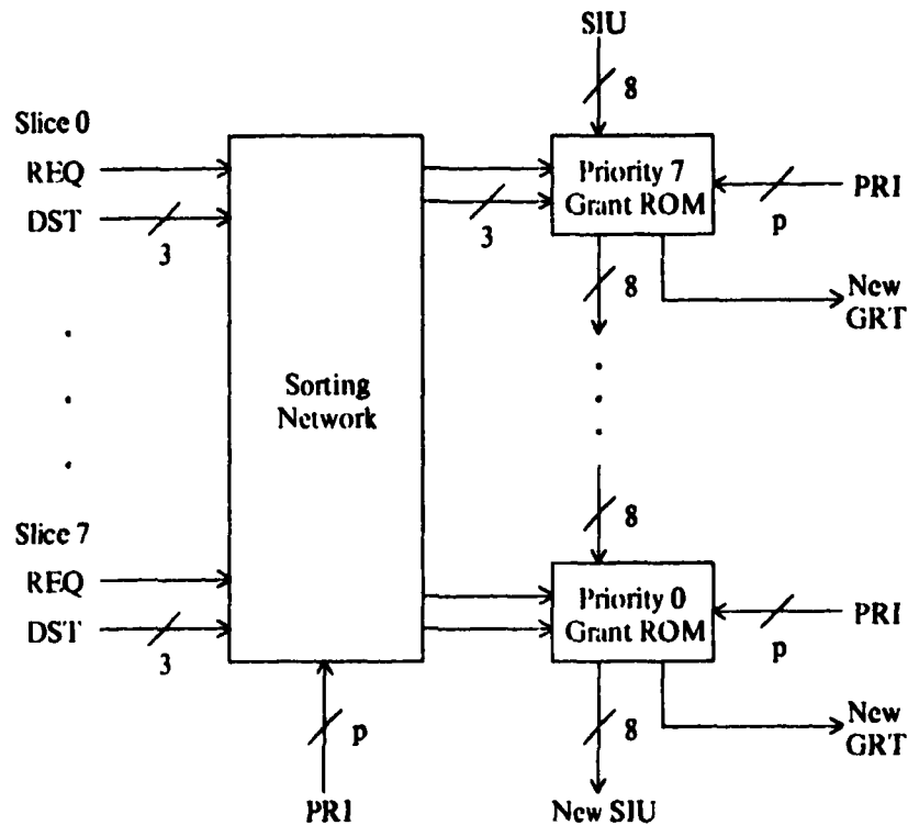
Figure 23: Chain Arbiter Implementation
