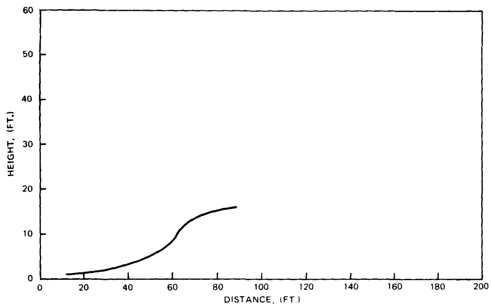
FIGURE 41. Scarp Profile No. 1 on the Southern Segment of the Airport Lake Fault.
