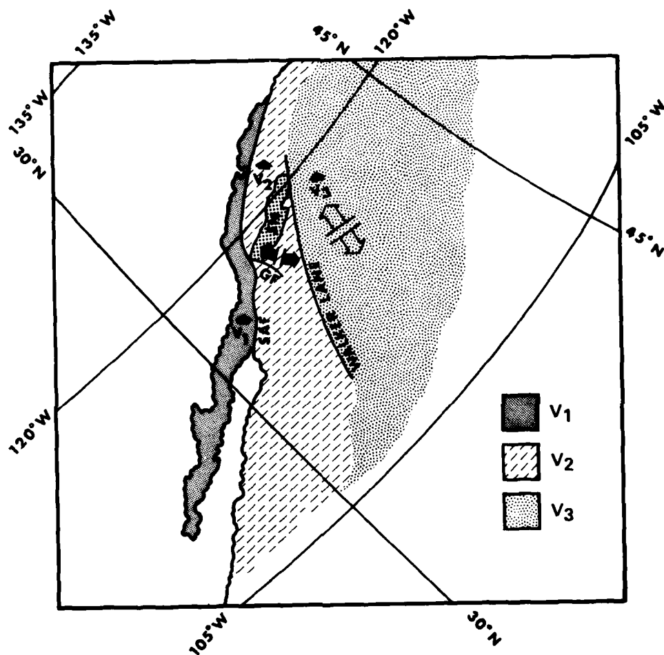
FIGURE 57. Schematic of Figure 56. (SAF) San Andreas fault, (GF) Garlock fault, (SN) Sierra Nevada. This schematic shows the northwestward migration of three sections of crust. The slowest movement is seen as V_3 . The intermediate northwest migration velocity is V_2 . The highest northwest migration velocity, V_1 , corresponds with movement on the San Andreas fault.
