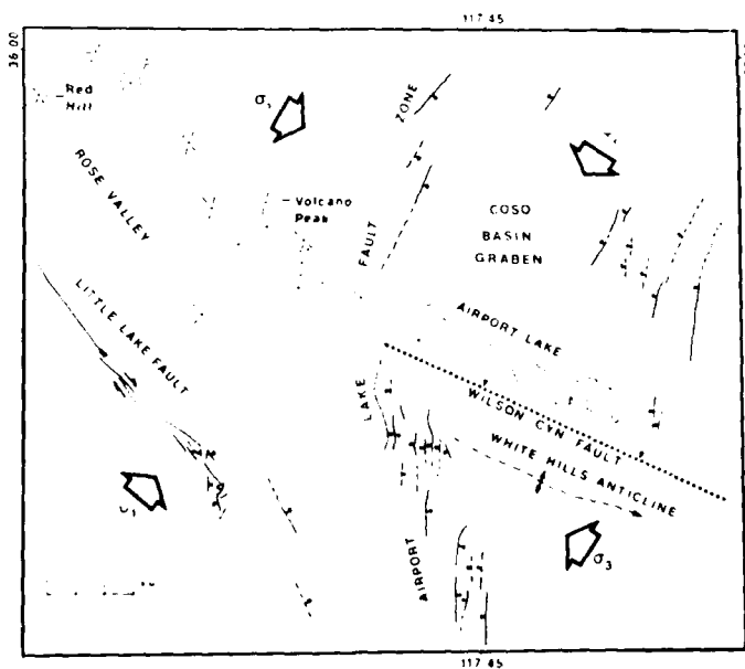
FIGURE 53. Schematic Diagram of the Southern Coso Range Showing the Local Stress Orientation. \sigma_3 is the direction of least compressive stress, and \sigma_1 is the direction of maximum compressive stress. The star symbols are cinder cones. The cones enclosed by a dashed line are the same age and composition.
