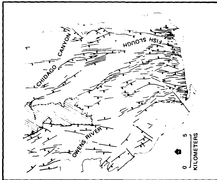
(b) Bishop Tuff.
