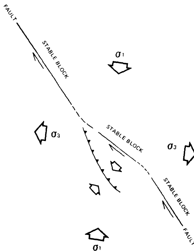
FIGURE 9. Schematic Model Indicating How Thrust Faulting Has Occurred on the Little Lake Fault.
