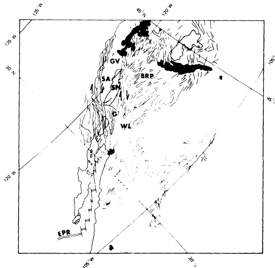
FIGURE 56. Fault Map of the Western United States and Mexico. (EPR) East Pacific rise, (WL) Walker Lane, (G) Garlock fault, (SN) Sierra Nevada, (SA) San Andreas fault, (BRP) Basin and Range province, (GV) Great Valley. Block areas are Quaternary volcanic rocks. Stippled areas are granitic plutonic rocks. (Modified from Atwater, 1970.)
