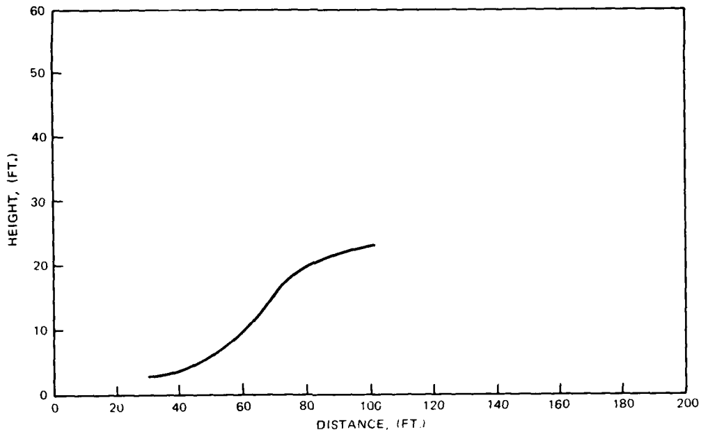
FIGURE 40. Scarp Profile No. 5 on the Coso Hot Springs Segment of the Airport Lake Fault.
