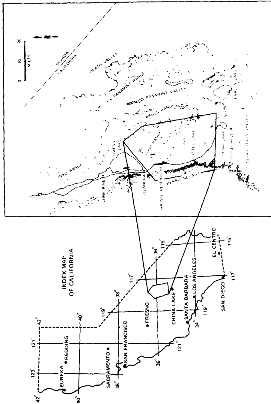
FIGURE 1. Index Map of the Study Area.
