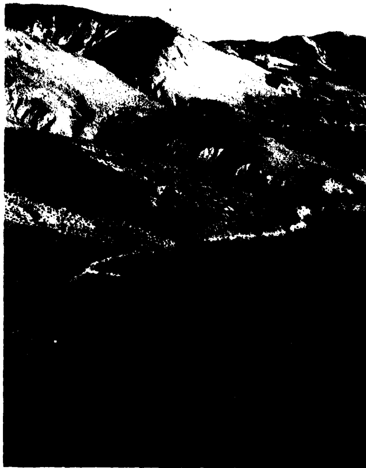
FIGURE 23. Aerial View Showing Location of Trench A.
