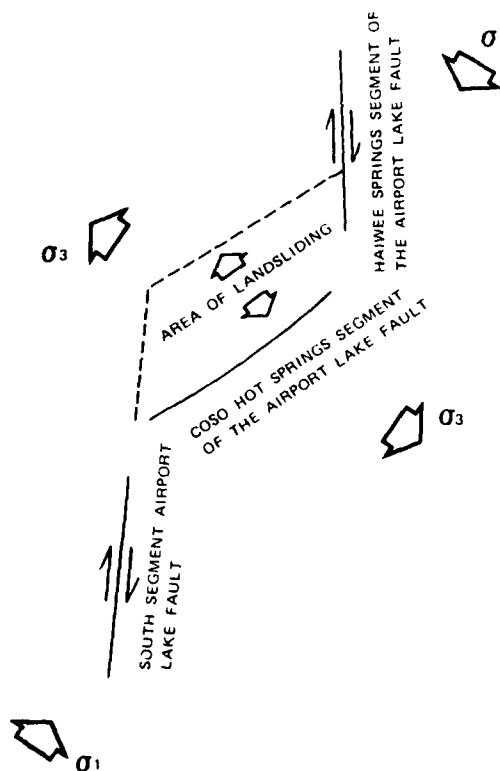
FIGURE 18. Schematic Diagram Indicating How Landslides Can Form Between en echelon Faults.
