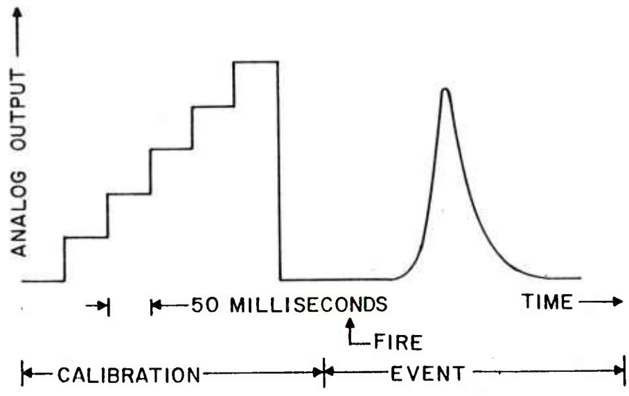
Figure 2. Data Format
