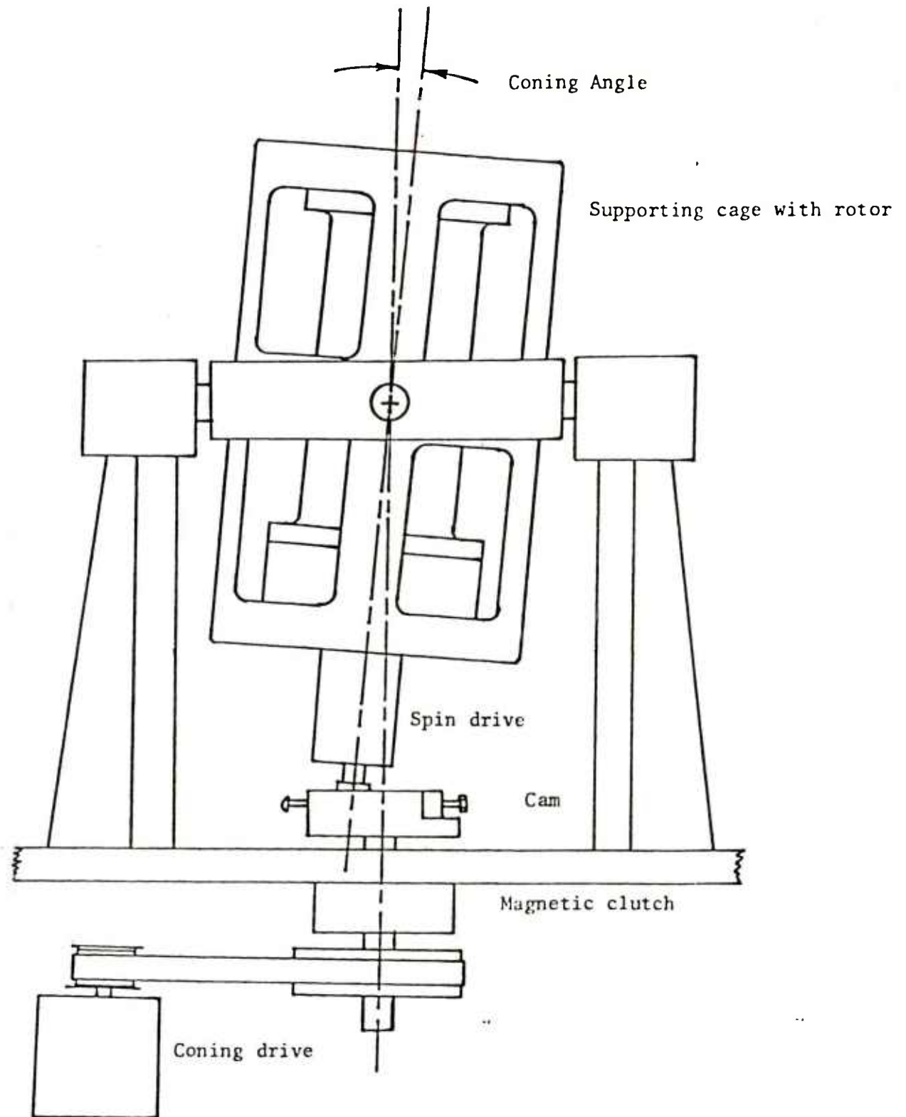
Figure 1. Gimbal Case
