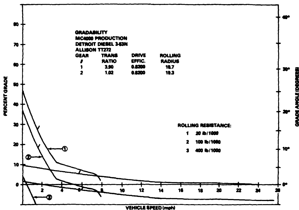
Figure 4. MC4000/M198 Gradability
