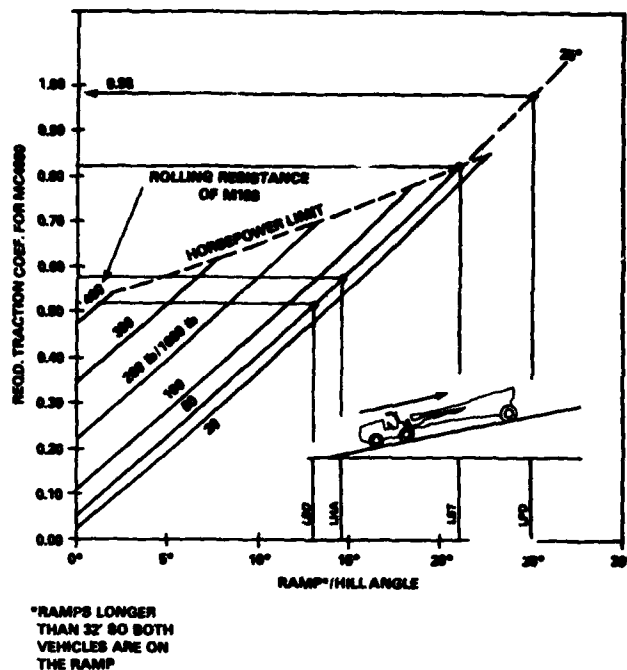
Figure 5. Traction Required for MC4000 to Push M198 (Stowed) Up Grades
