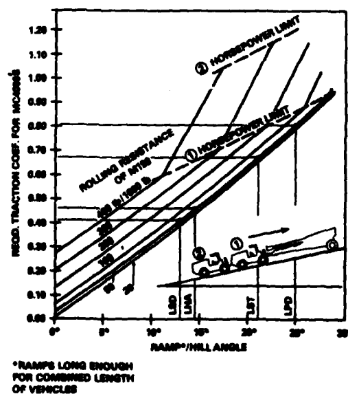
Figure 6. Traction Required for Two MC4000s to Push M198 (Stowed) Up Grades
