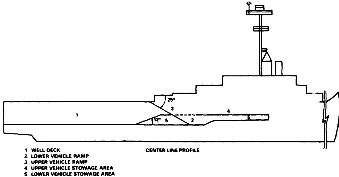
Figure 39. Profile of Amphibious Transport Dock (LPD)
