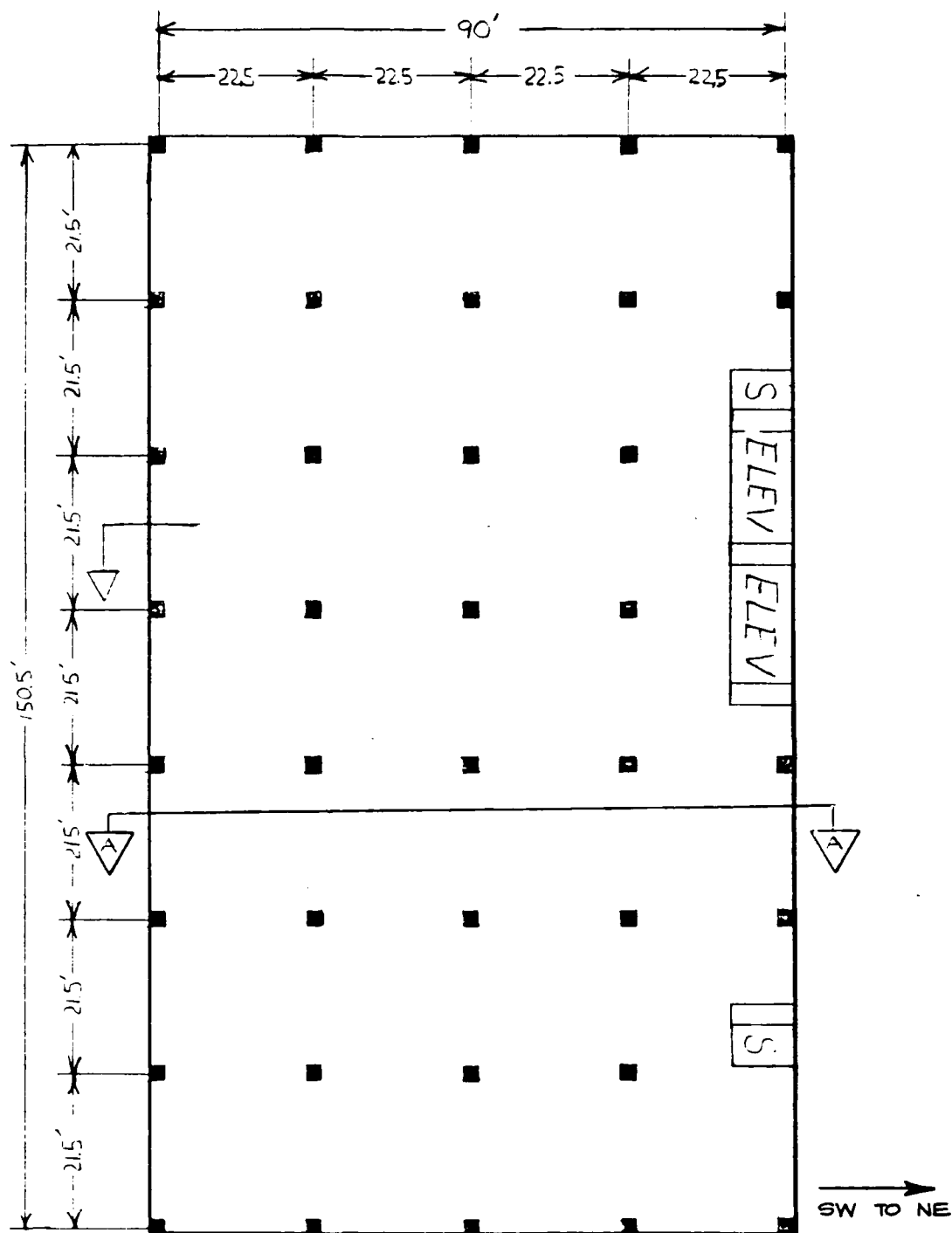
Fig. 5-3. Typical Floor Plan View.
