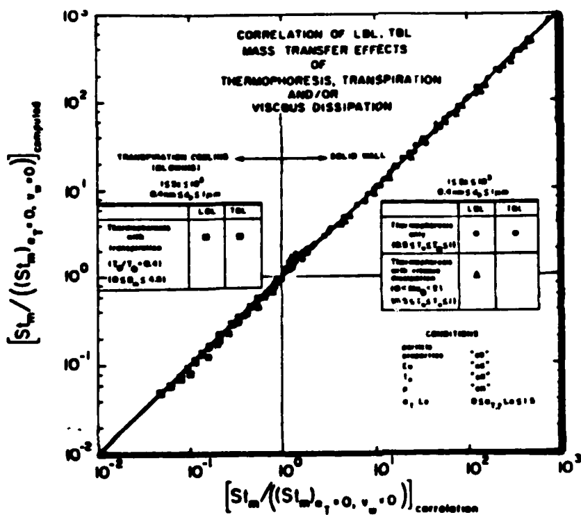
FIG. 1 Test of Thermophoretic "Section" - Thermophoretic "Sink" Correlation Scheme (Section 4) Against Exact Solutions to the Particle Mass Conservation Equation for Self-Similar Laminar Boundary Layers (after Gökçöglu and Rosner (1982)), and Law-of-the-Wall Fully Developed Turbulent Boundary Layers.
