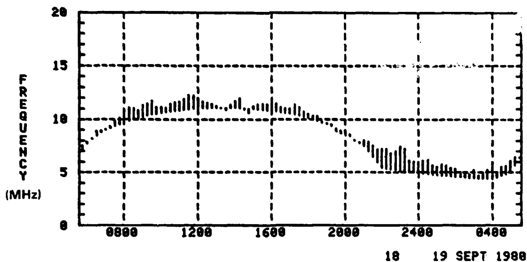
Fig. 11 — Difference between updated model and actual MUF (no nose extension)
