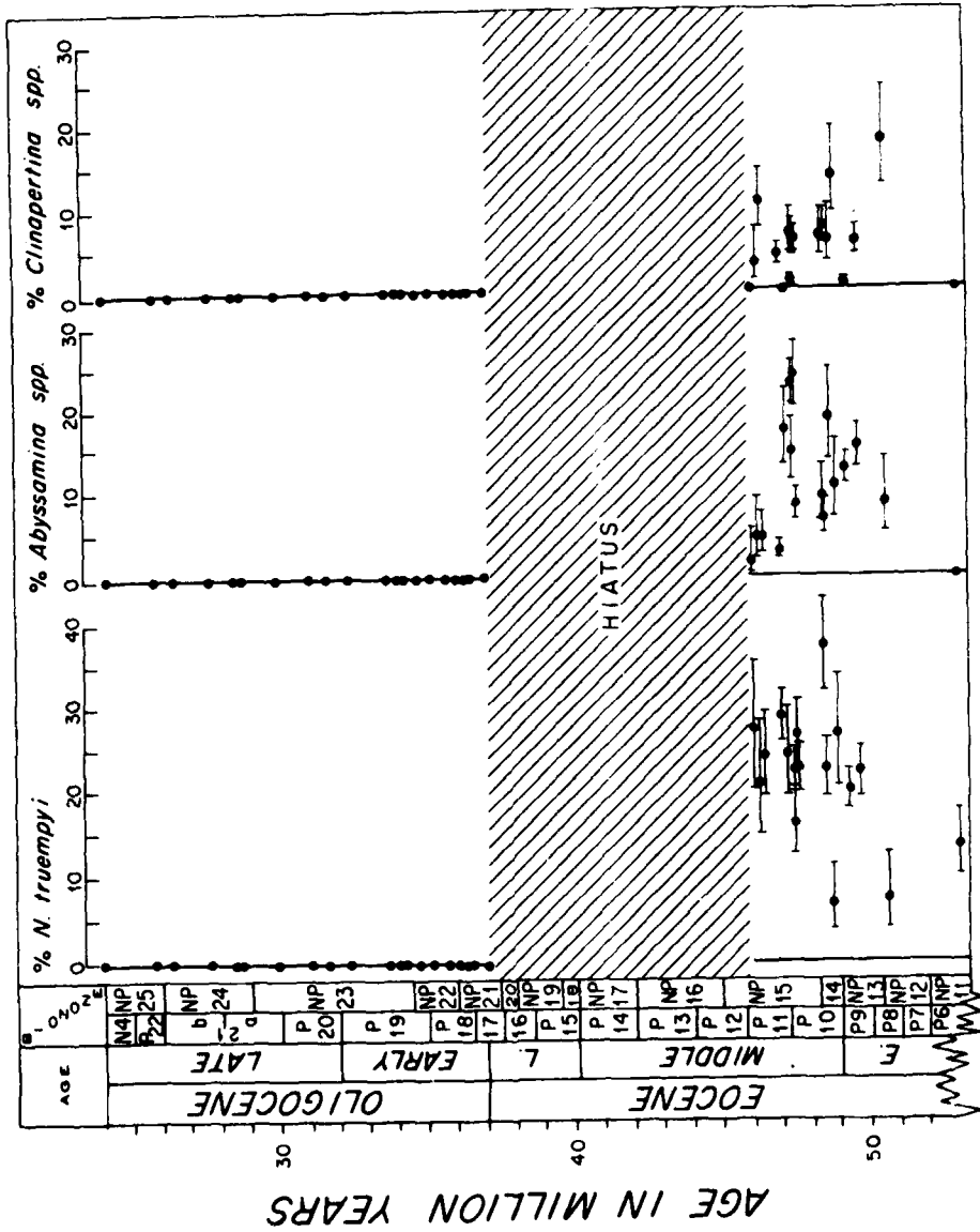
Figure 18. Distribution of dominant Eocene abyssal taxa, Site 119. 80°/o confidence interval is indicated. After Miller (in press).
