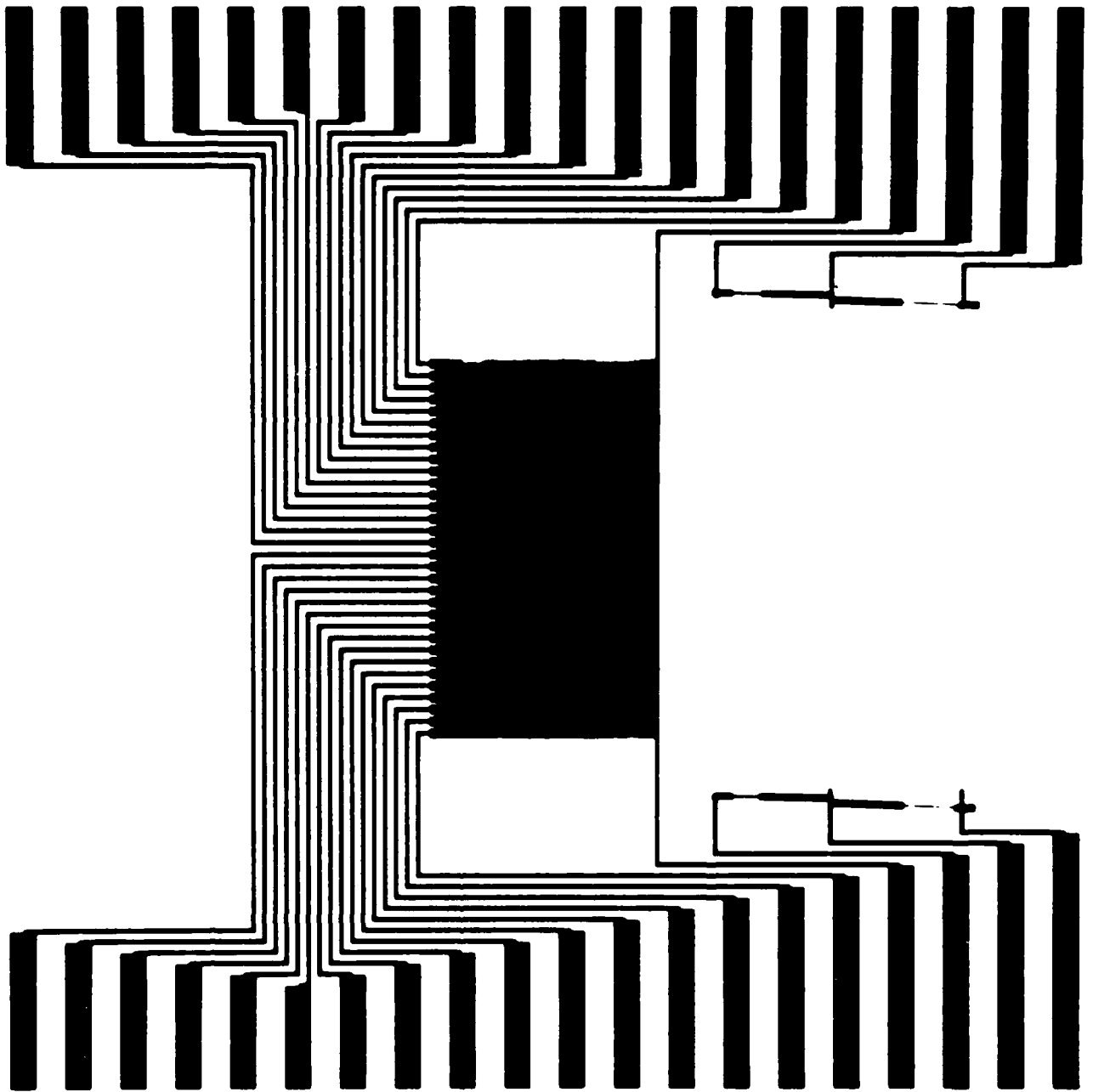
Figure 5-5. Metallization pattern mask.
