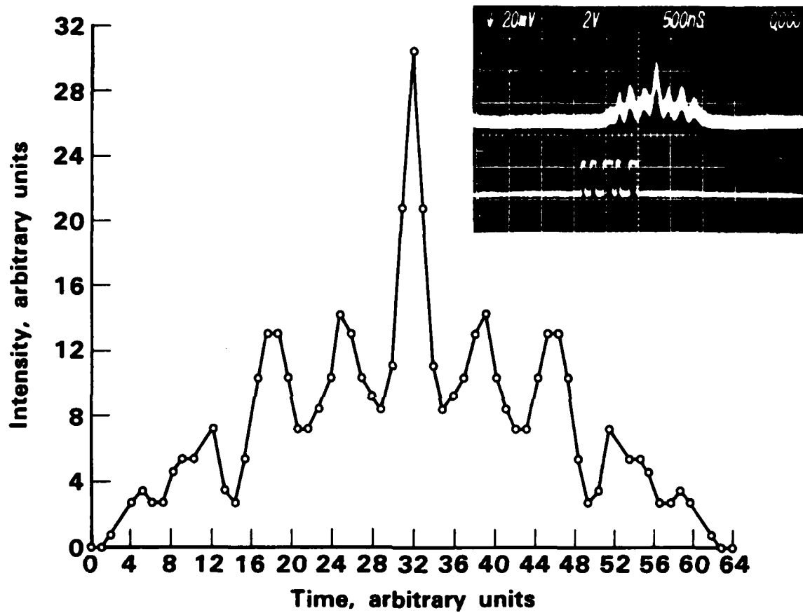
Figure 5-10. Correlation Function
