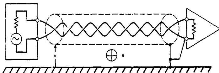
(b) GROUND LOOP OPENED
