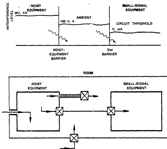
FIGURE 5 SECOND BARRIER TO CONFIN NOISY EQUIPMENT AND TO SHIELD SMALL-SIGNAL EQUIPMENT
