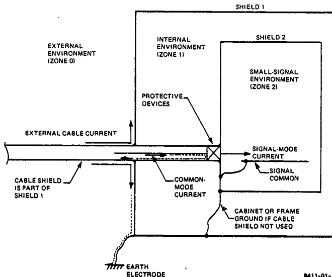
FIGURE C-7 CONCEPT OF SHIELDING FOR INTERFERENCE CONTROL
