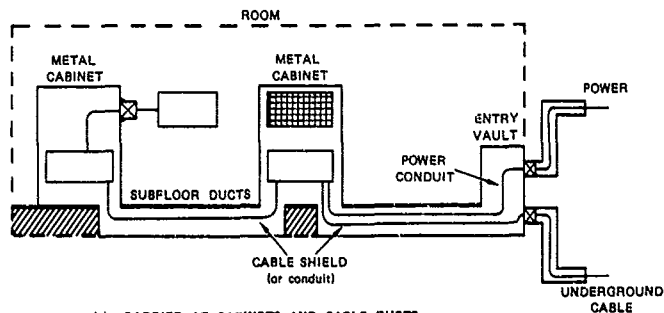
(a) BARRIER AT CABINETS AND CABLE DUCTS
