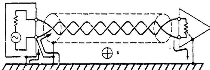
(c) ACTUAL CIRCUIT WITH GROUND LOOP OPEN
