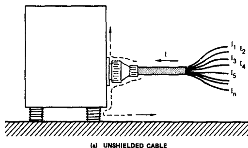
(a) UNSHIELDED CABLE
