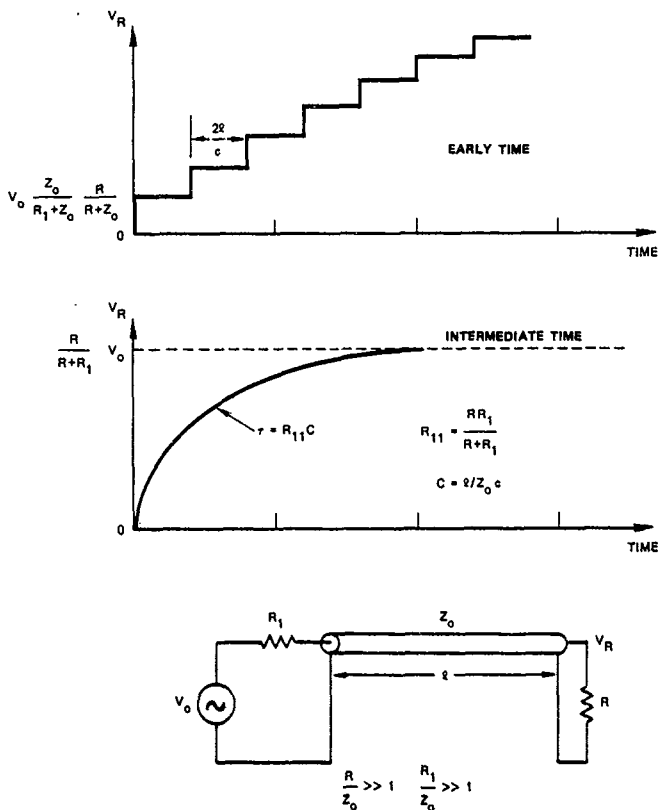
FIGURE D-2 CHARGING TRANSIENTS ON SWITCHED RESISTIVE POWER CIRCUIT
