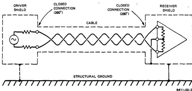
FIGURE C-11 TOPOLOGICALLY CLOSED ELECTROMAGNETIC SHIELD OVER BALANCED TWISTED SHIELDED PAIR
