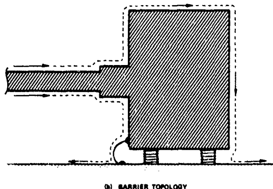
FIGURE 3 CONFIGURATION AND TOPOLOGY WITH SHIELDED INTERCONNECTING CABLE
