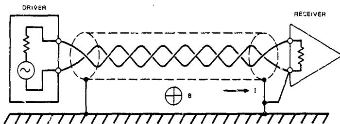
(a) "GROUND LOOP"
