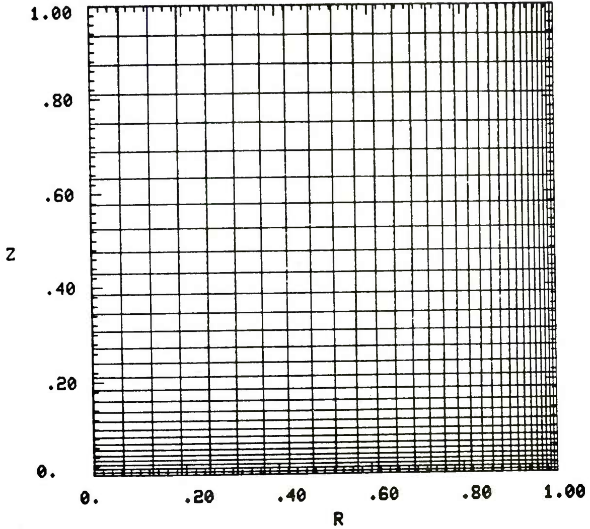
Fig. 2. Computational Grid for Reynolds number of 10,000.
