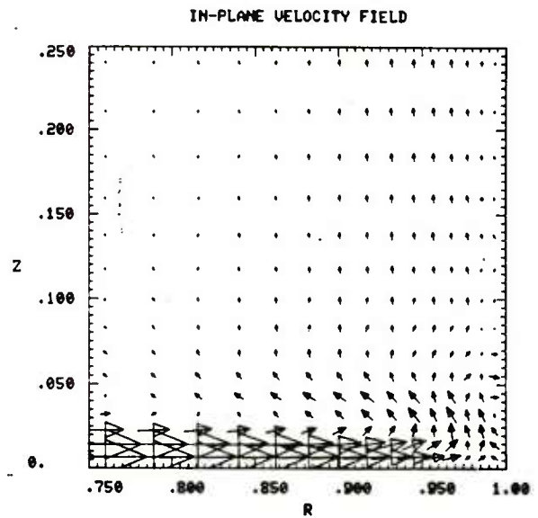
Fig. 3d. Time = 62.5
