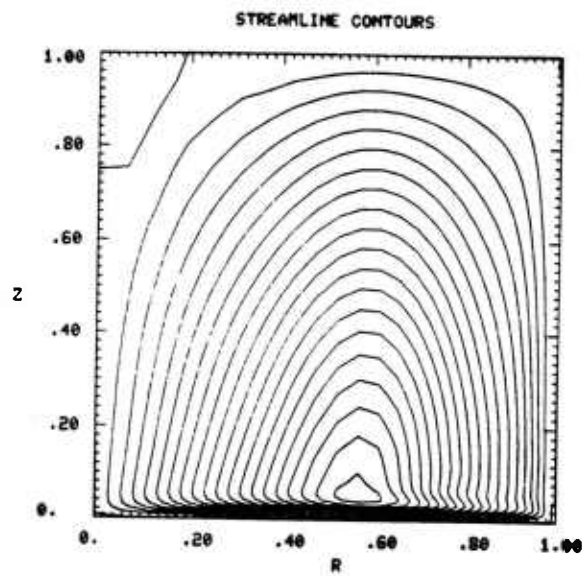
Fig. 5c. Time = 93.75
