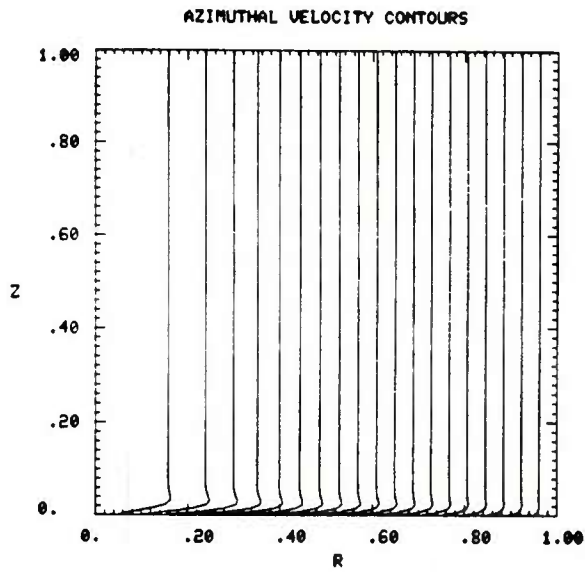
Fig. 4e. Time = 218.75
