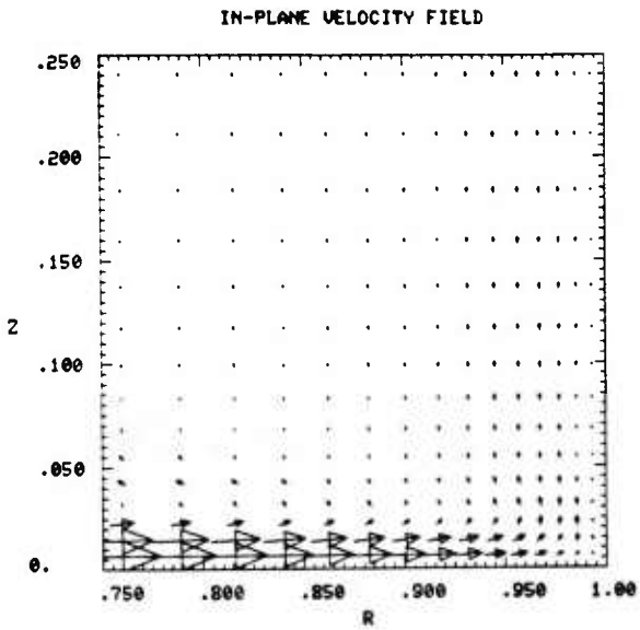
Fig. 3e. Time = 93.75
