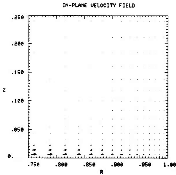
Fig. 3g. Time = 218.75
