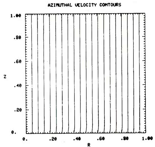
Fig. 8b. Time = 125.0
