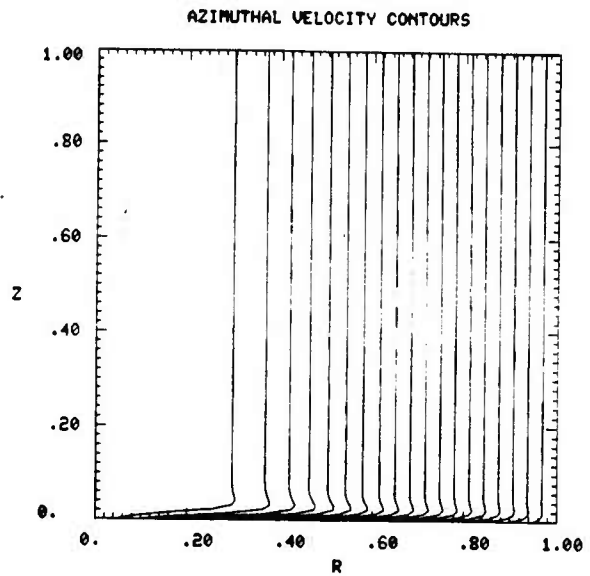
Fig. 4d. Time = 156.25
