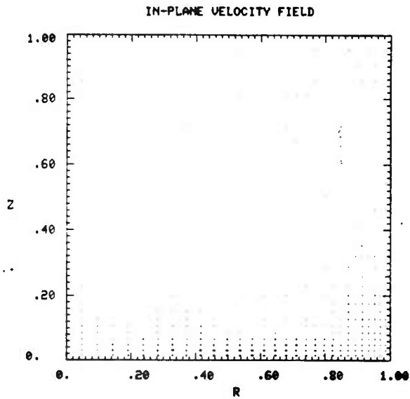
Fig. 7c. Time = 125
