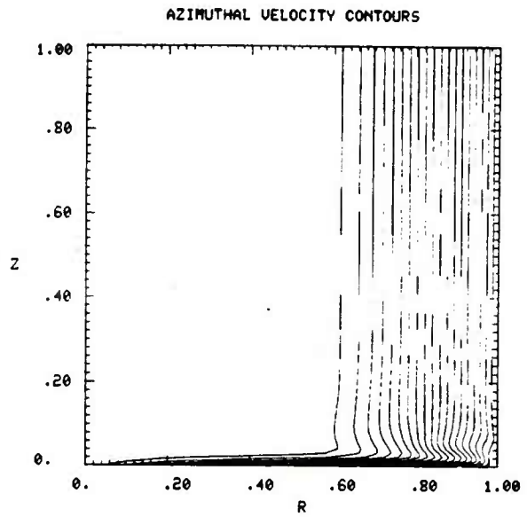
Fig. 4b. Time = 62.5
