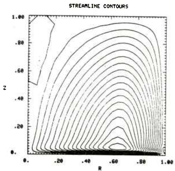
Fig. 5b. Time = 62.5
