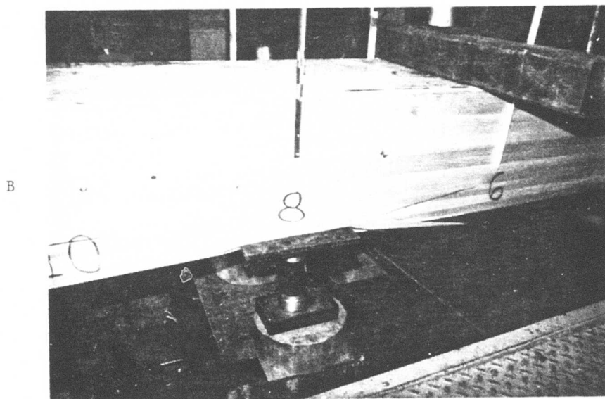
Fig. 3-40. Pre- and Post-Test Photographs of Test Specimen.
