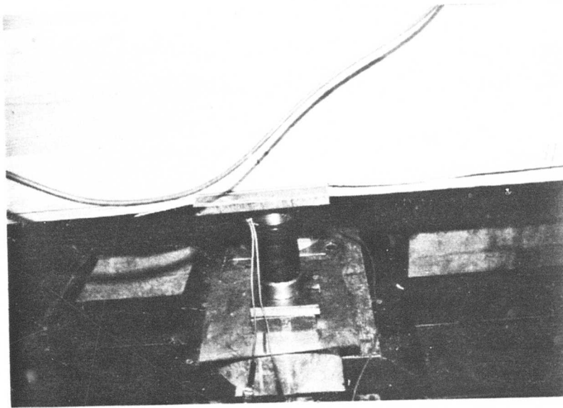
Fig. 3-34. Closeups of Bearing-Flexural Failure at the Midspan Shore on the Failed Glulam Beam.
