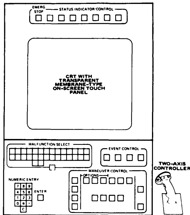
FIGURE 2. INTERACTIVE CONTROL/DISPLAY MODULE
