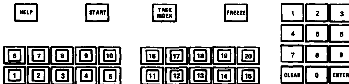
Figure 3. Instructor Input Device
