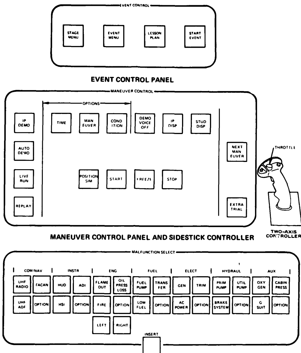
REPRESENTATIVE MALFUNCTION CONTROL PANEL
