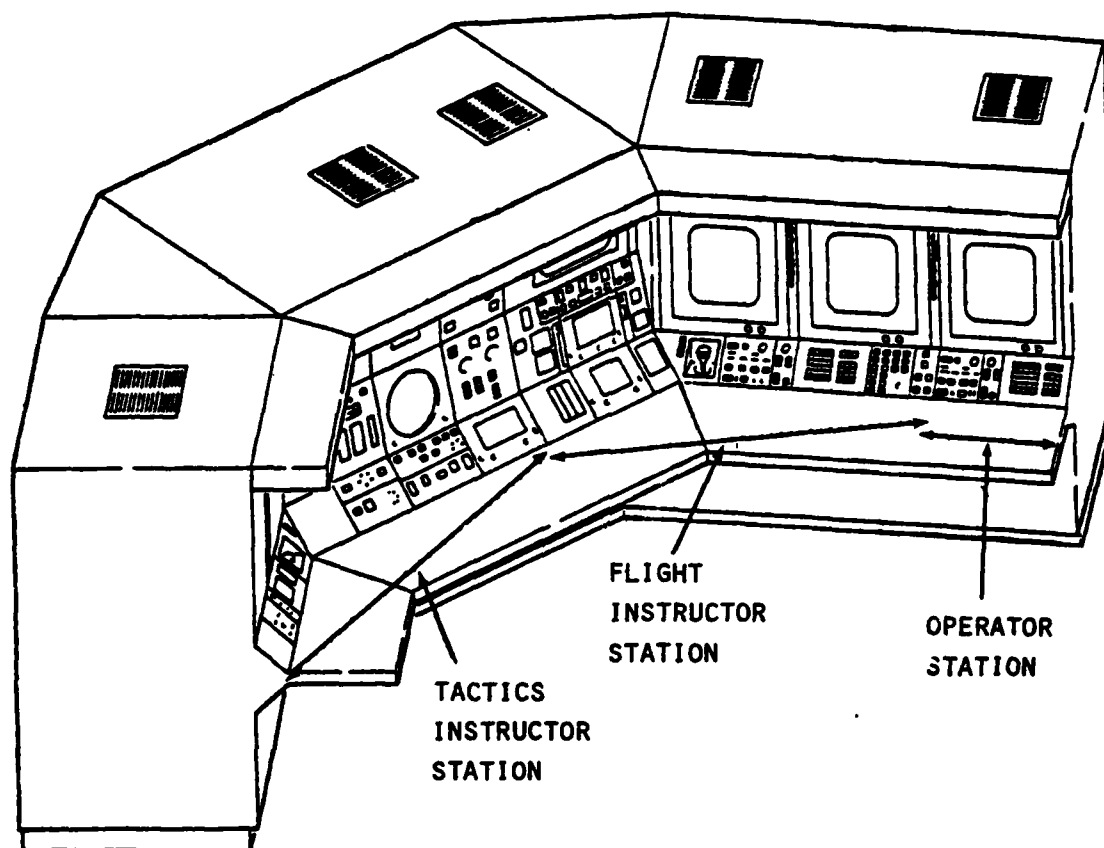
Figure 2. Device 2F112 IOS Arrangement
