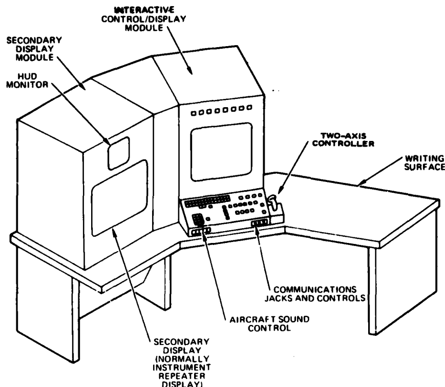
FIGURE 1. GENERAL CONFIGURATION OF VTXTS SIMUL FOR INSTRUCTOR CONSOLE (USED ON IFT, OFT, ACMT)
