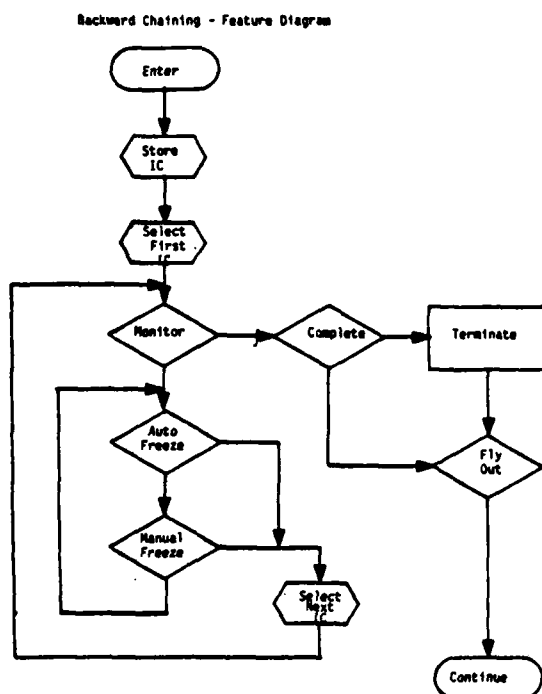
Figure 3 Example of a Feature Diagram
