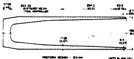
Fig. 11 Preform design of 155-mm shell
