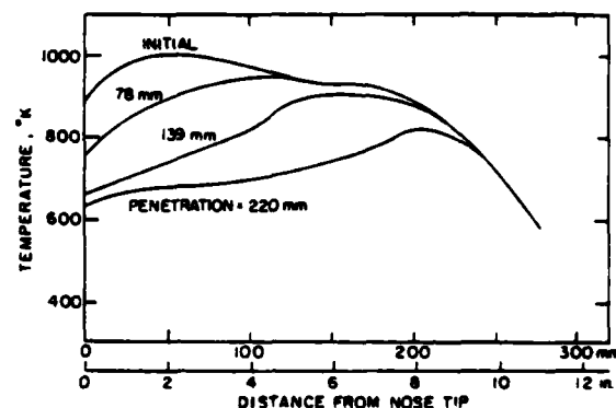
Fig. 15 Outer surface temperature distributions at different die penetrations
