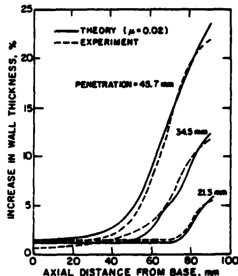
Fig. 16 Development of increase in wall thickness
