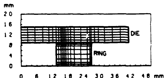
FIG. 9. Initial mesh for Al 1100 ring compression.
