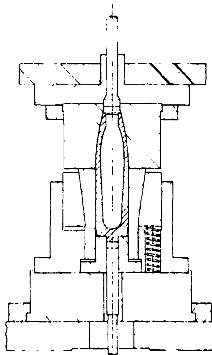
Fig. 1 Shell nosing process (from reference [6])
