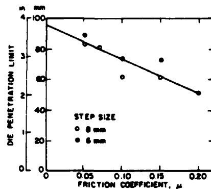
Fig. 12 The effect of friction coefficient on the die penetration limit in nosing
