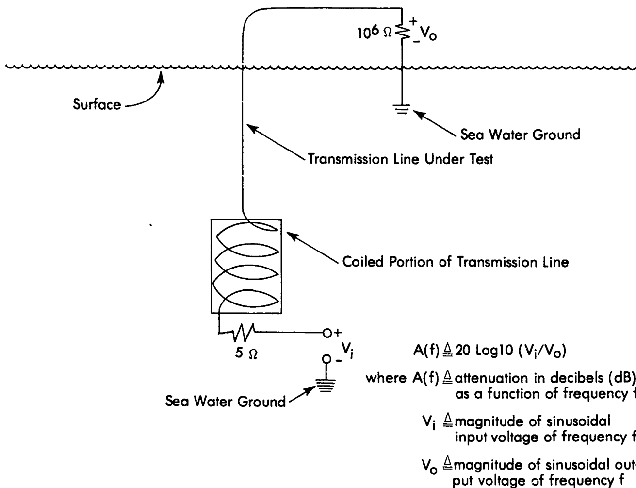
Figure 3. Defining attenuation
