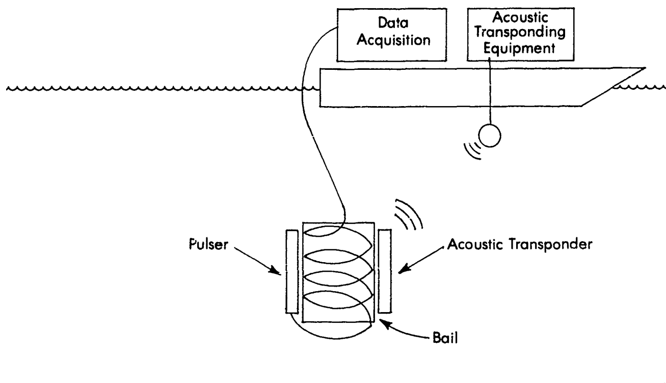
Figure 2. Test setup
