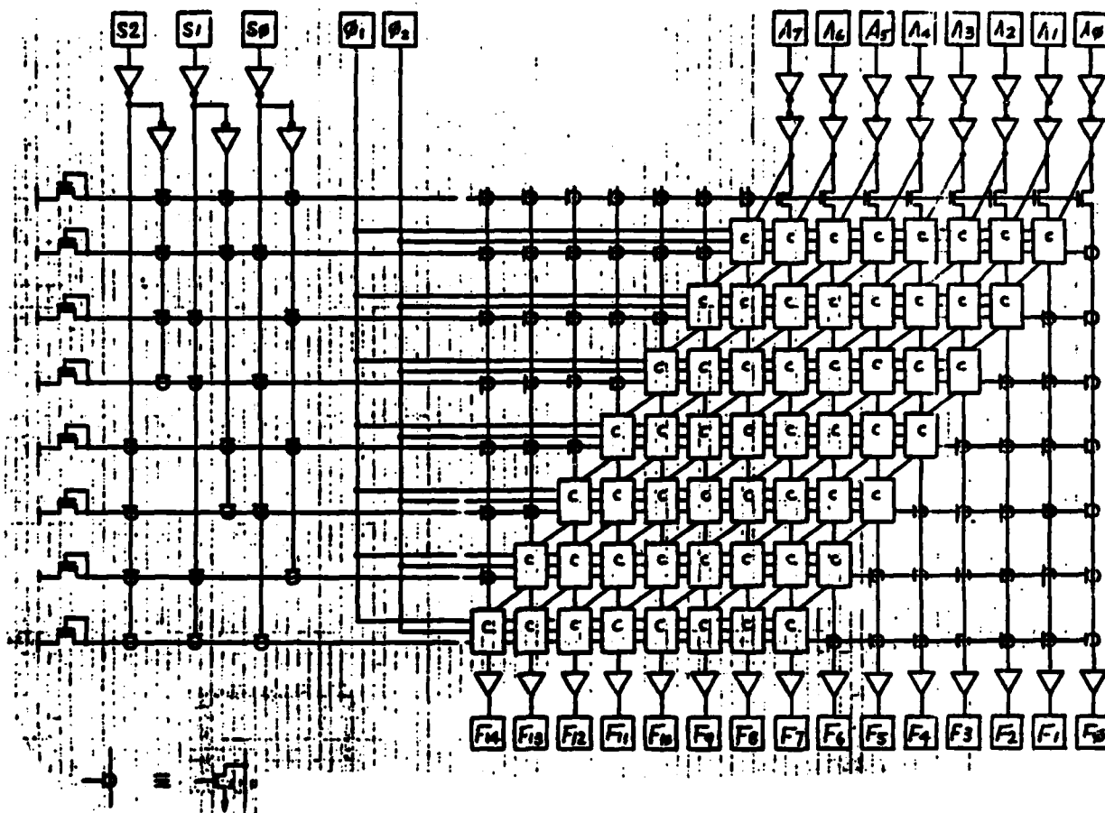
Figure 36: Schematic of Barrel Shifter
