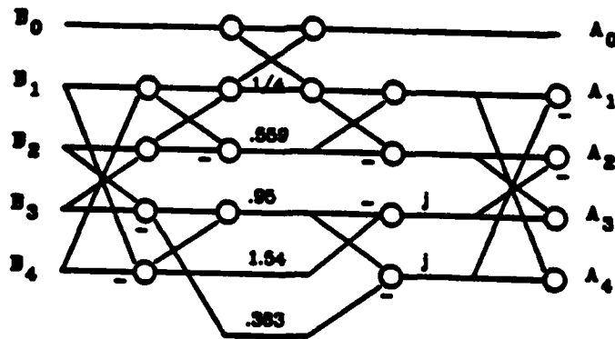
Figure 14: Base 5 Signal Flow Graph
