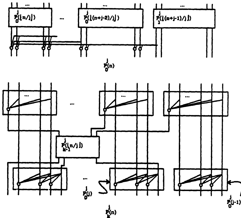
Figure 56: Recursive Construction of High Fan-in Circuits
