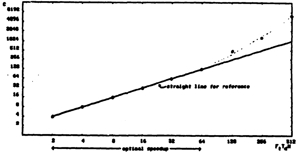
Figure 6: Cost in number of chips
