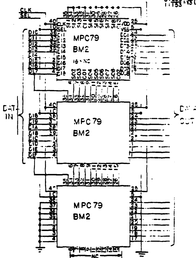
Figure 34: 16 bit Root 3 Circuit
