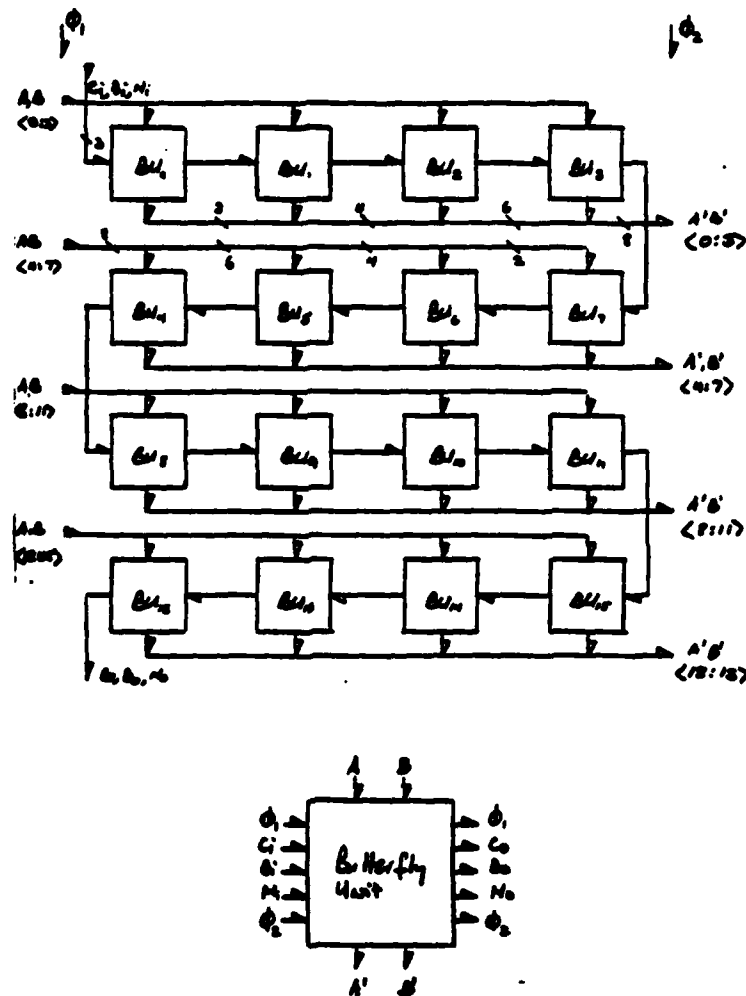
Figure 47: 16 Bit Butterfly Processor
