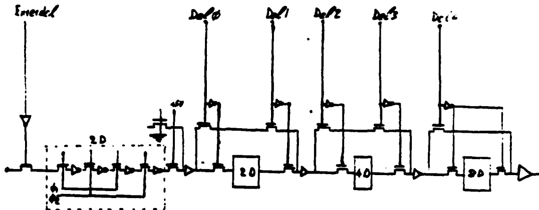
Figure 51: Programmable Delay Circuit
