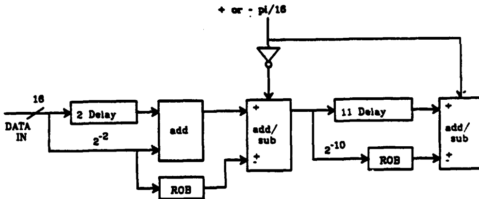
Figure 38: Block Diagram of \frac{\pi}{16} Circuit
