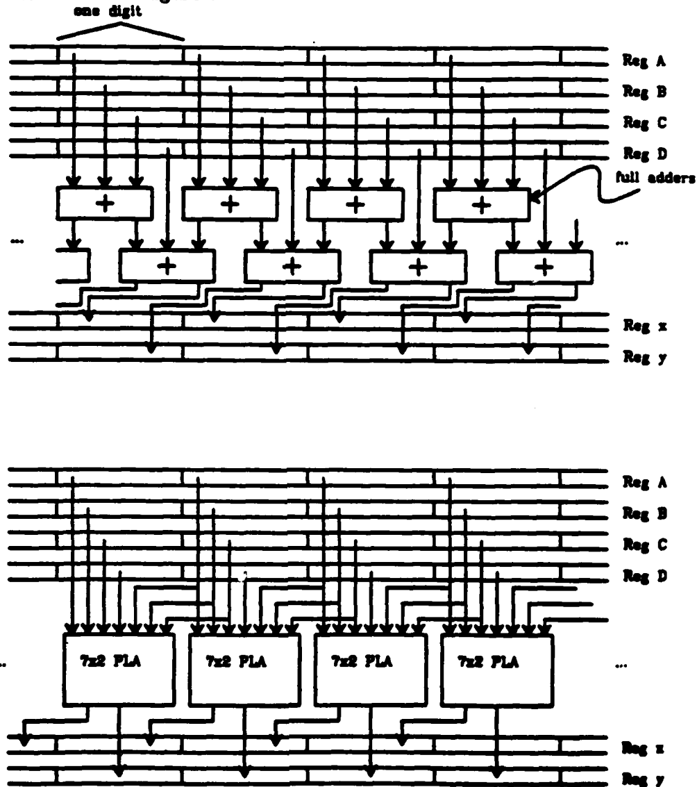
Figure 67: Four to Two Reduction Adder
