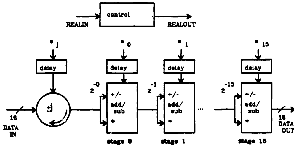
Figure 40: Block Diagram of CORDIC rotator
