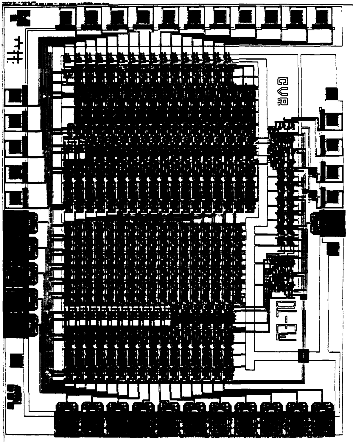
Figure 39: CIFPLOT of \frac{\pi}{18} Chip
