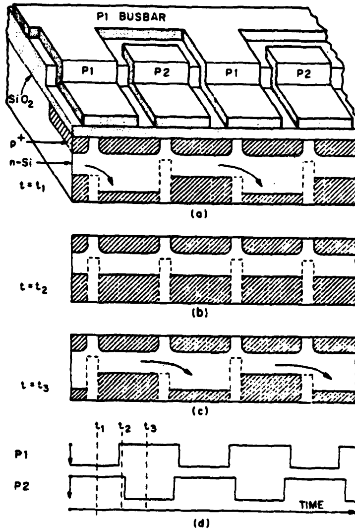
Figure 29 (a): Schematic rendering of a p-channel BBD with the associated potential diagram shown in the cross section of the silicon substrate. (b,c): Potential diagrams shown for various biasing conditions illustrating the transfer of charge. (d): The corresponding time slots marked in the diagram of the clock waveforms.
