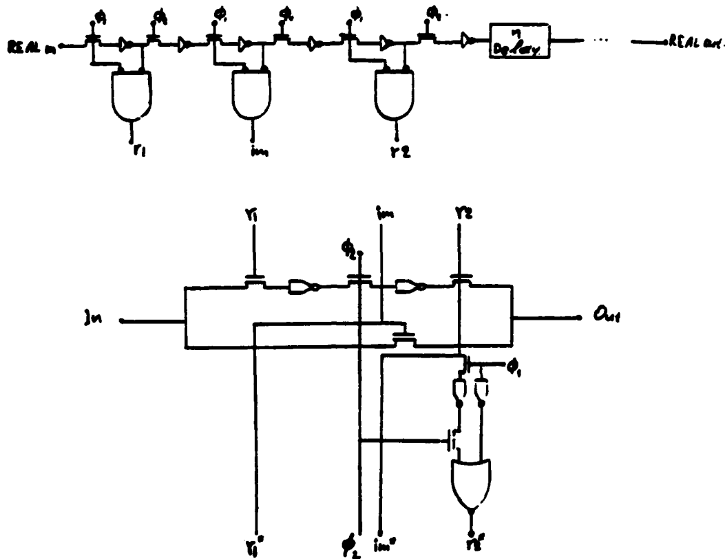
Figure 45: ROB and ROB Control Signals
