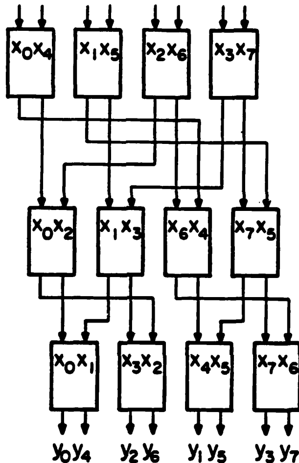
Figure 73: The FFT network for N=8 .
