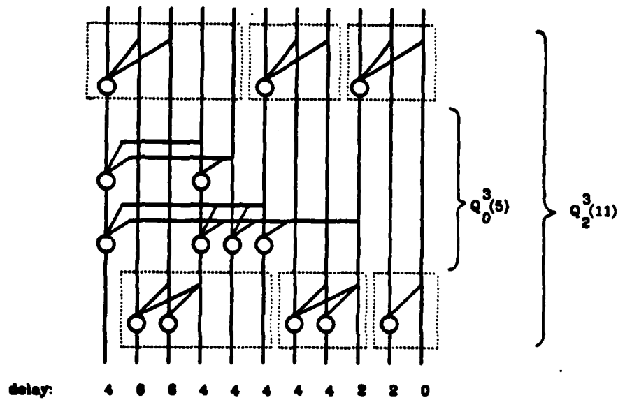
Figure 65: Example for Fan-in 3
