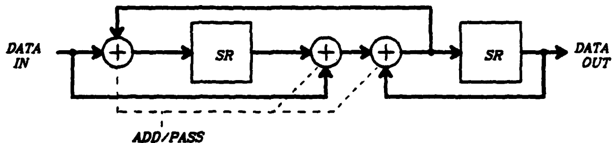
Figure 10: Last Half of Base 3 Butterfly
