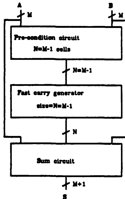
Figure 66: Fast Adder Circuit
