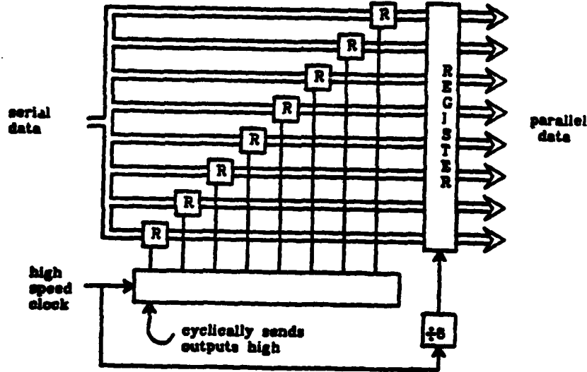
Figure 4: Decimator for Example 1
