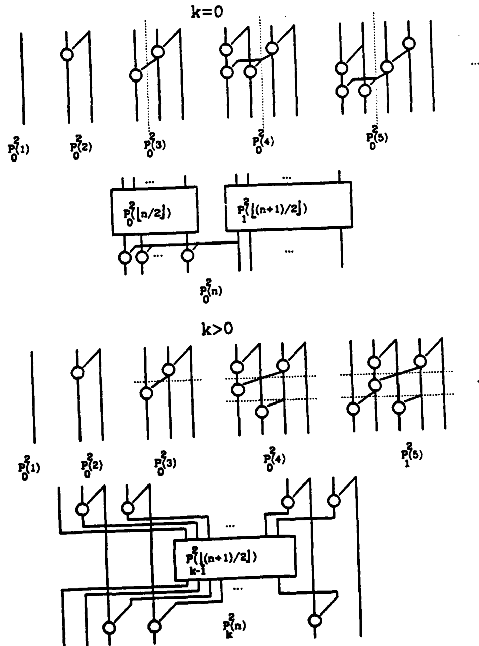
Figure 54: Definition of P_k^2(n) Circuits
