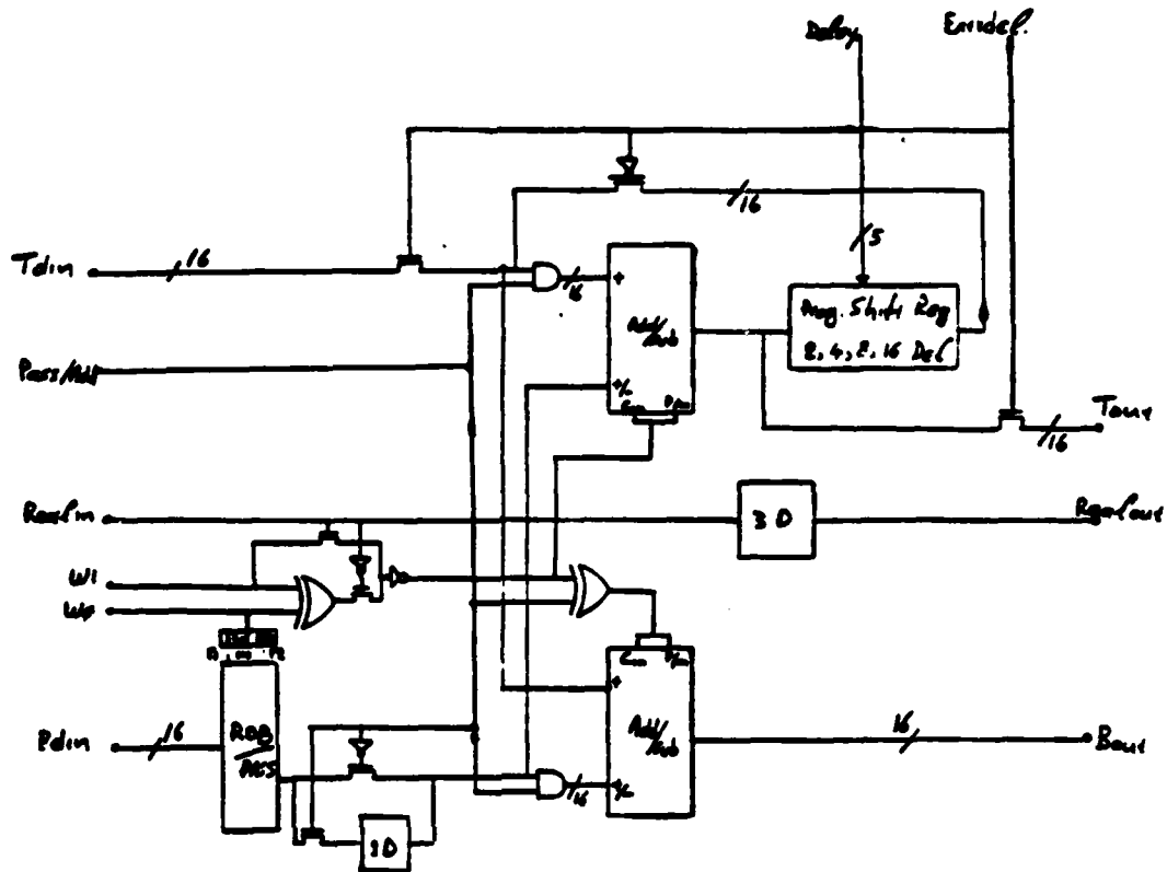
Figure 50: Schematic of Butterfly Module
