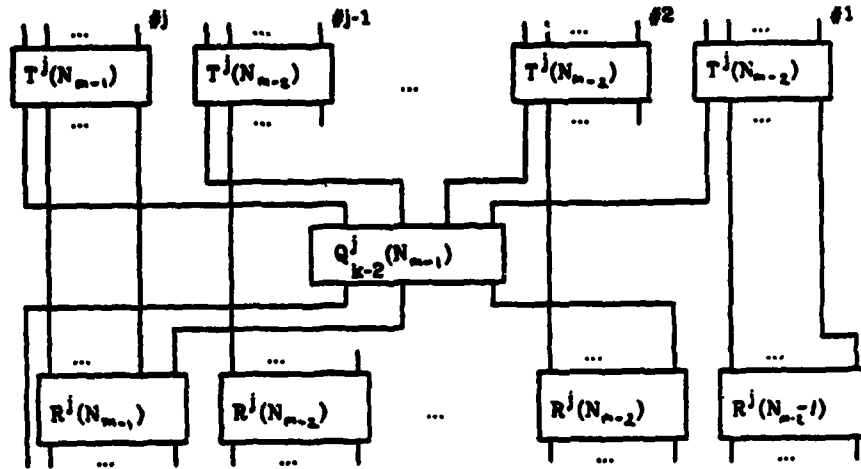
Figure 62: General Construction of Q_k^j(N_m)
