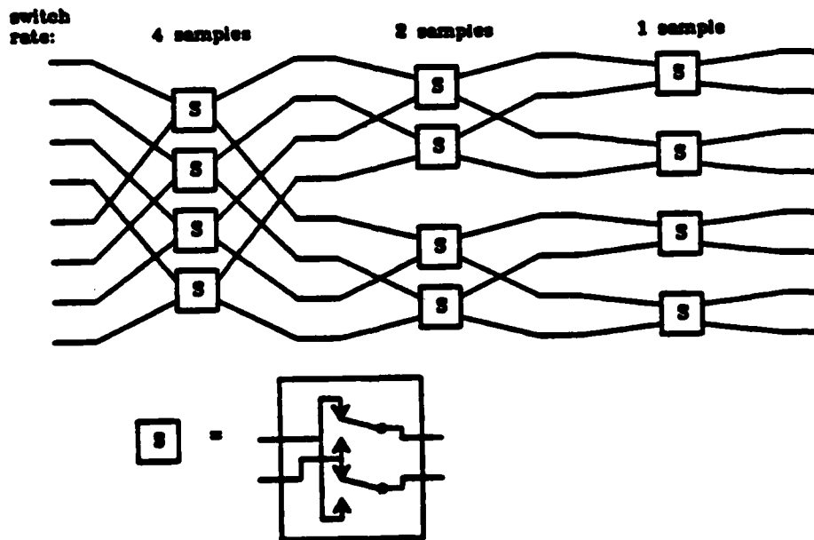
Figure 3: Commutator for Example 1
