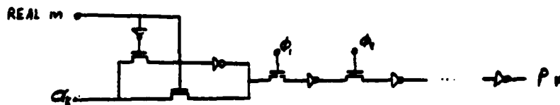
Figure 44: Inversion of a_k
