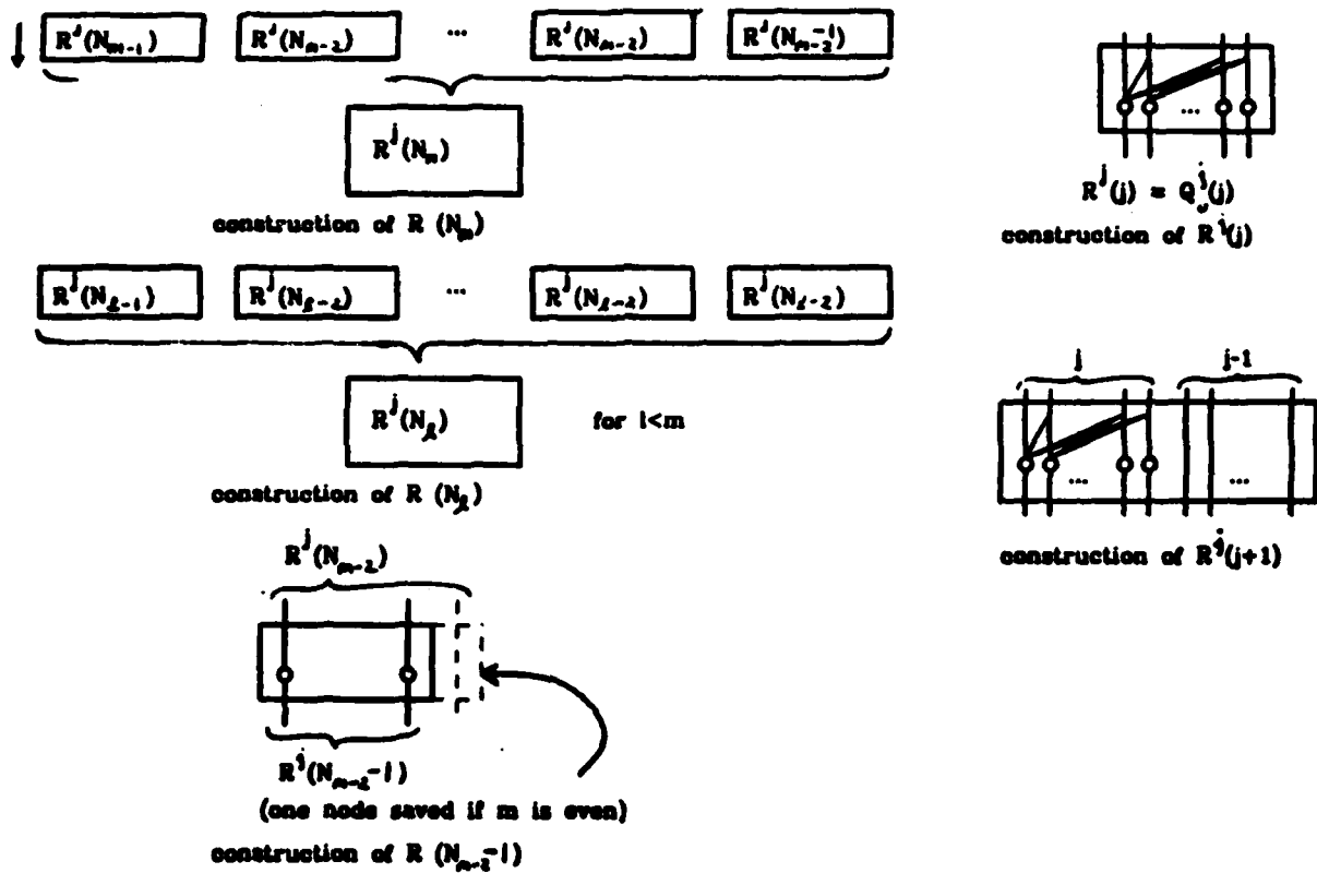
Figure 64: Construction of R circuits
