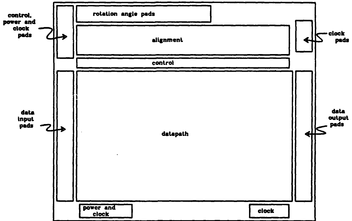
Figure 41: Floor Plan of CORDIC rotator
