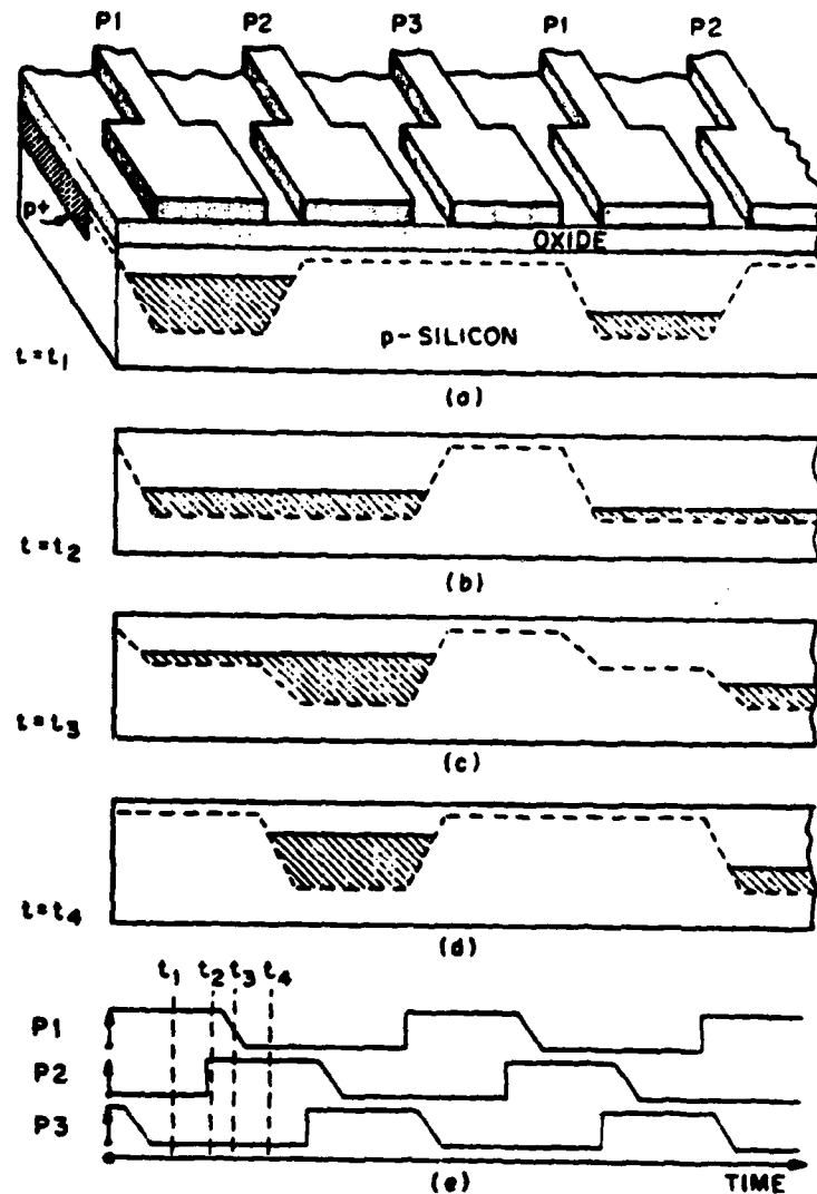
Figure 30 (a): Schematic rendering of a 3-phase n-channel CCD with the charge carrying potential wells shown in the cross section of the silicon substrate. (b,c,d): Potential wells shown at subsequent time intervals illustrating the transfer of charge. (e): The corresponding time slots marked in the diagram of the waveforms.
