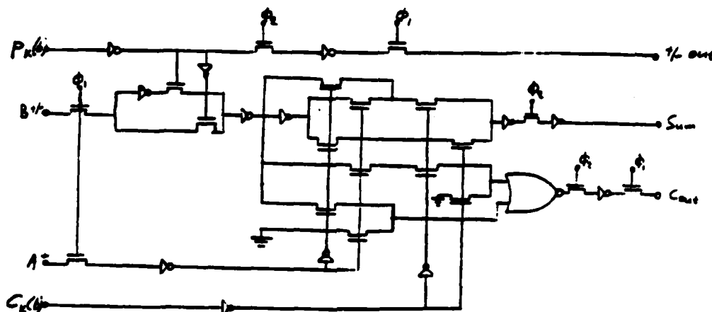
Figure 43: Adder Module
