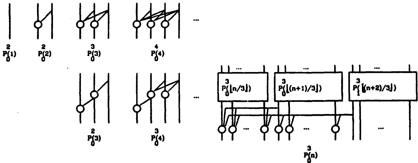
Figure 55: High Fan-in Circuits
