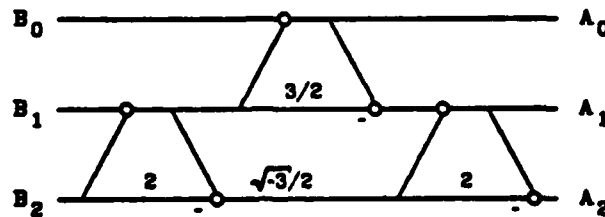
Figure 7: Signal Flow Graph of Base 3 DFT
