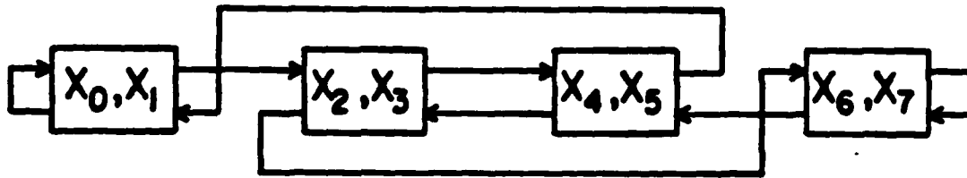
Figure 74: The perfect shuffle interconnections for N=8 .
