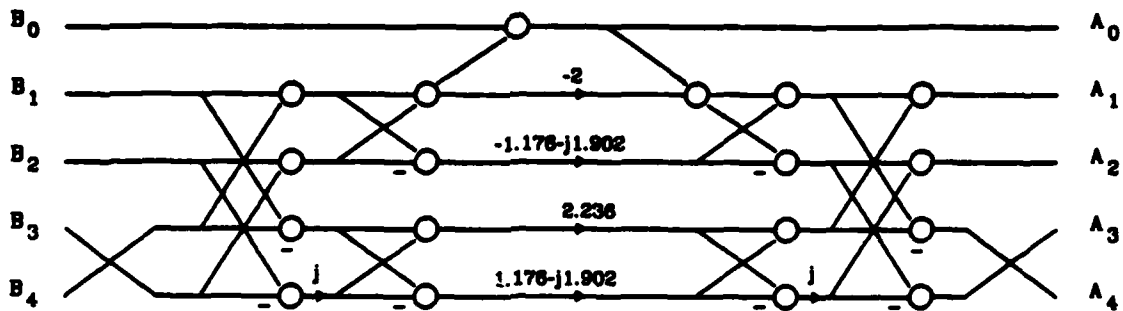
Figure 15: New Base 5 Signal Flow Graph
