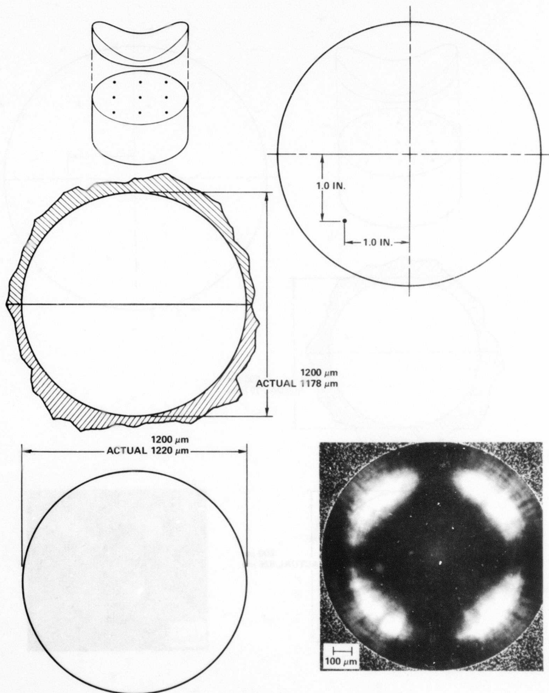
Fig. A26 Sample 90-7: 1200 μm spherical void.
